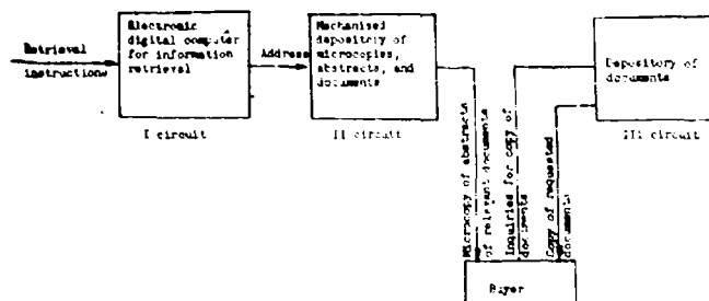
Fig. 1. Block diagram of three-circuit IPS.
