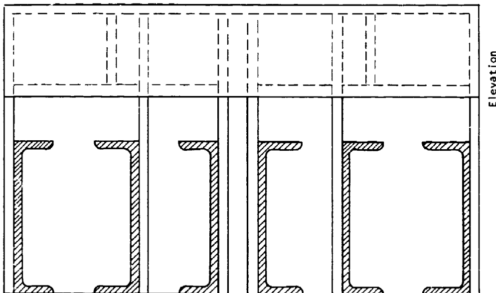
Figure 78 Plan and Elevation Views of Possible Cantilevered End Reaction
