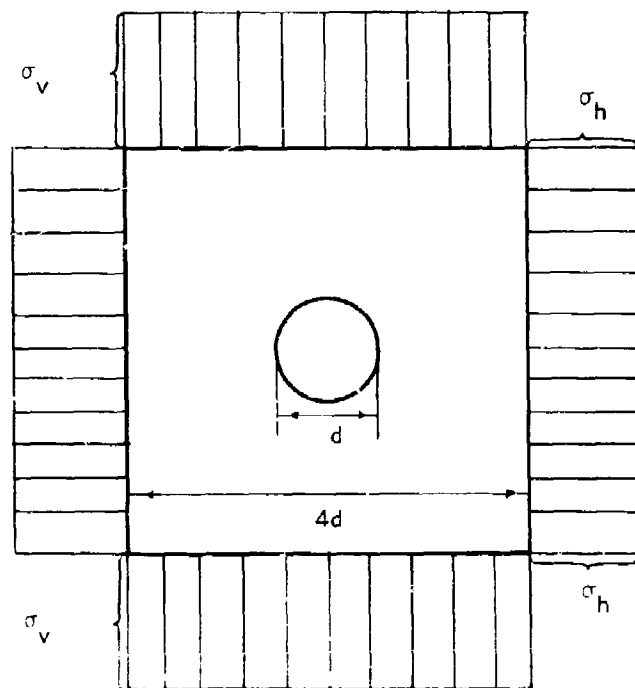
Figure 2 Approximate Stress Distribution Some Distance From Tunnel
