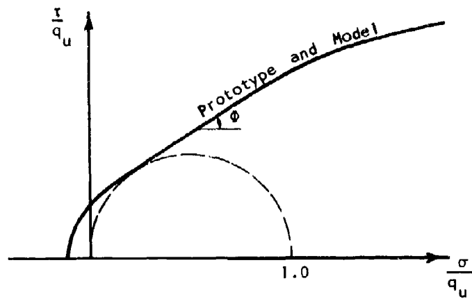
Figure 7 Dimensionless Prototype and Model Mohr Envelopes
