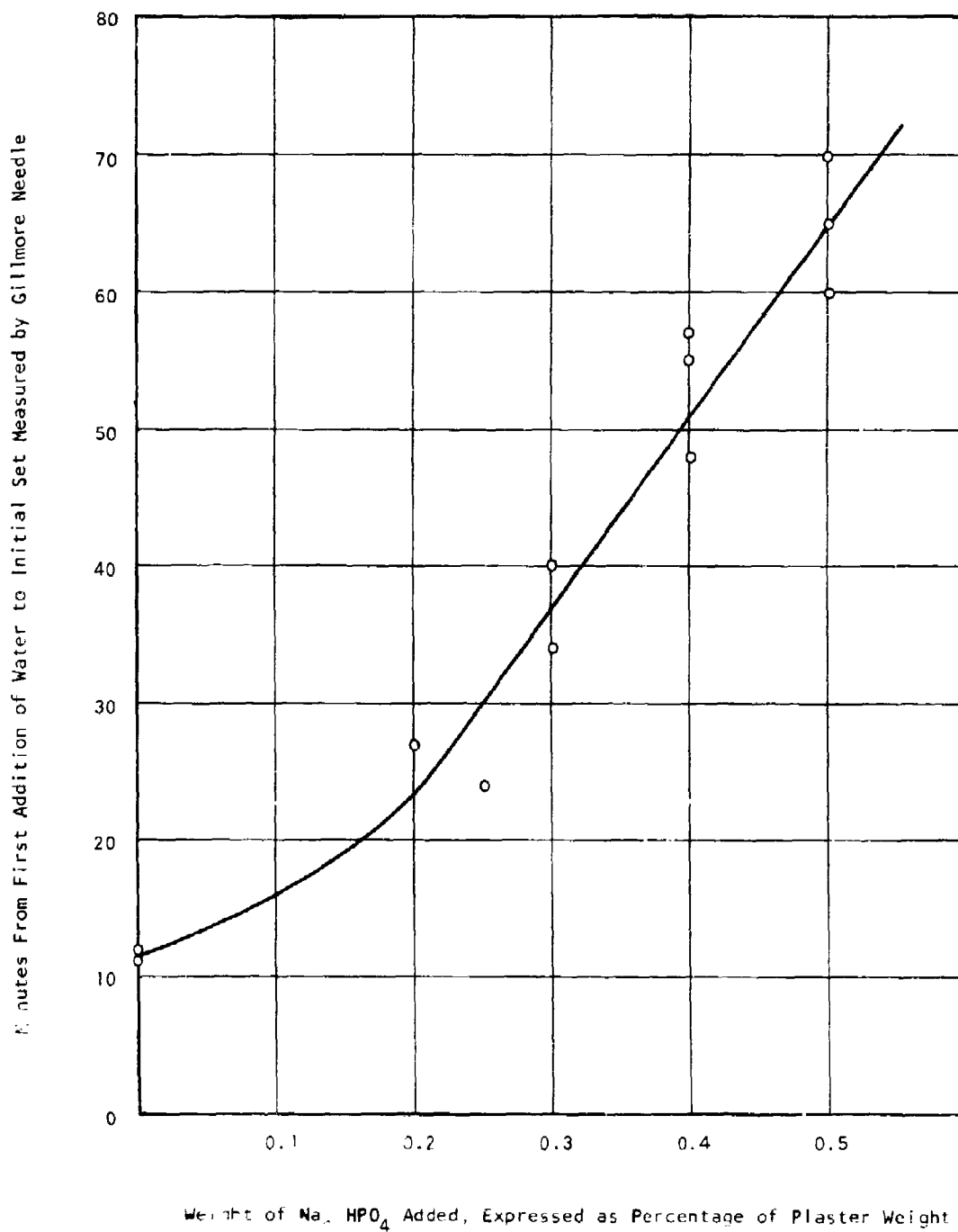
Figure 11 Retarding Effect of \text{Na}_2\text{HPO}_4 on Water/Plaster/ Kaolinite Mixtures of 2/1/2
