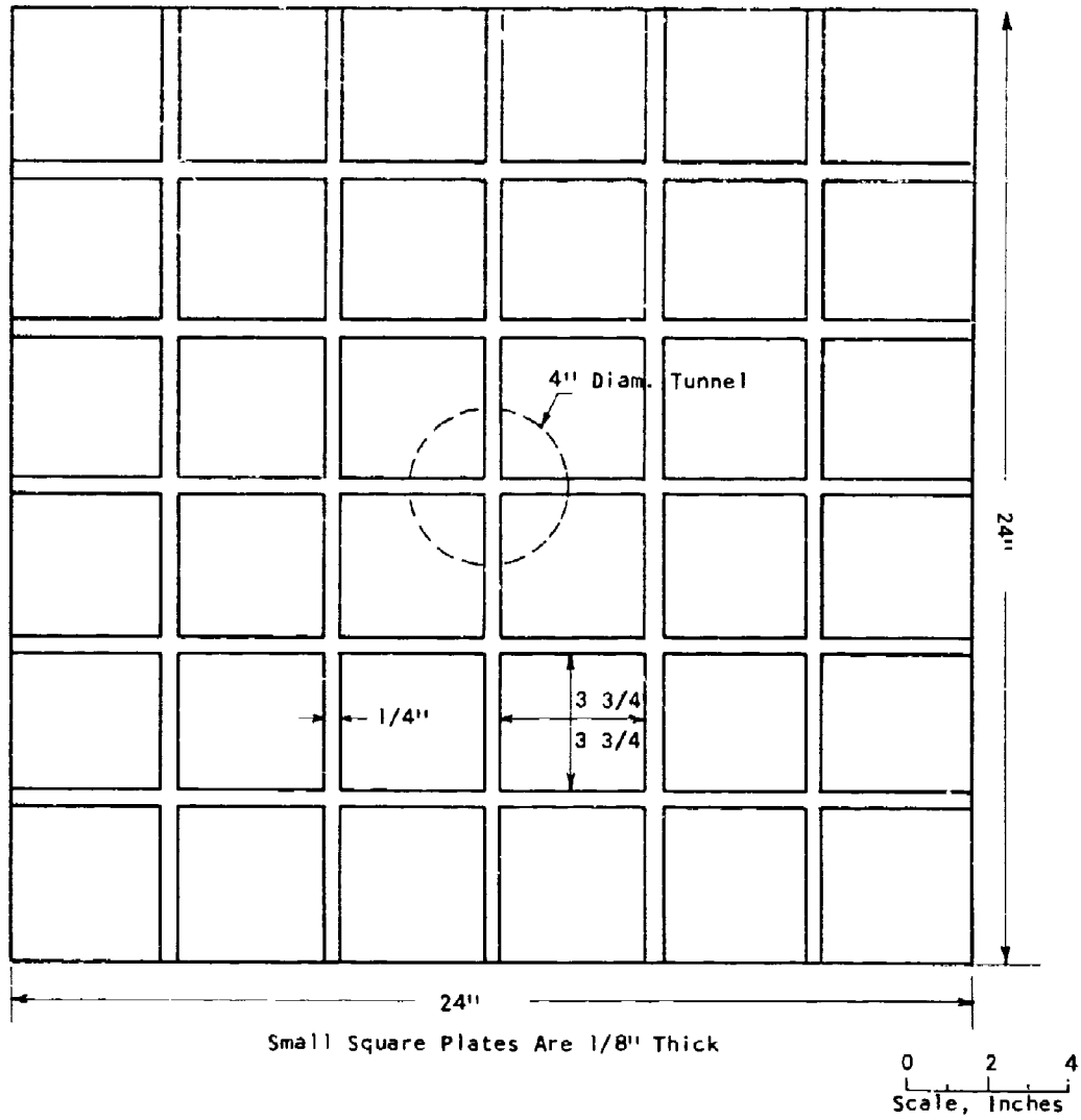
Figure 99 Sketch of Possible Friction Reducing System
