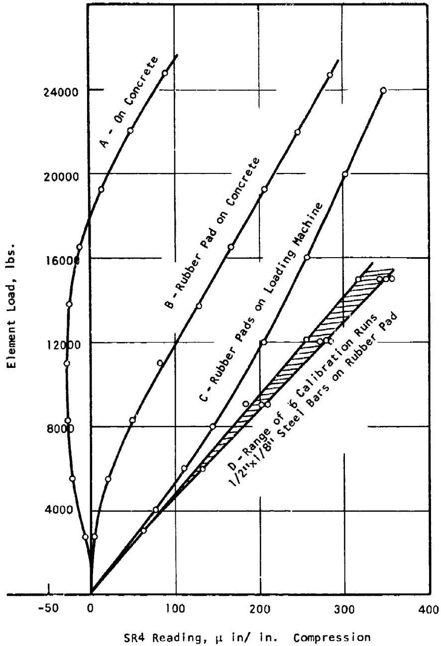
Figure 60 Calibration Curves For Element #3-1 On Different Surfaces
