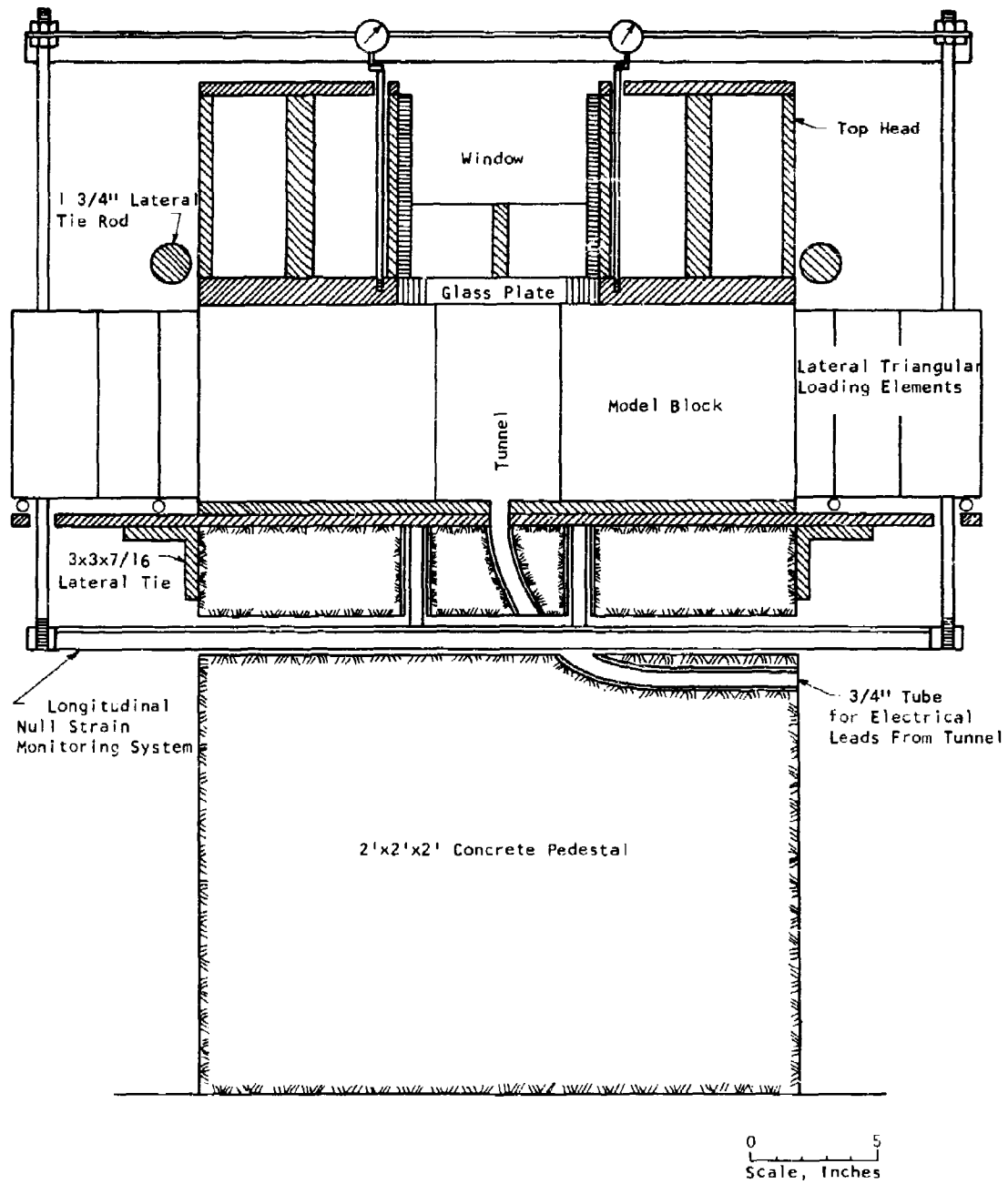
Figure 93 Schematic Diagram of Base and Loading Element Assembly
