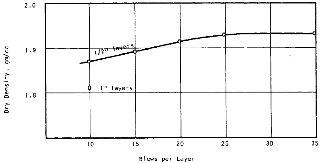
Figure 27 Compaction of Dry Plaster of Paris and Fine Wabash Sand, Mixed at 1/8, in 2" Diam. x 4" Long Molds with Vicksburg Tamper, No Extension on Mold
