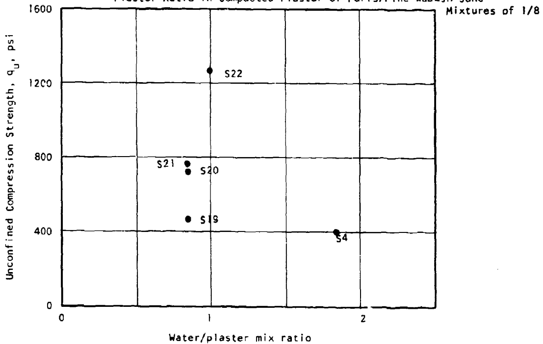
Fig. 37 Variation of Unconfined Compression Strength with Water/Plaster Ratio in Compacted Plaster of Paris/Fine Wabash Sand Mixtures of 1/8
