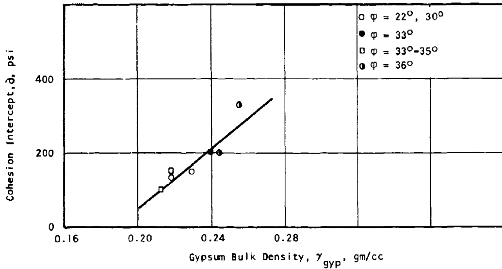
Figure 39 Variation of Cohesion Intercept With Bulk Gypsum Matrix Density Impact Compaction of Water/Plaster/Sand Mixtures
