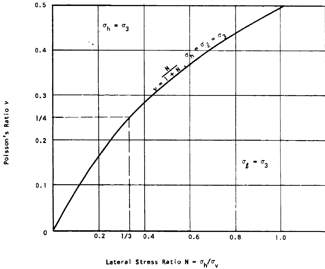
Figure 45 Variation of Minor Principal Stress With Values of N and v .
