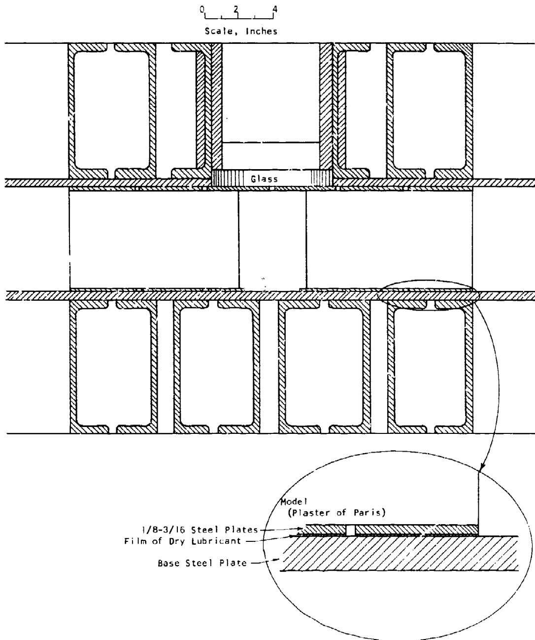
Figure 100 Sketch of Possible Friction Reducing System
