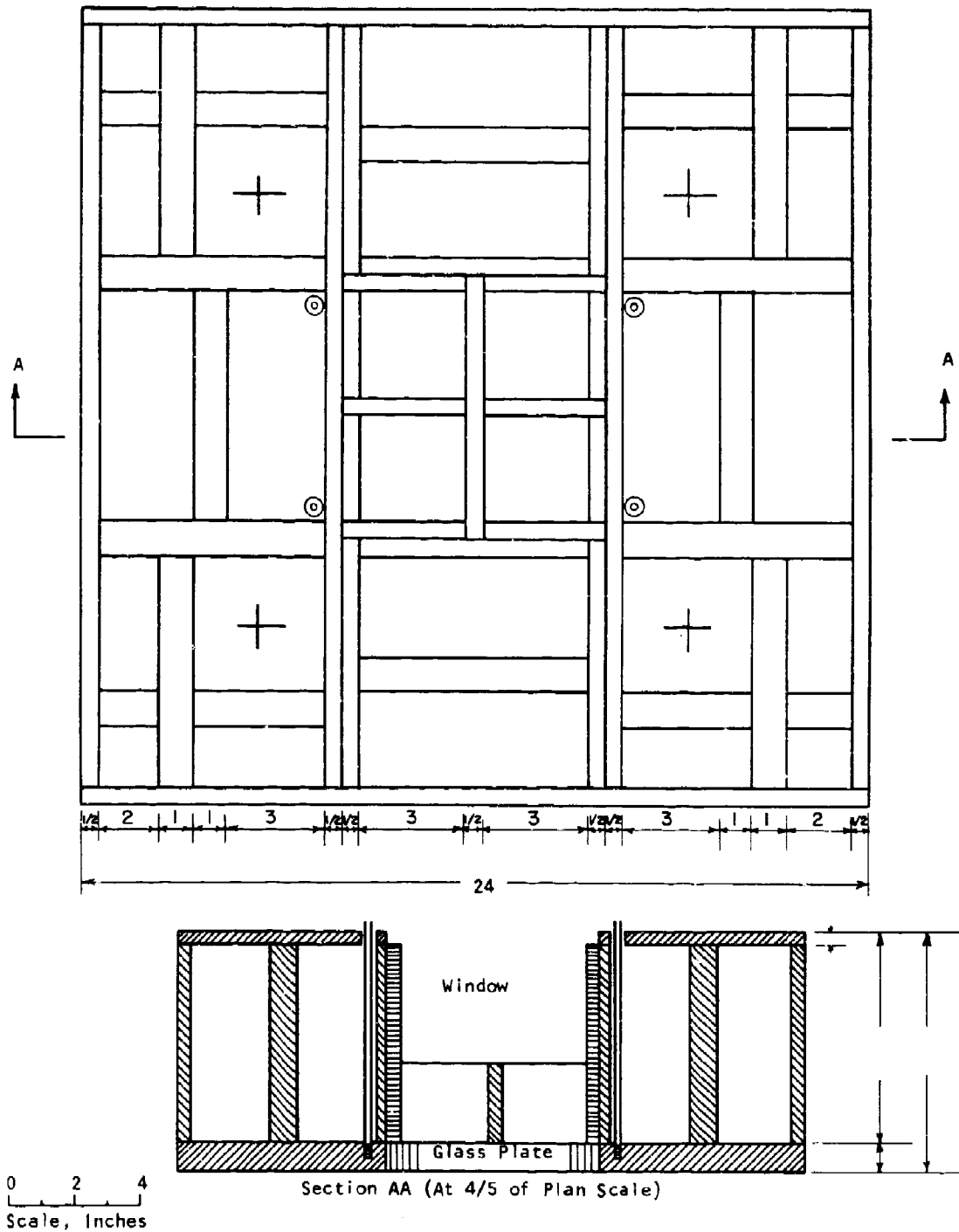
Figure 80 Plan and Section of Top Head. Window is 1"x8"x8" Plate of LOF Tuflex Glass. In Plan View, Crosses Mark Centers of Hydraulic Jacks, Circles Represent 1/2" Holes in Top Plate to Receive 1/4" Rod Threaded into Bottom Cover Plate.
