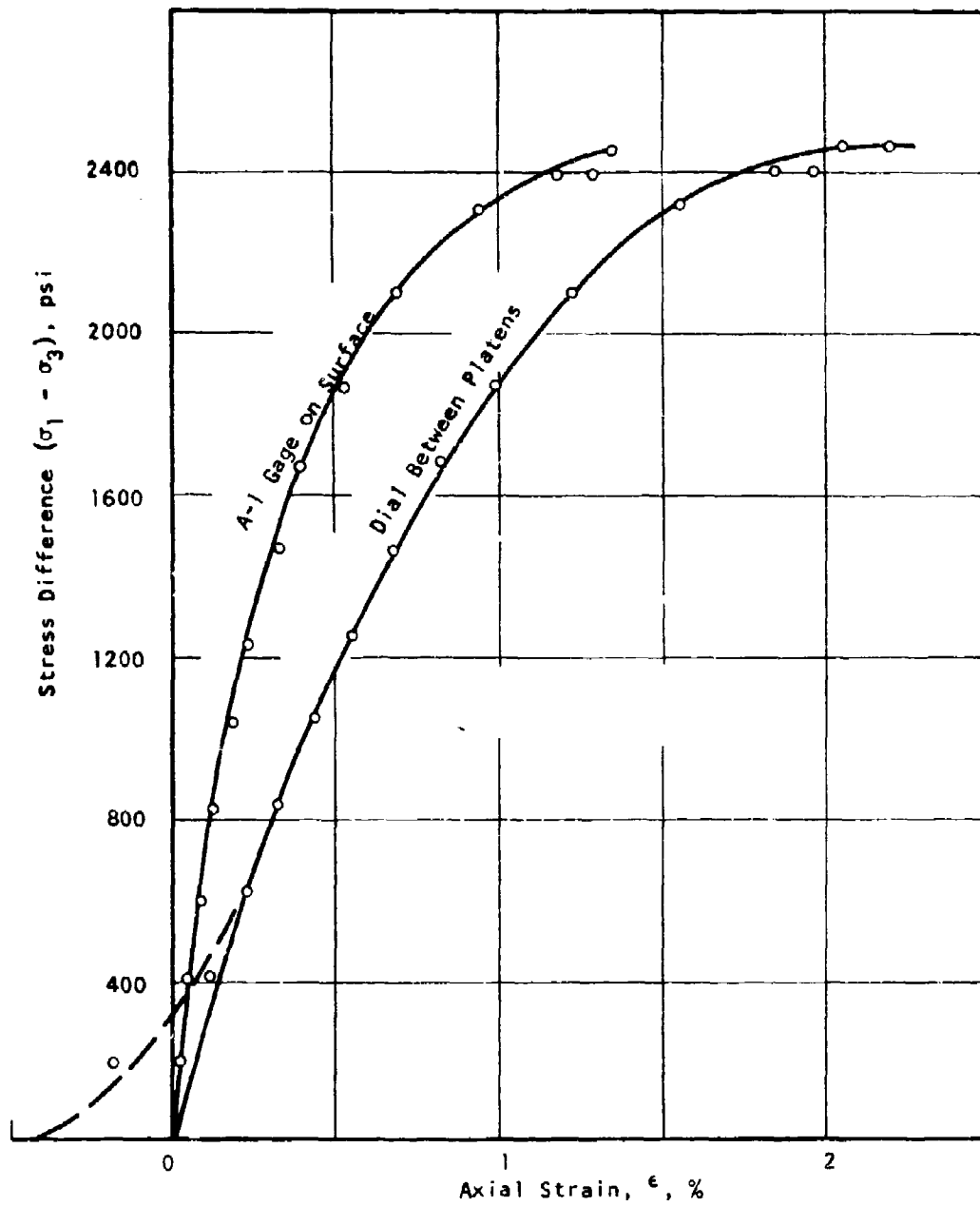
Figure 108 Stress-Strain Curves \sigma_3 = 500 psi Specimen S29-7
