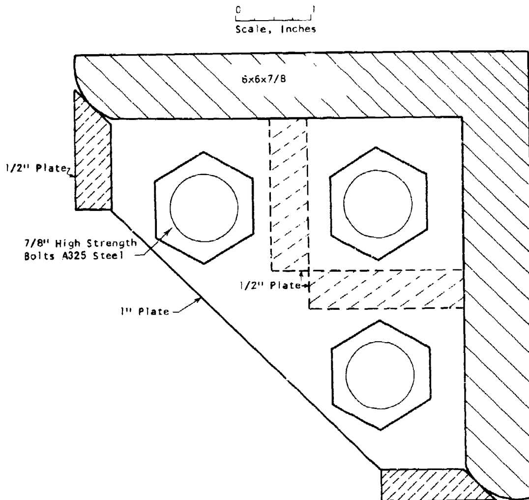
Figure 71 Sketch of Corner Connection Between Top and Bottom Heads
