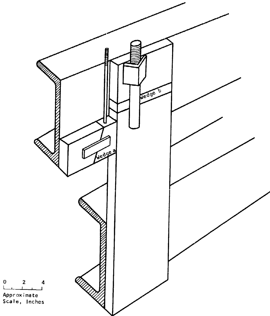
Figure 74 Sketch of End Connection
