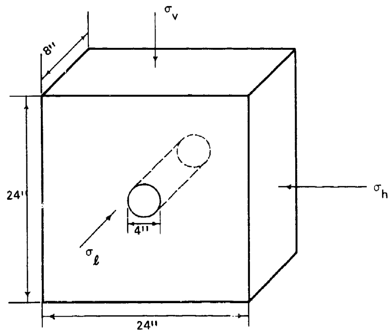
Figure 10 Proposed Model Block
