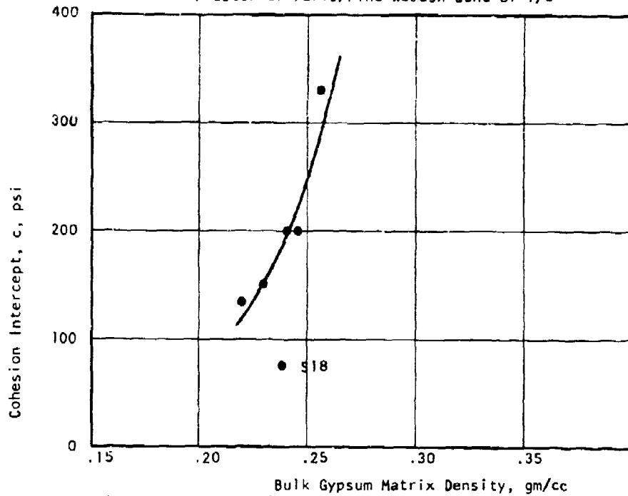
Figure 36 Variation of Cohesion Intercept of Mohr Diagram with Bulk Gypsum Matrix Density in Compacted Mixtures of Plaster of Paris/Fine Wabash Sand of 1/8
