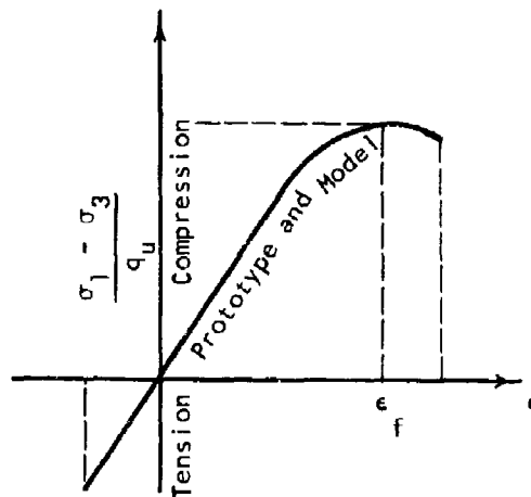
Figure 8 Prototype and Model Stress-Strain Curves
