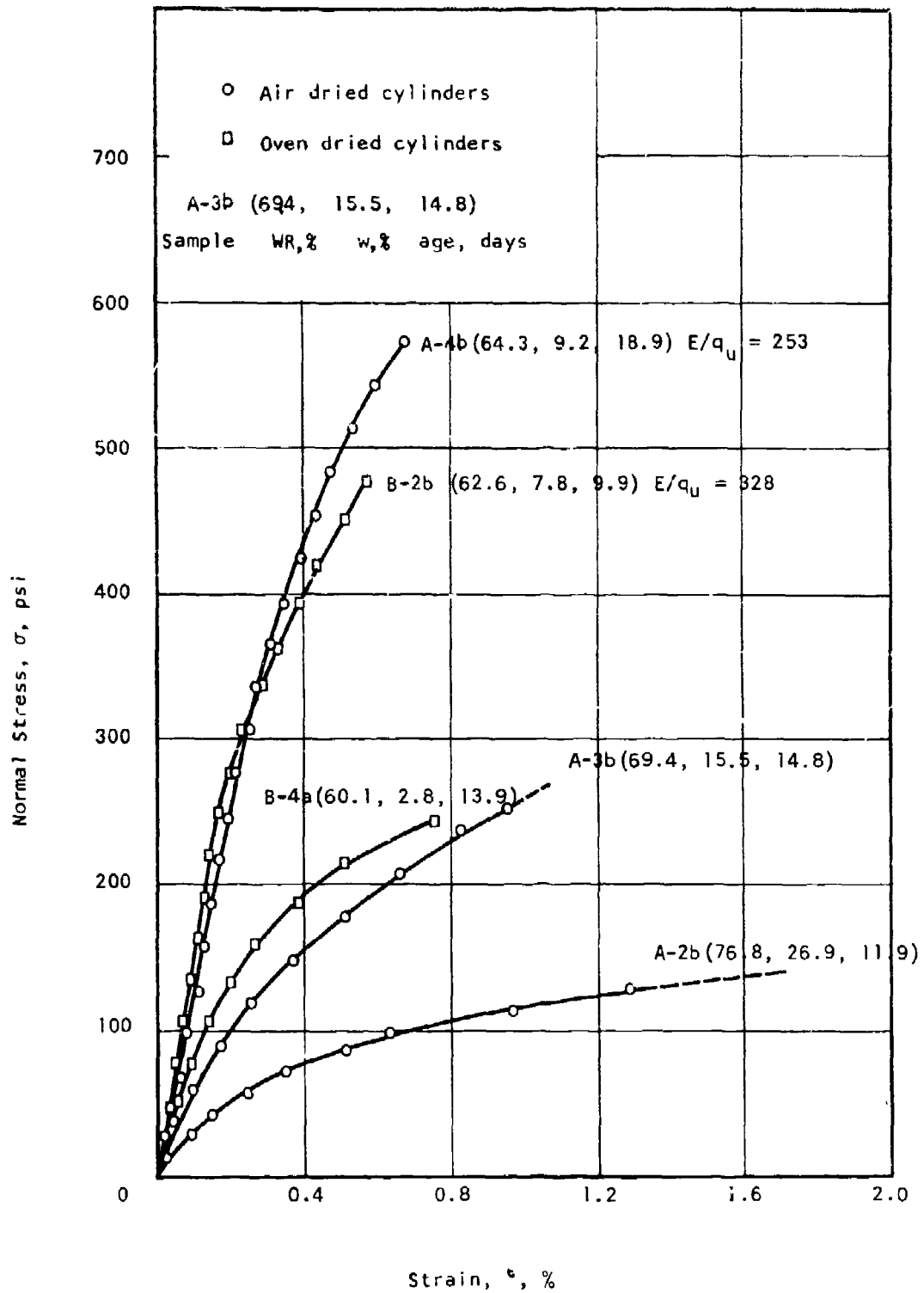
Figure 20 Typical Stress-Strain Curves Unconfined Compression
