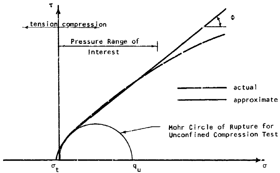
Figure 3 Failure Envelope Considered Typical For Rock
