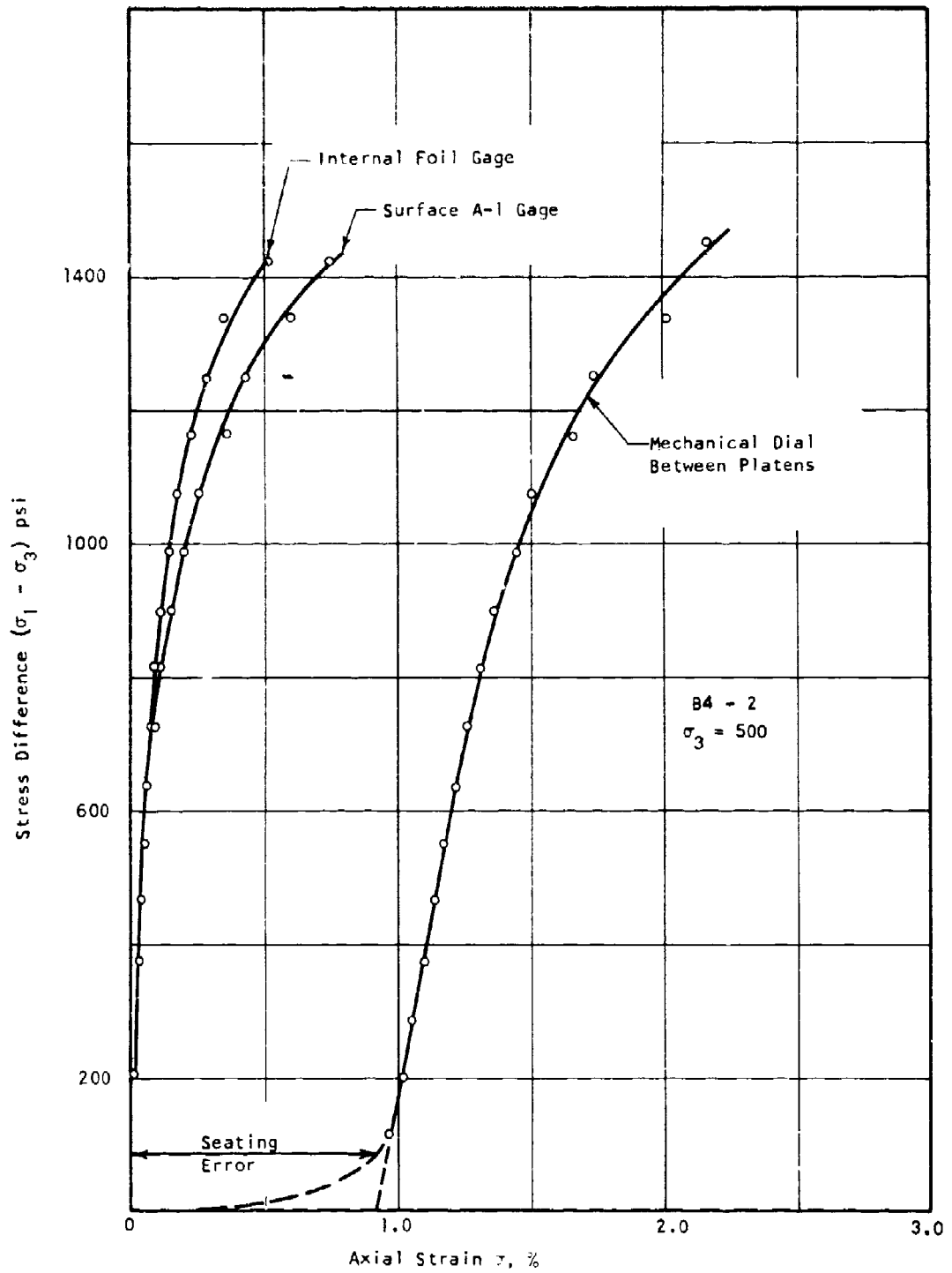
Figure 114 Stress-Strain Curves
