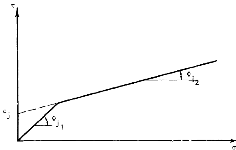
Figure 5 Typical Failure Envelope Along Rock Mass Discontinuities
