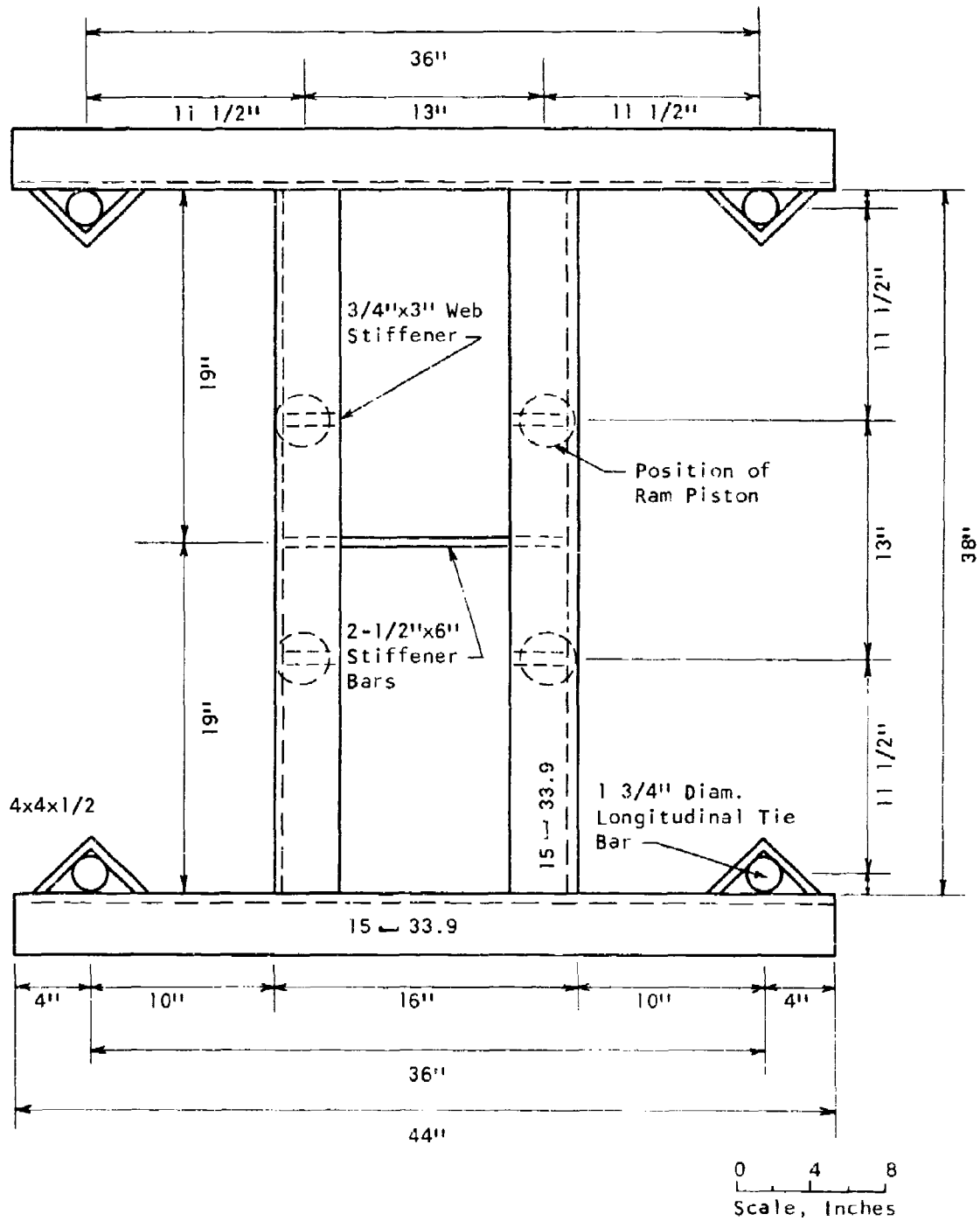
Figure 95 Top Longitudinal Reaction Head
