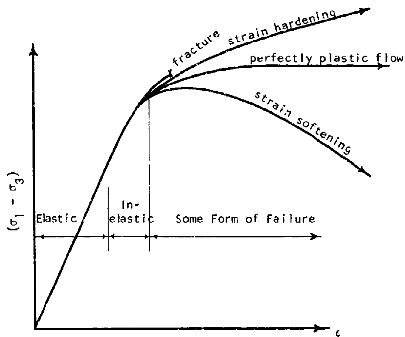
Figure 3 Failure Envelope Considered Typical For Rock
