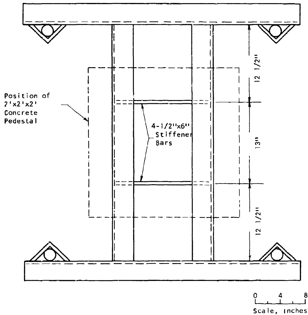
Figure 94 Bottom Longitudinal Reaction Head Details and Dimensions Not Shown Are Identical to Top Reaction Head
