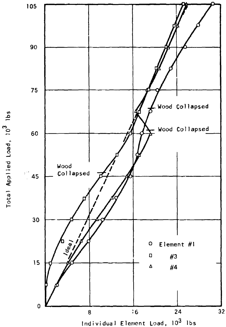
Figure 63 Load Distribution of Set of Triangular Elements
