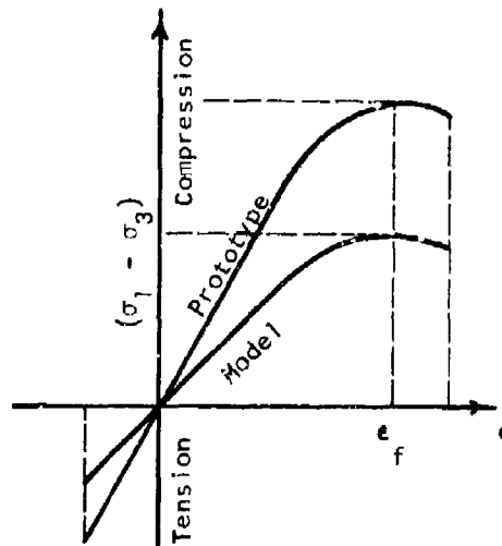
Figure 8 Prototype and Model Stress-Strain Curves
