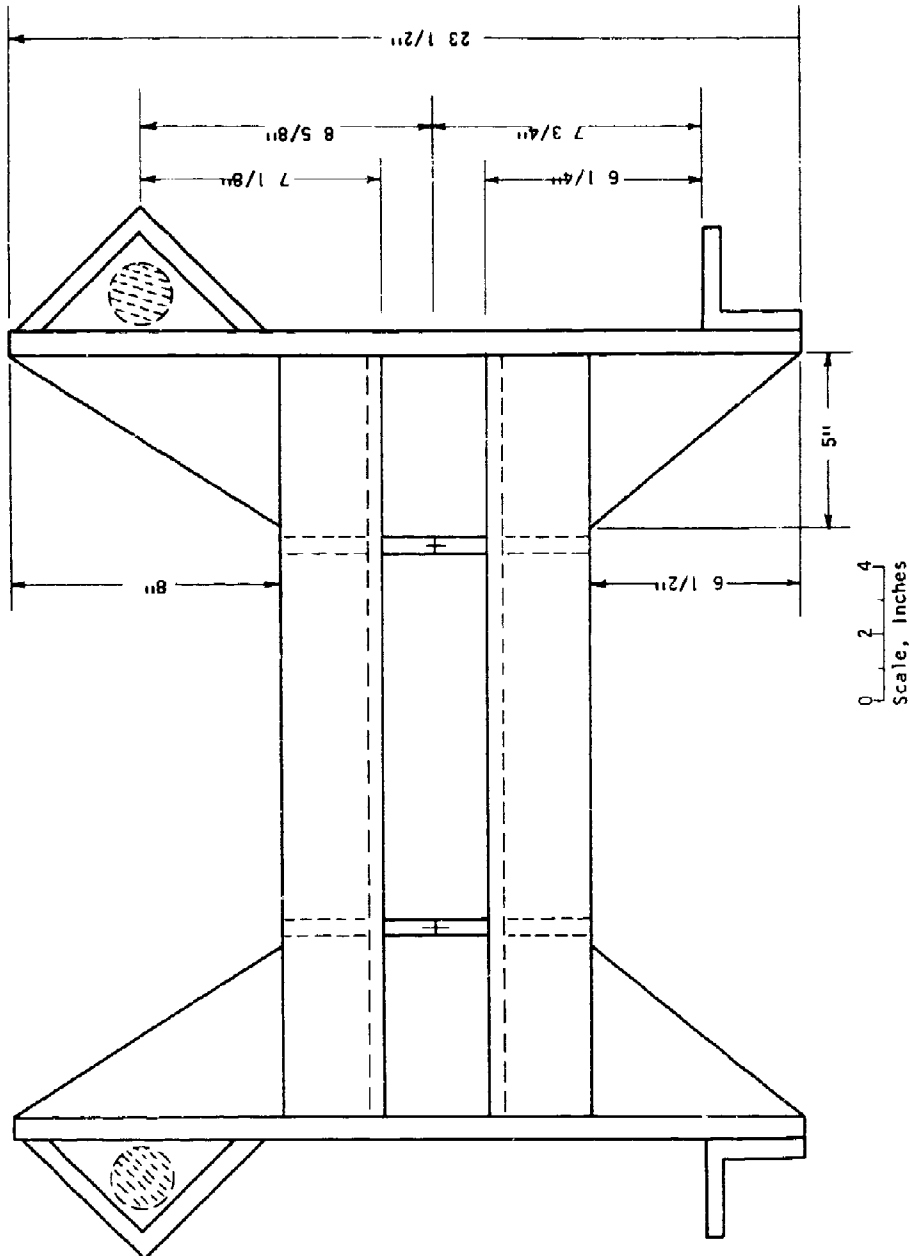
Figure 89 Longitudinal End Reaction in \sigma_H Direction Details and Dimensions Not Shown Are Identical to \sigma_V Ends
