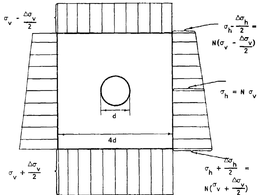
Figure 1 Stress Distribution Some Distance From Tunnel
