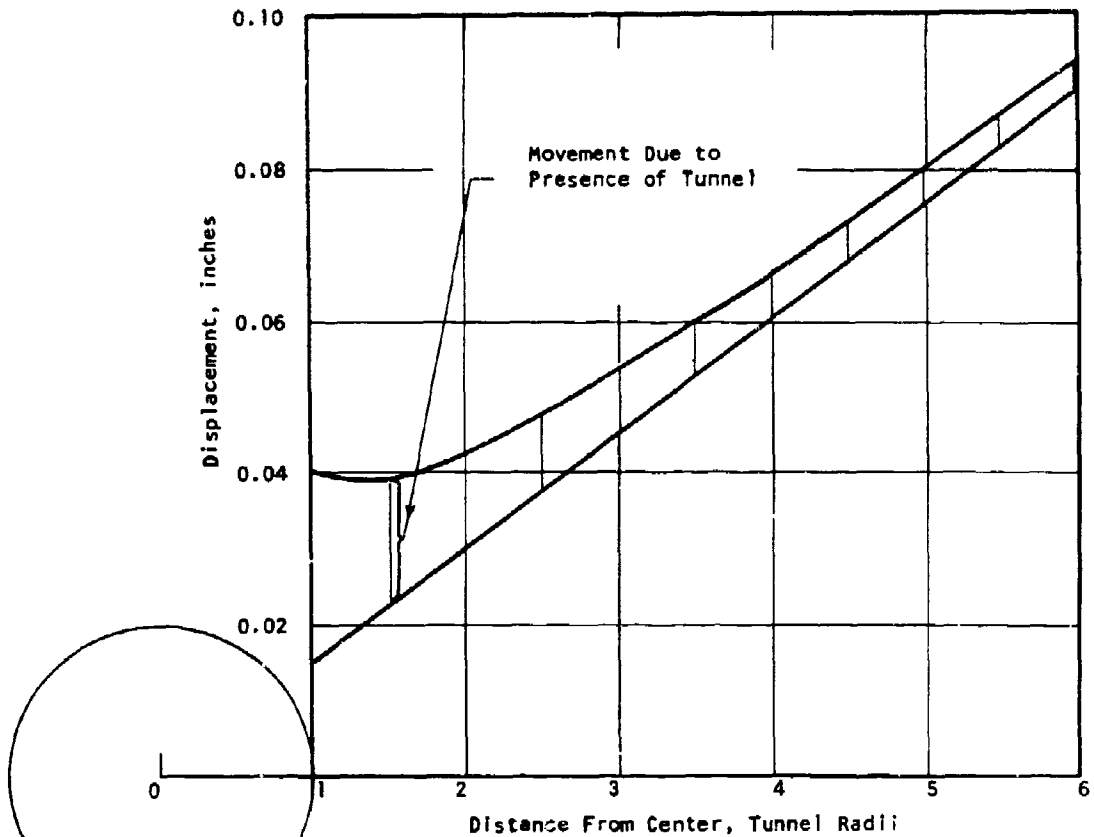
Figure 49 Inward Movement Radially Toward Center of Block
