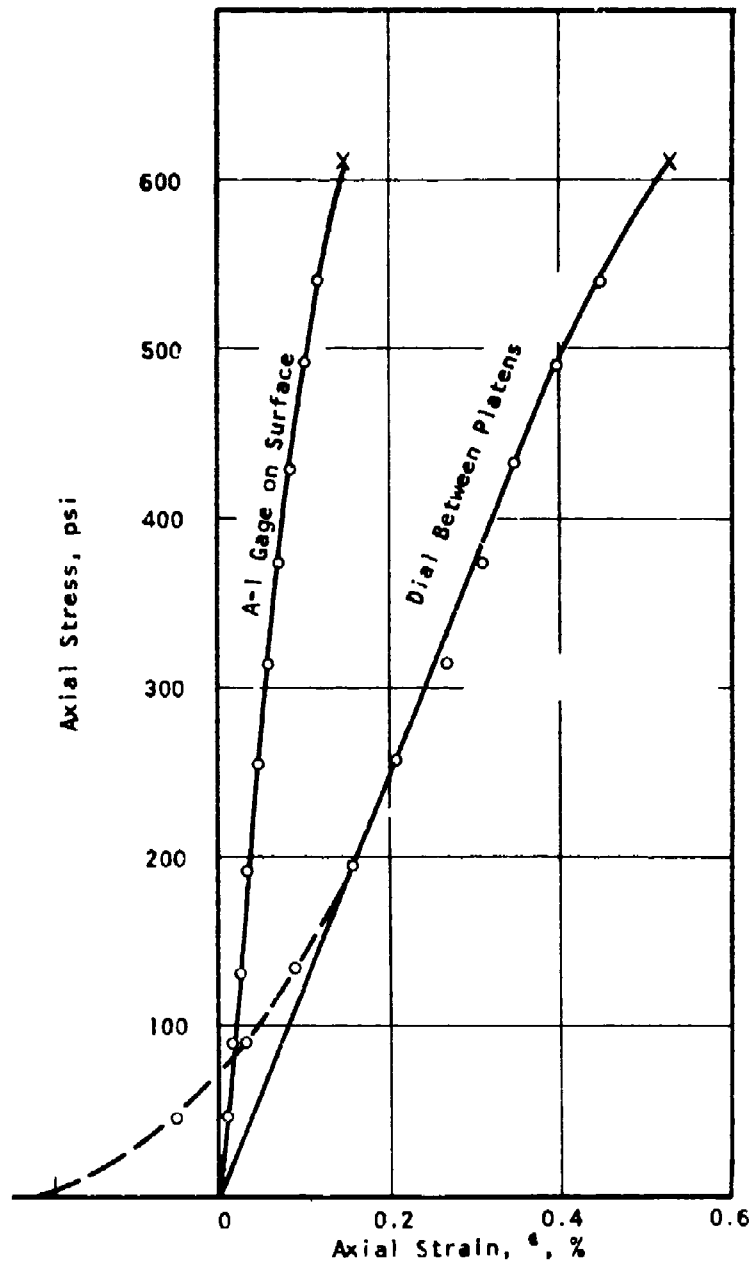
Figure 107 Stress-Strain Curves \sigma_3 = 0 Specimen S29-1
