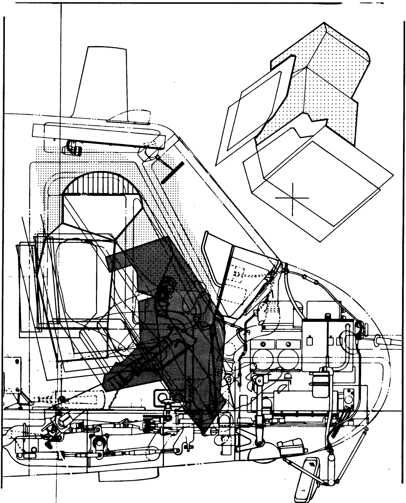
Fig. 33b. ARMOR CONFIGURATION 1 -- SIDE VIEW 45° AZIMUTH, -45° ELEVATION
