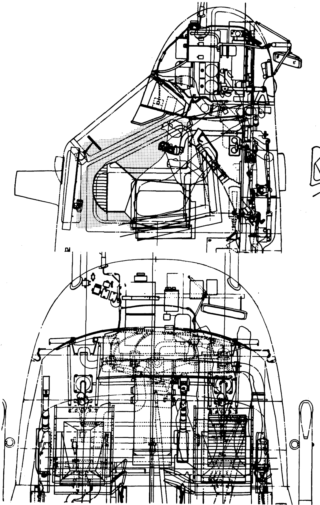
Fig. 27a. UH-1 INBOARD PROFILE/TOP VIEW
