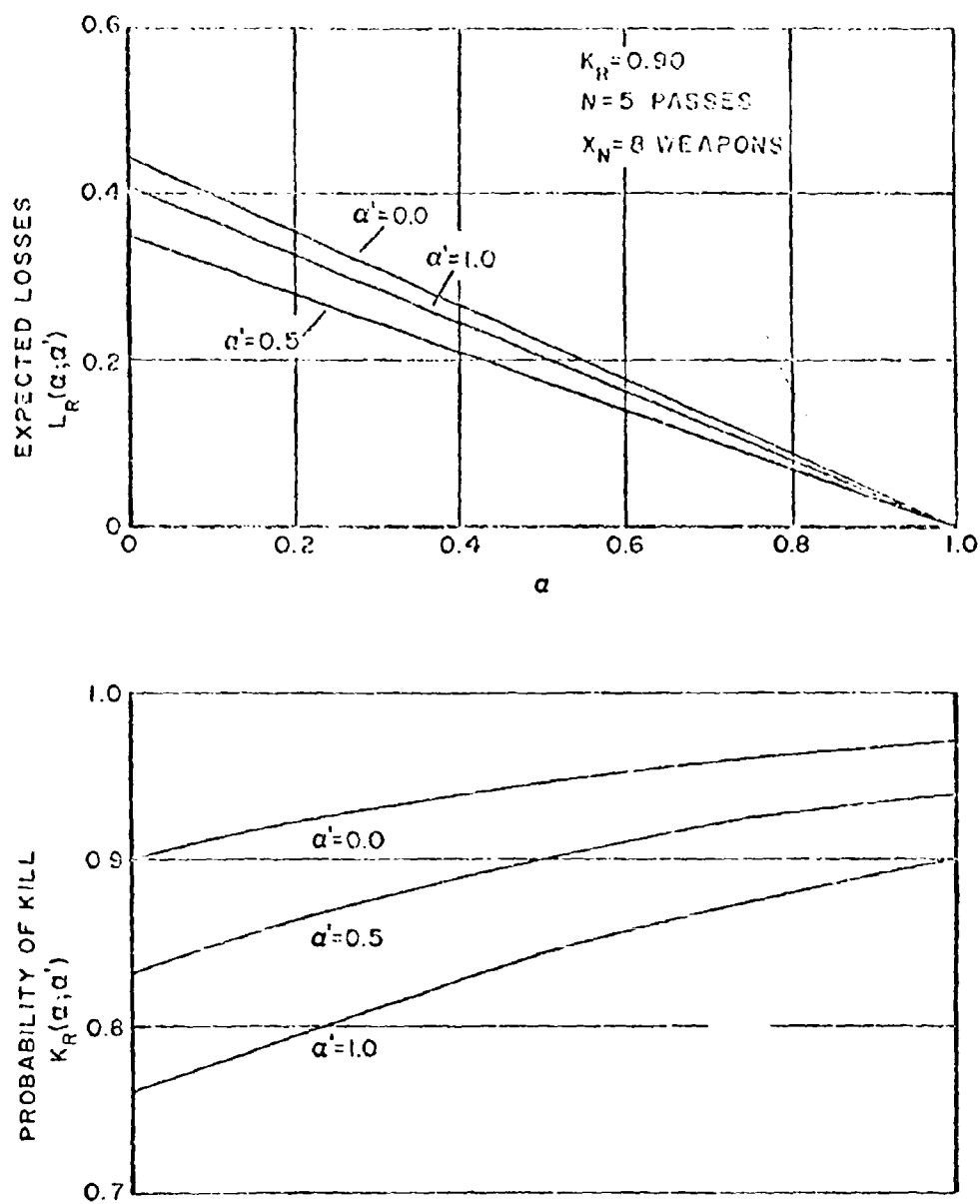
Fig. 32.--Profiles of system performance: P_K duel raid model.
