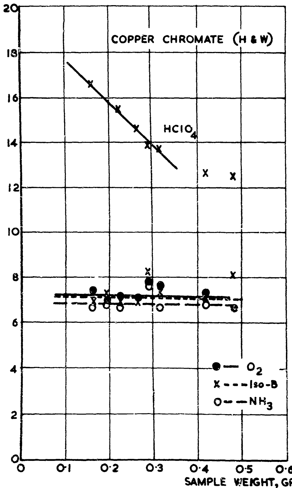
FIG.4. PERCENTAGE WEIGHT CHANGES WITH VARIOUS REACTIVE GASES FOR DIFFERENT WEIGHTS OF COPPER CHROMATE (H & W)
