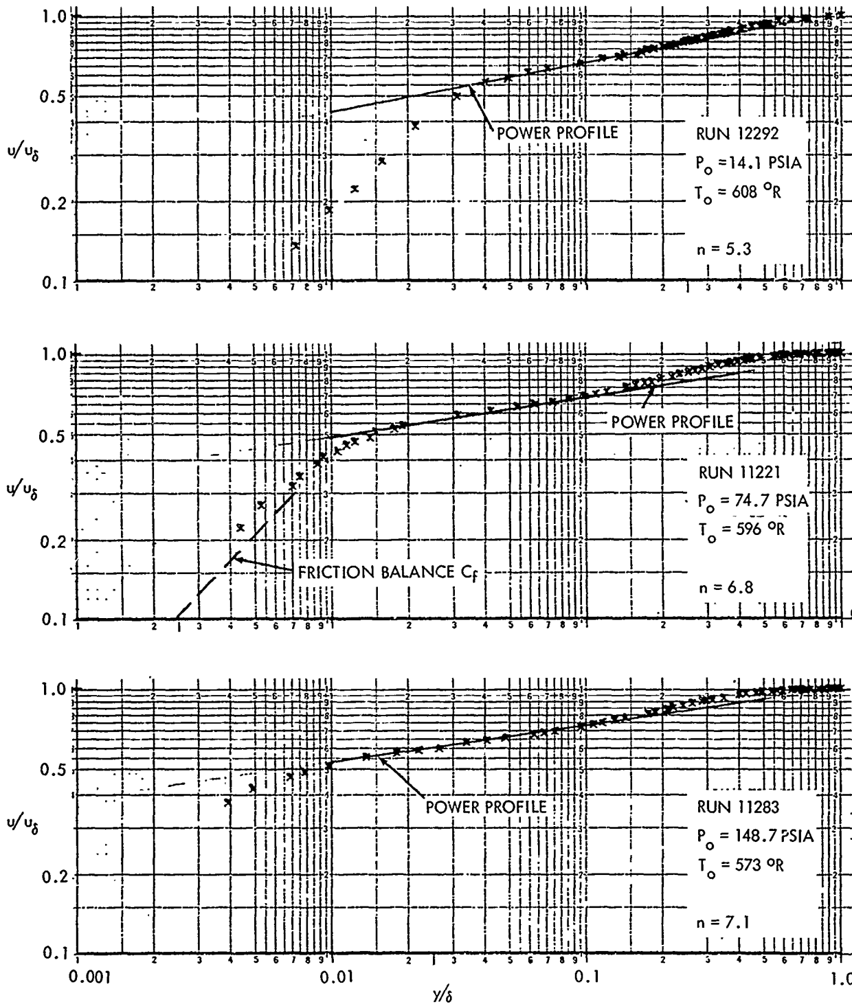
FIG. 5c(1) VELOCITY PROFILE AT THE 72 INCH STATION
