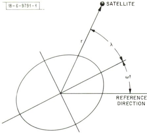
Fig. 1. Reference system for elliptic earth.
