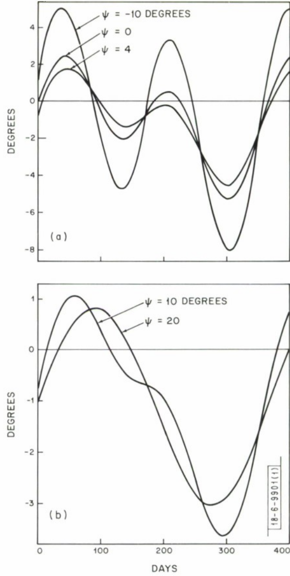
Fig. A-2. Salar time as seen on the sotellite for different angles of tilt.
