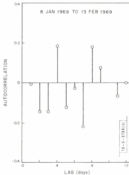
Fig. 27. Autocorrelation of the sensor errors (fourth period).
