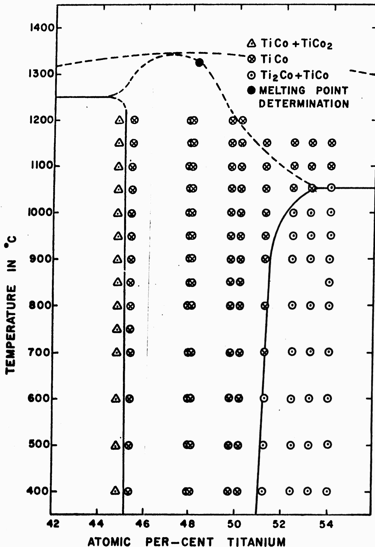
Fig. 1 - PHASE RELATIONSHIPS NEAR THE EQUIATOMIC COMPOSITION AS ESTABLISHED BY HIGH TEMPERATURE X-RAY DIFFRACTOMETRY.
