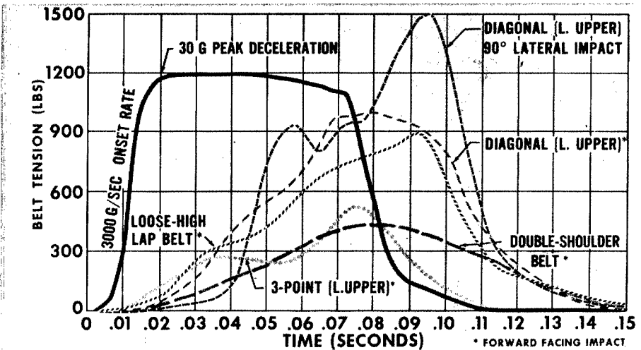
Figure 2. Comparison of belt loads in baboon subjects 30 G impact with four restraint systems.
