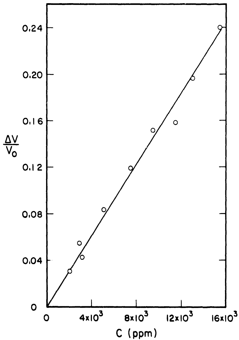
Figure 10. Calibration curve for 0.1 mm glass beads.
