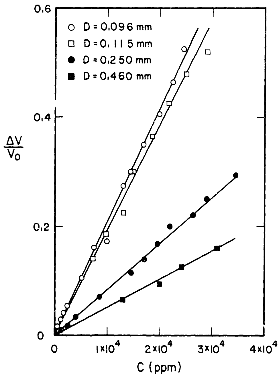
Figure 8. Calibration curves obtained for four different sand sizes.
