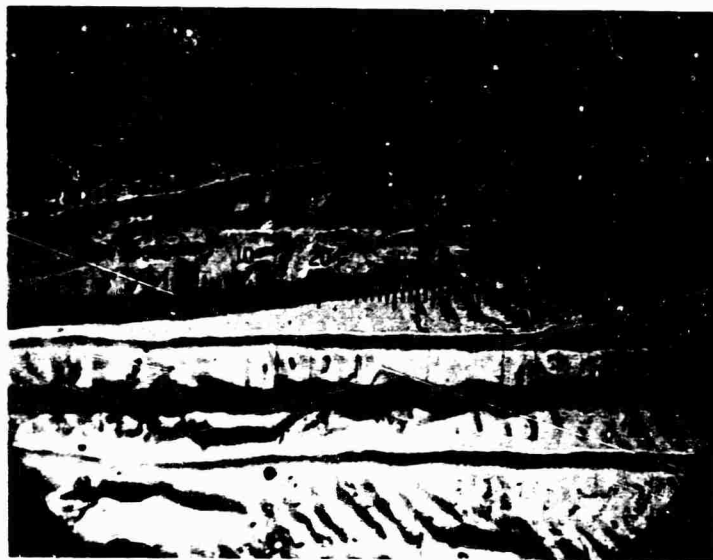
a) River pattern observed during continuous crack propagation of cast PMMA (Mag. 100x)
