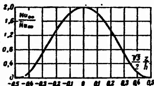
Fig. 14-2. Distribution of local values of Nu_{\infty} along side of triangular tube.
