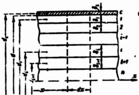
Fig. 10-3. Derivation of heat-balance equations.
