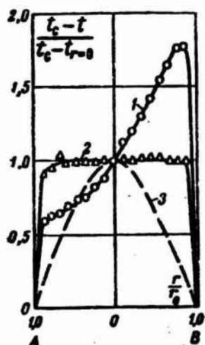
Fig. 14.23. Temperature distribution in curved tube with D/d = 40 and Re = 4000 . 1) In AB plane; 2) in CD plane; 3) the same, straight tube.
