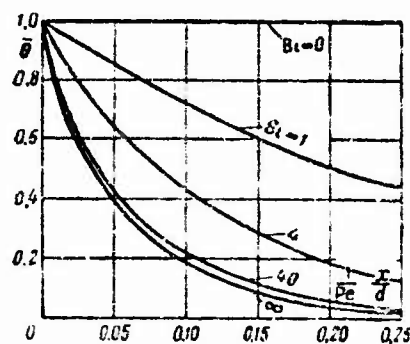
Fig. 11-2. Variation in \bar{\theta} along length of round tube for various values of Bi.
