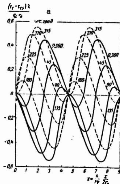
Fig. 17-19. Difference in wall temperatures for pulsating and stationary flows at M = 1.0 ; \text{Pr} = 0.7 ; \gamma = 1 . a) deg.
