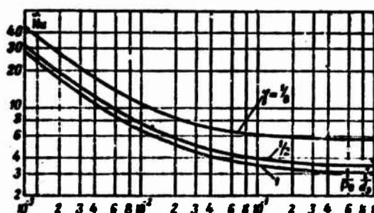
Fig. 14-5. Dependence of \overline{Nu} as function of \frac{1}{Pe \cdot d_o} at values \gamma = 1 , 1/2 , and 1/8 for a rectangular tube with t_s = \text{const} .
