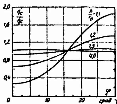
Fig. 14-15. Distribution of local heat-flux density over cylinder circumference for various values of b/r_0 . 1) deg.
