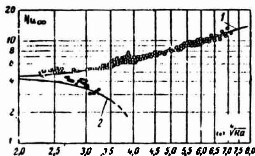
Fig. 16-27. Nusselt number from data of theoretical computation (curves) and experiment (circles). 1 - \frac{\partial \theta}{\partial x} > 0 ; 2 - \frac{\partial \theta}{\partial x} < 0 .
