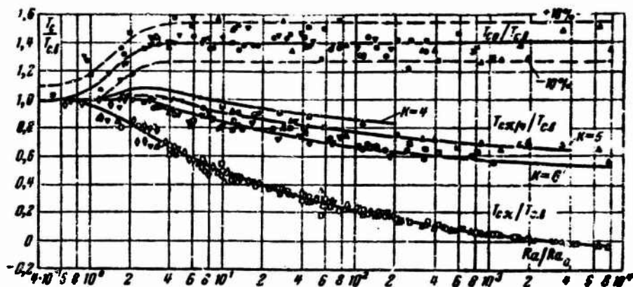
Fig. 16-36. Comparison of Eq. (16-56) (solid lines) with experimental data (points) for Ra = 2 \cdot 10^5 - 4 \cdot 10^7 and Re = 50 - 2400 .
