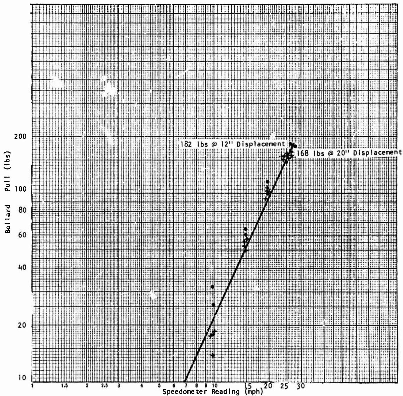
FIGURE 36. BOLLARD PULL TESTS - REAR WHEEL DRIVE ONLY, WHEEL PUMPS WITH 50% EXIT NOZZLE 7.50-16 NDCC TIRES, SKIRTS
