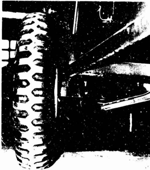
FIGURE 8. WATER COLLECTOR MOUNTED ON FRONT SUSPENSION (REAR VIEW)
