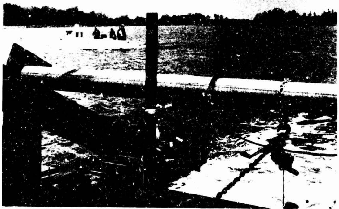
FIGURE 12. LOAD-CELL CONNECTION BETWEEN TEST VEHICLE AND SUPPORT RAFT
