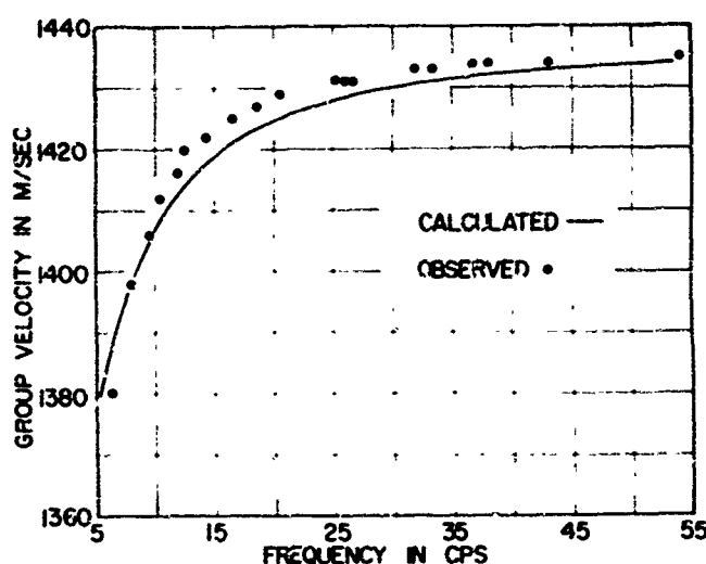
FIG. 13. Observed dispersion of waves of the first mode from several shots compared with first mode computed for model given in Table 1. From Hunkins and Kutschale (1963).
