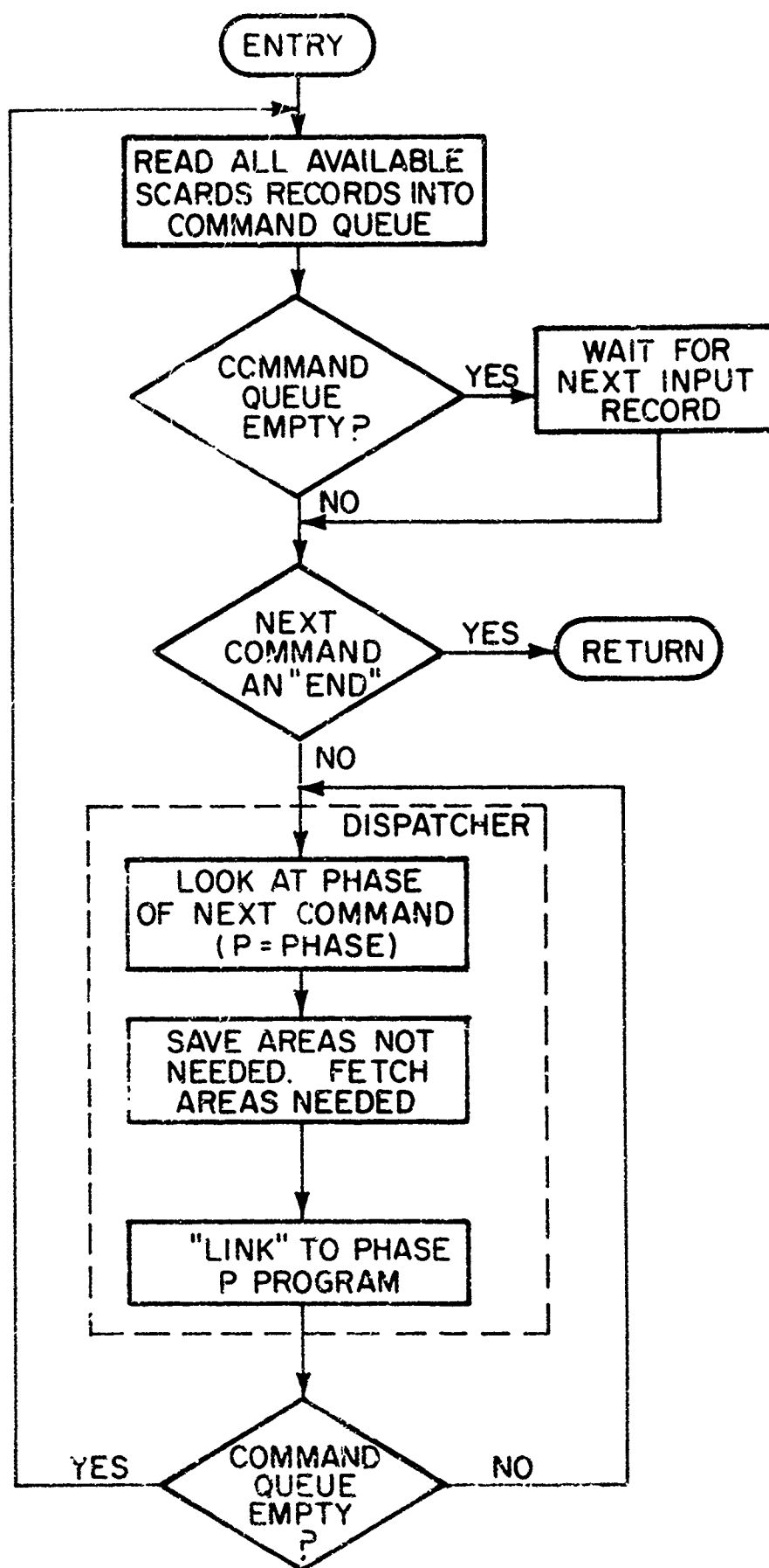
Figure 2.1 Supervisor flow diagram
