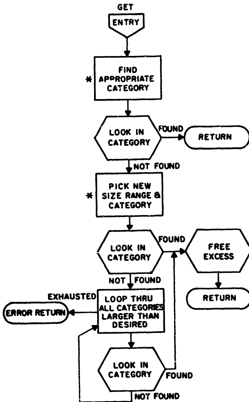
Figure A2 Flow Chart for GET Function
