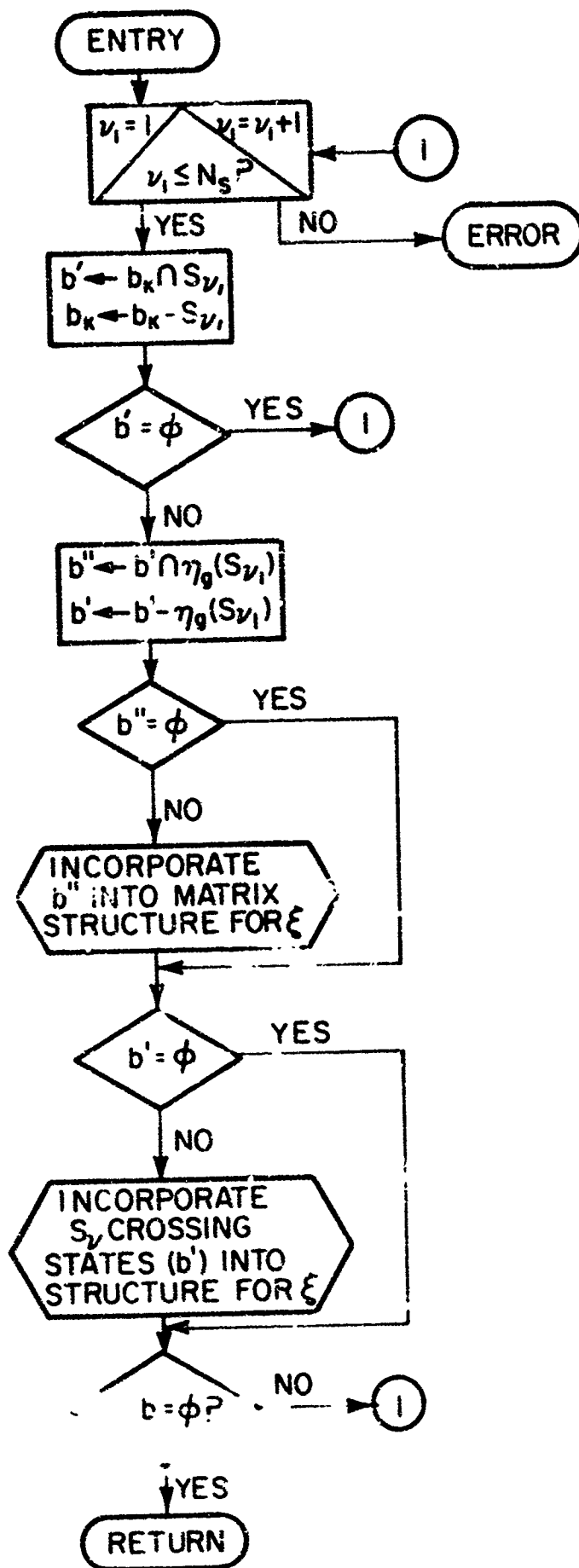
Figure 6.5 The matrix-event generator.
