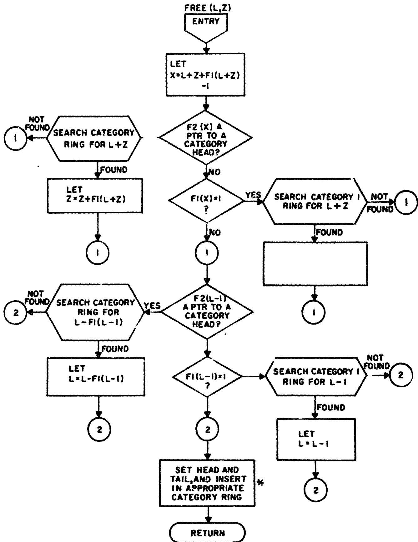
Figure A3 Flow Chart for FREE Subroutine
