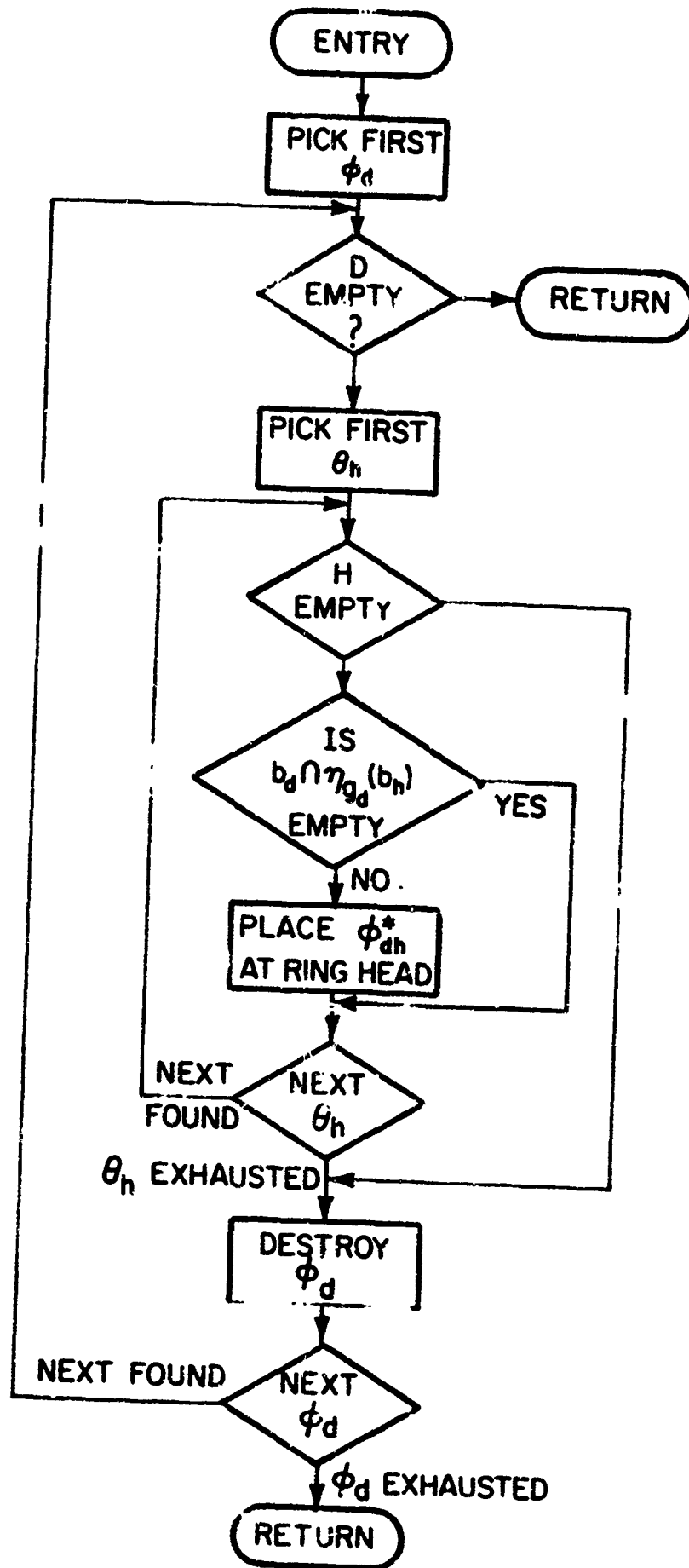
Figure 5.13 Flow diagram: Event set consolidator.
