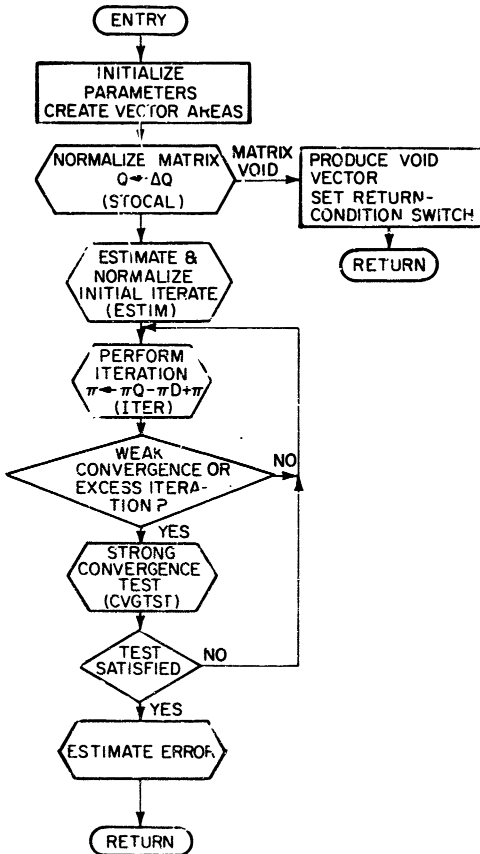
Flow diagram for state proximity solver.
