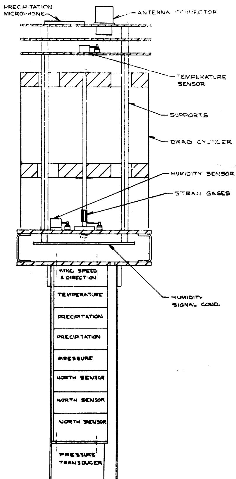
Figure 2-29. Sensor Package
