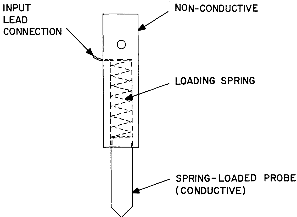
Figure 4-13. Terminal Probe
