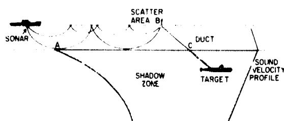
Three-part model of propagation losses. A, duct loss; B f , forward scatter loss; and C, ray path loss.
