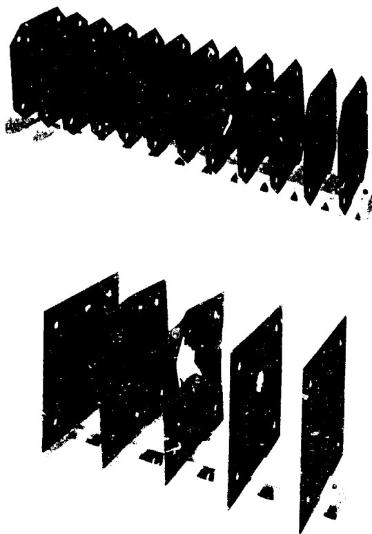
A 1-gram steel sphere impacting at 5,500 feet per second is able to perforate eleven 1/16-inch-thick aluminum plates spaced 4 inches apart (above). The same projectile impacting at 15,000 feet per second, however, is able to perforate only three of the same target plates (below).
