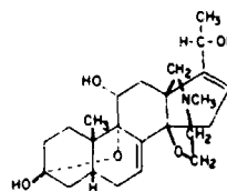
Chemical formula of batrachotoxinin A, C_{24}H_{35}NO_5 (R = H, Br, C_6H_4CO- ).
