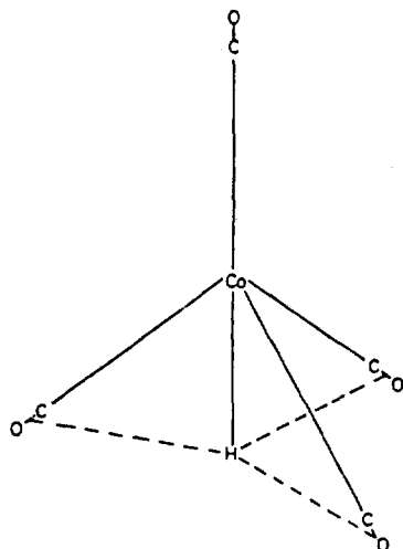
Molecular model of \text{HCo(CO)}_4 . Intramolecular interactions between the axial hydrogen atom and the equatorial carbon monoxide molecules in \text{HCo(CO)}_4 are shown by the dashed lines. These interactions, accounting for observed infrared properties, can be deduced from mass spectral fragmentation studies.
