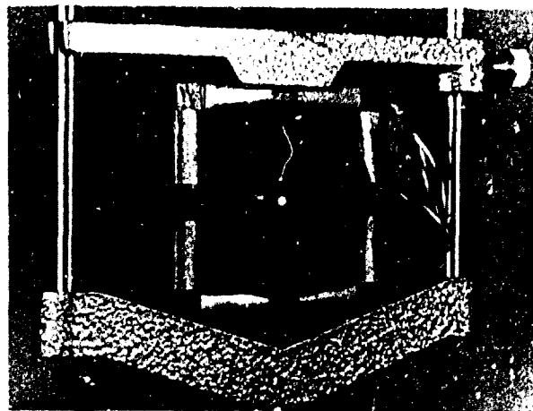
Apparatus used to achieve optical frequency translation of laser light beams. The birefringent single-crystal YIG rod is the light dot in the center of the field coil assembly (the four dark areas around the YIG).
