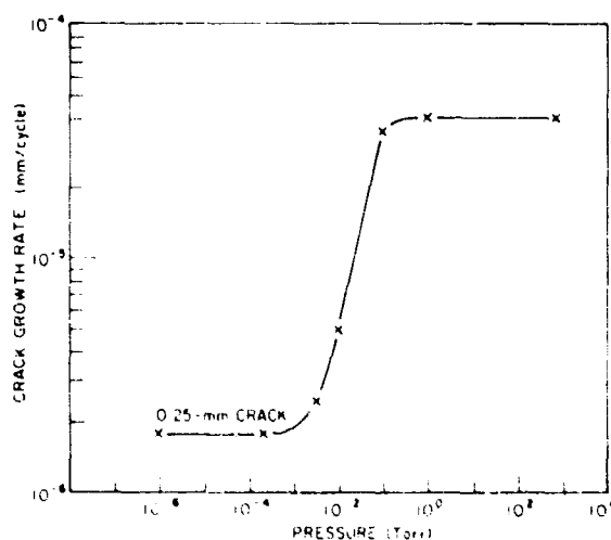
Effect of oxygen pressure at 500^\circ\text{C} on rate of fatigue crack growth for Type 316 stainless steel at a bonding strain of 0.141 percent
