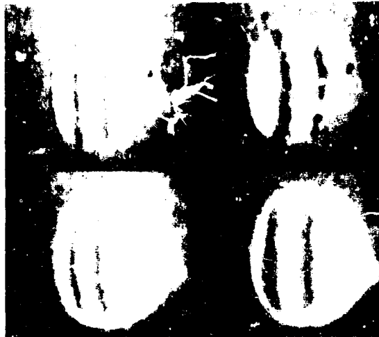
Interferograms through a neodymium-glass laser rod before pumping (upper pictures) and during pumping (lower pictures). Left: Laser rod is in water of constant temperature. Thus, before pumping, the fringes are straight (upper picture), indicating no distortion. After pumping (lower picture), they become distorted. Right: Water temperature is decreased before start of pumping. Thus, the fringes are initially curved (upper picture) but become straight during pumping (lower picture) when compensation is achieved.
