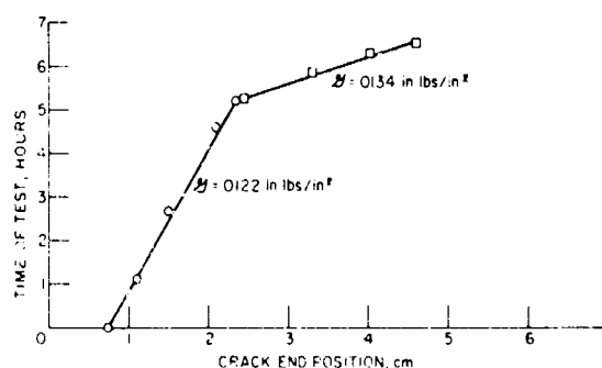
Crack length as a function of a constantly applied driving force, G . The slope of the line gives the rate of crack propagation. (Test for 3 \times 12 \times 0.127 -inch plate glass conducted at 74^\circ\text{F} and at almost 100 percent relative humidity.)
