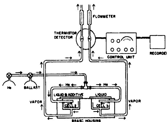
Dual-cell thermal conductivity apparatus used at NRL for measuring relative rates of evaporation of volatile liquids.
