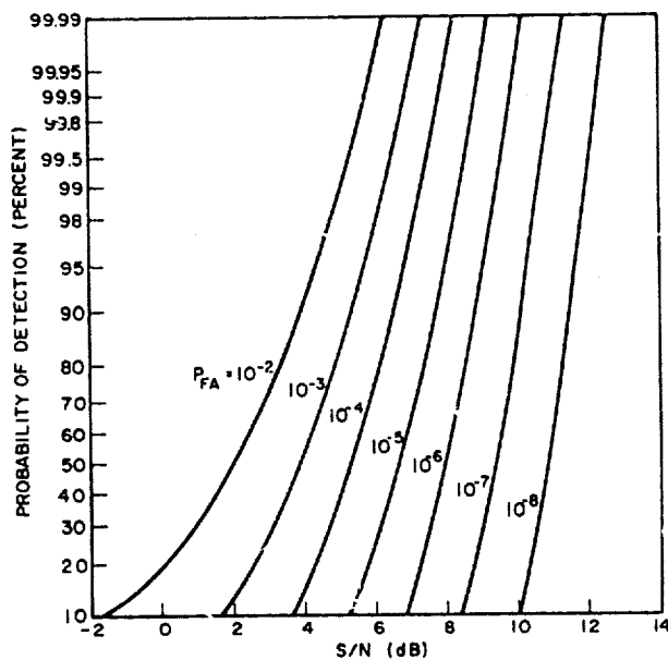
Probability of detection versus S/N according to the log-normal clutter model for probability of false alarm ranging from 10^{-2} to 10^{-8} and with \sigma = 6 decibels and number ( N ) of pulses integrated = 30.
