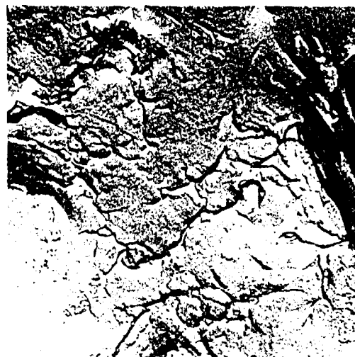
Electron micrograph of replica of stress-corrosion fracture surface of a steel alloy. Broad featureless areas are considered to be due to simultaneous chemical action and stress. Ridges are interpreted as being formed by ligaments resistant to chemical effects that undergo plastic straining until they are torn apart. Magnification: 60,000X.
