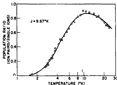
Typical electron paramagnetic resonance data used to determine the exchange constant J of exchange-coupled \text{Mn}^{2+} pairs in \text{KZnF}_3:\text{Mn}^{2+} . The population of the S = 1 state (ratio of pair to single ion intensity) of a nearest-neighbor \text{Mn}^{2+} pair is plotted as a function of temperature and compared with the theoretical expression for that state (solid line). The value J = +9.67^\circ\text{K} is found from a least-square fit of the data to theory.
