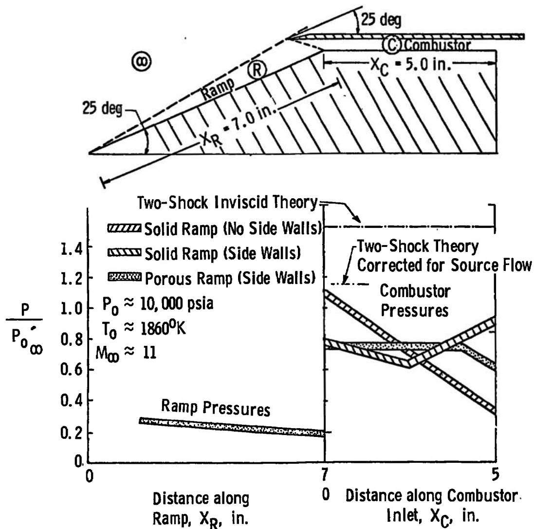
Fig. 10 Summary of Static Pressure Recovery
