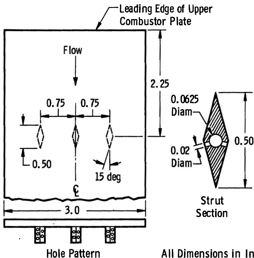
Fig. 4 Strut Injector Detail
