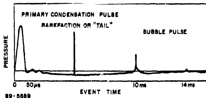
Figure 2 REPRESENTATIVE ELECTRODELESS SPARK PRESSURE WAVEFORM
