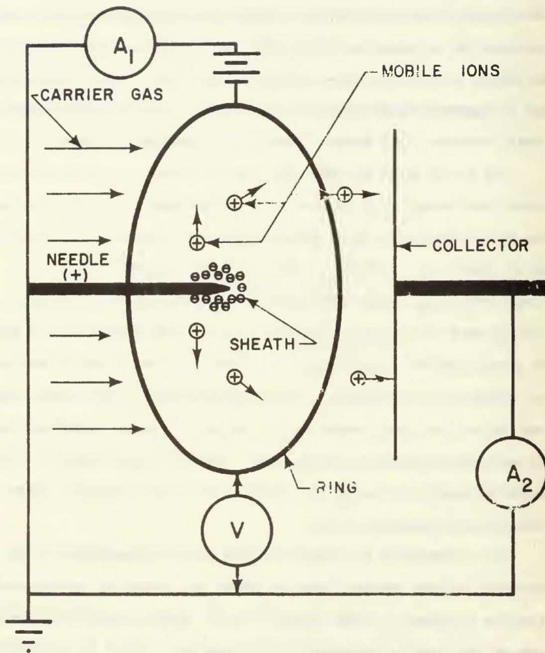
FIGURE I GENERATOR SCHEMATIC
