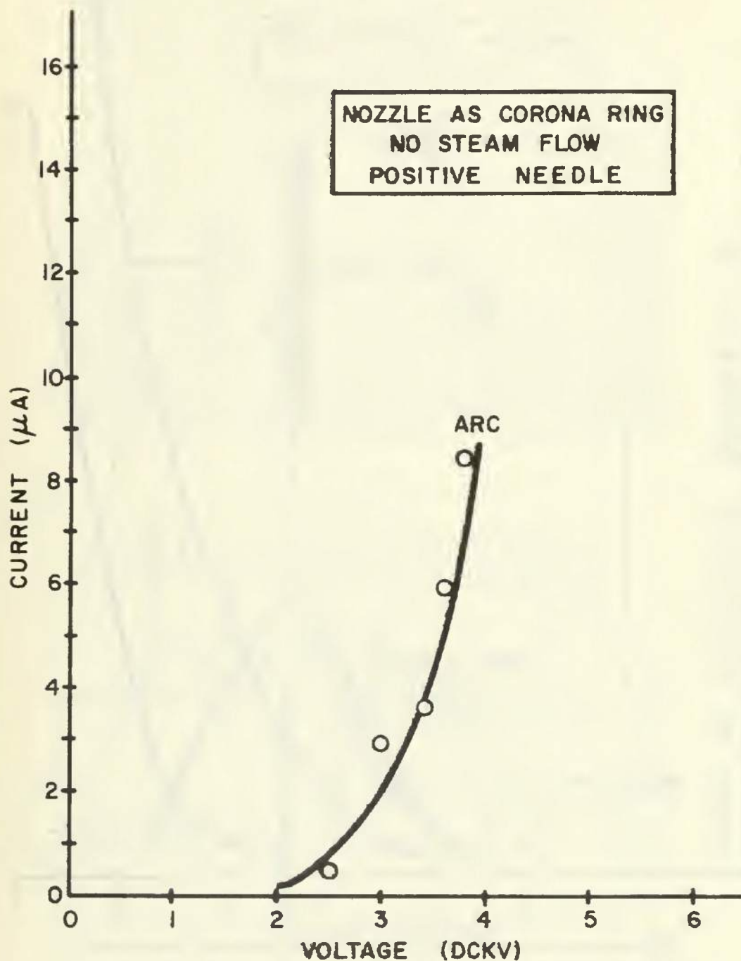
FIGURE X CORONA CURRENT VS VOLTAGE MICRON INJECTOR UNIT
