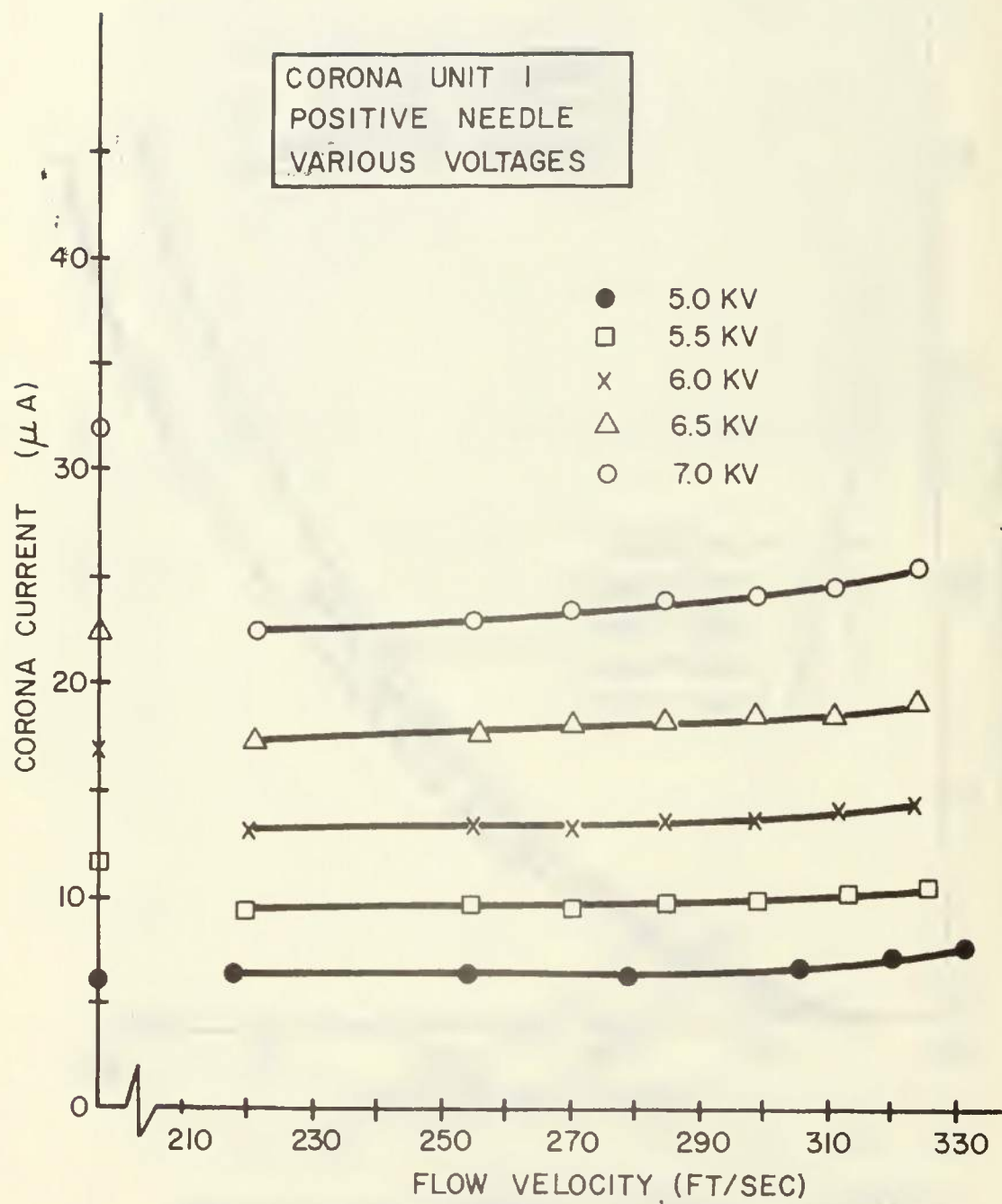
FIGURE 16. CORONA CURRENT VS FLOW RATE
