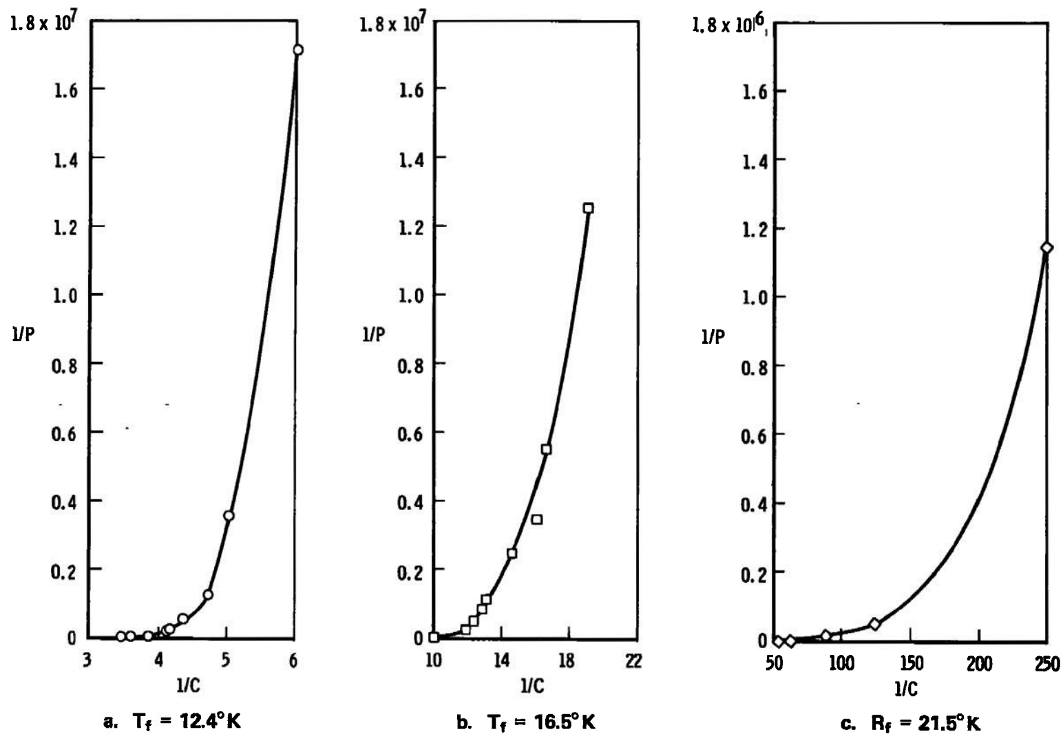
Fig. 4 Sorption Isotherms for Carbon Dioxide Frost Formed at a Pressure Level of 2 \times 10^{-5} torr Plotted in Langmuir Coordinates
