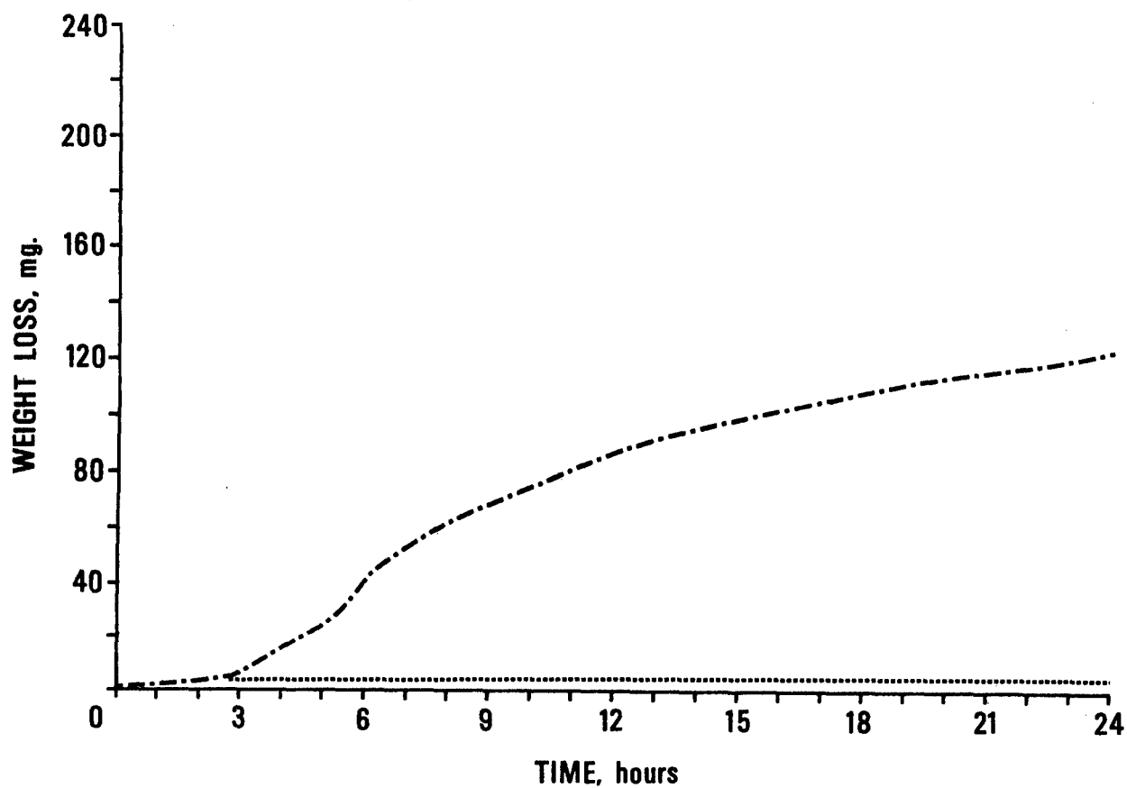
Figure 34. TGA (Upper) and Water Loss (Lower) Curves of N3031A (Lubeco, Inc.) (AF 712).
