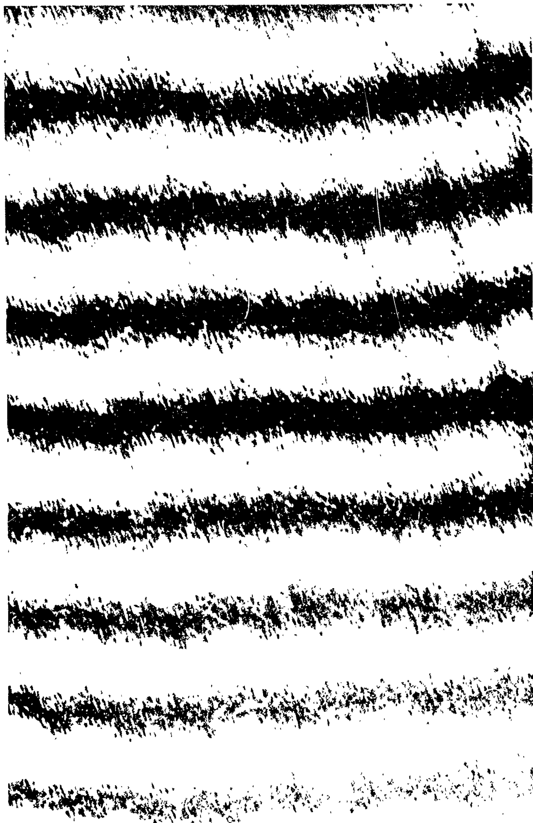
Figure 2 - Interference pattern from two V-shaped grooves. The grooves are approximately 4 \times 10^{-5} inch deep and are 0.005 inch apart. The groove angle is 110^\circ and the ratio of groove side to distance between grooves is approximately 100. The wavelength of the light is 6328\text{\AA} .
