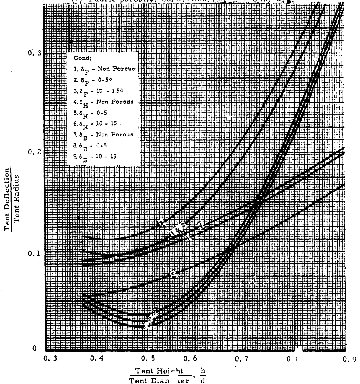
Figure 51. Variation of Tent Deflection with Shape and Fabric Porosity (Cylindrical Single-Wall Tents, 1:2 W/H)
