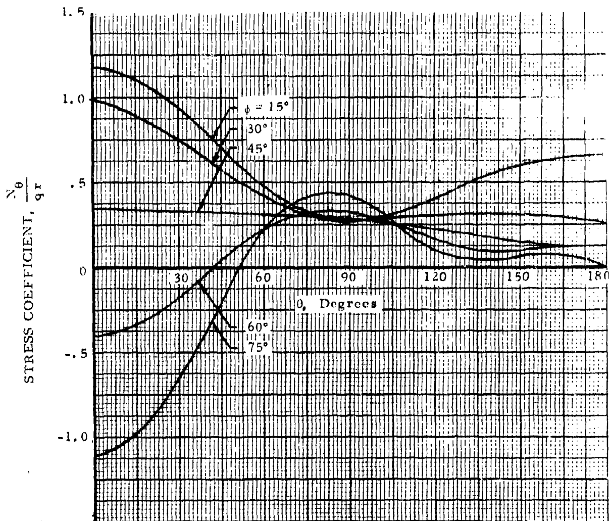
Figure 85. Typical Calculated Stress Coefficients, \frac{N_{\theta}}{qr} ; Spherical Ends, h/d = 3/8 , P_e = 4/5q , q = .6
