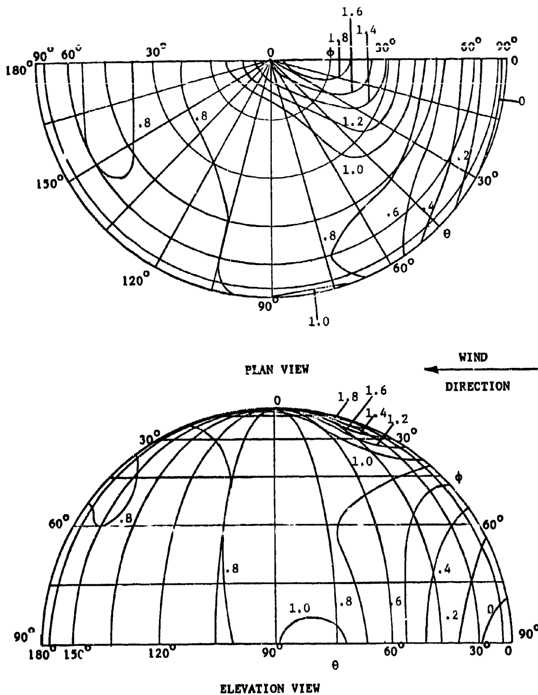
Figure 116. N_\theta/q_r for Spherical Tent ( h/d = 1/2 )
