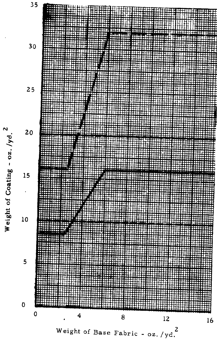
Figure 174. Weight of Coating For Single-And Two-Ply Coated Fabric
