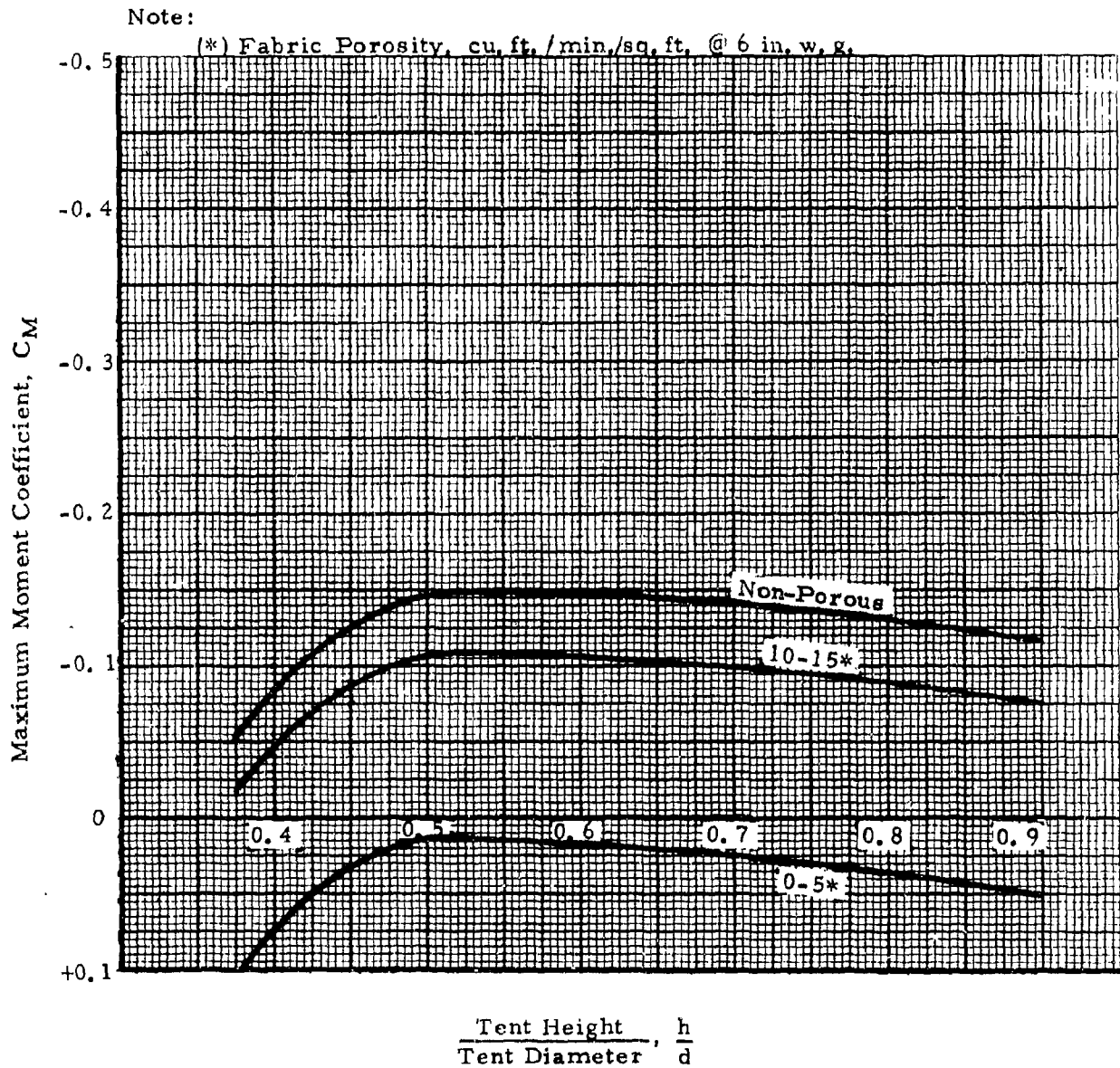
Figure 35. Variation of Moment Coefficient with Shape and Fabric Porosity (Spherical Single-Wall Tents)
