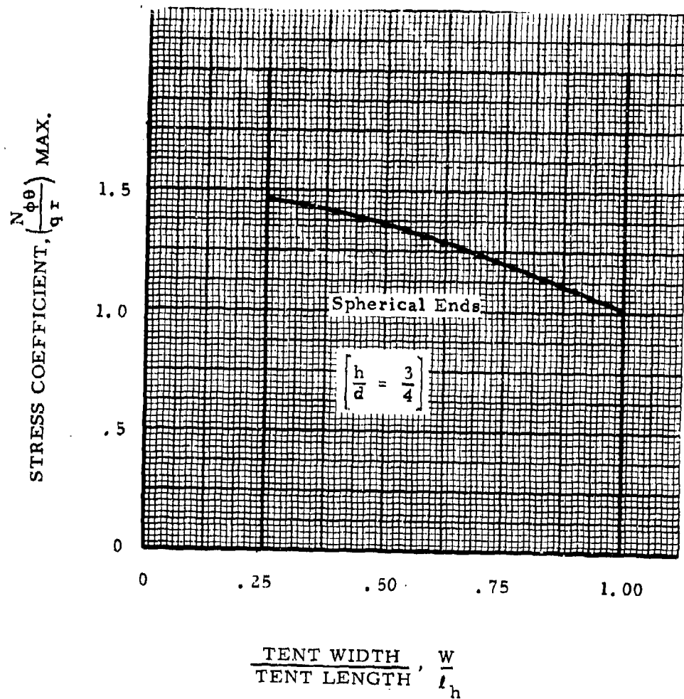
Figure 105. Maximum Design Stress Coefficient, \frac{N_{\phi\theta}}{q_r} , Dynamic Pressure Limit ( q = 6.0 ) Constant h/d = W/l_h Range ( W/l_h = .25 to 1.00 ), h/d = 3/4
