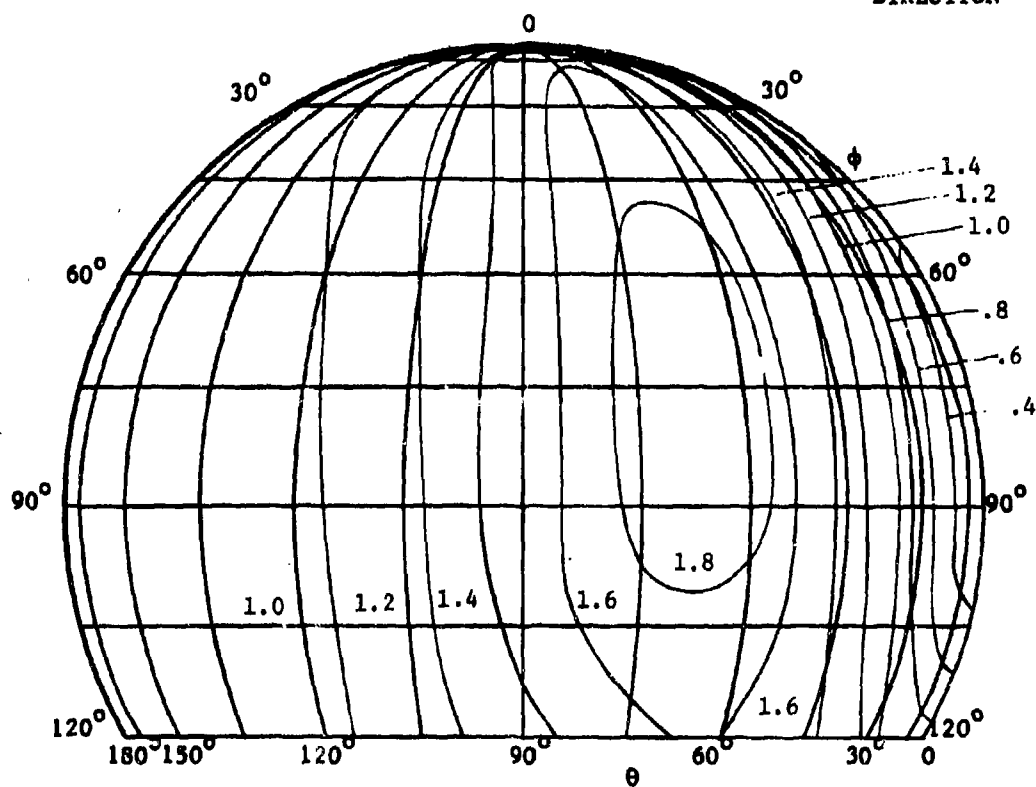
ELEVATION VIEW
