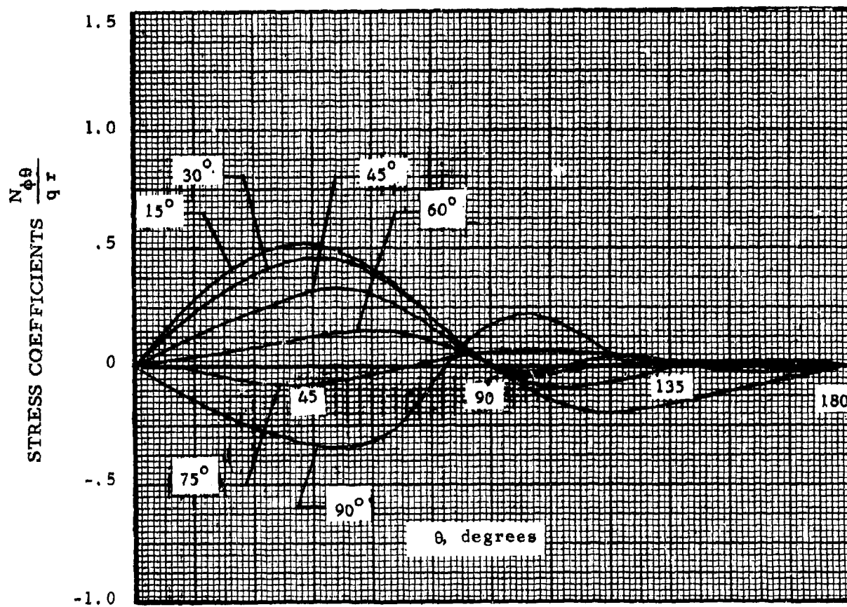
Figure 73. Typical Stress Coefficients, \frac{N_{\phi\theta}}{qr} ; Single-Wall Spheres, h/d = 1/2
