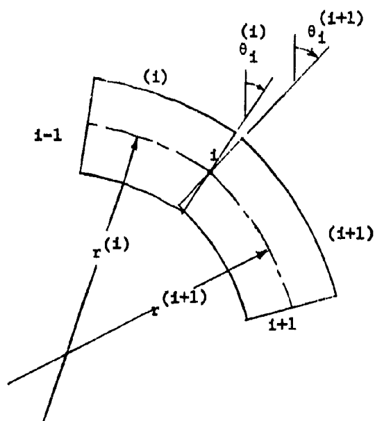
Figure 149. Mismatch of Finite Elements
