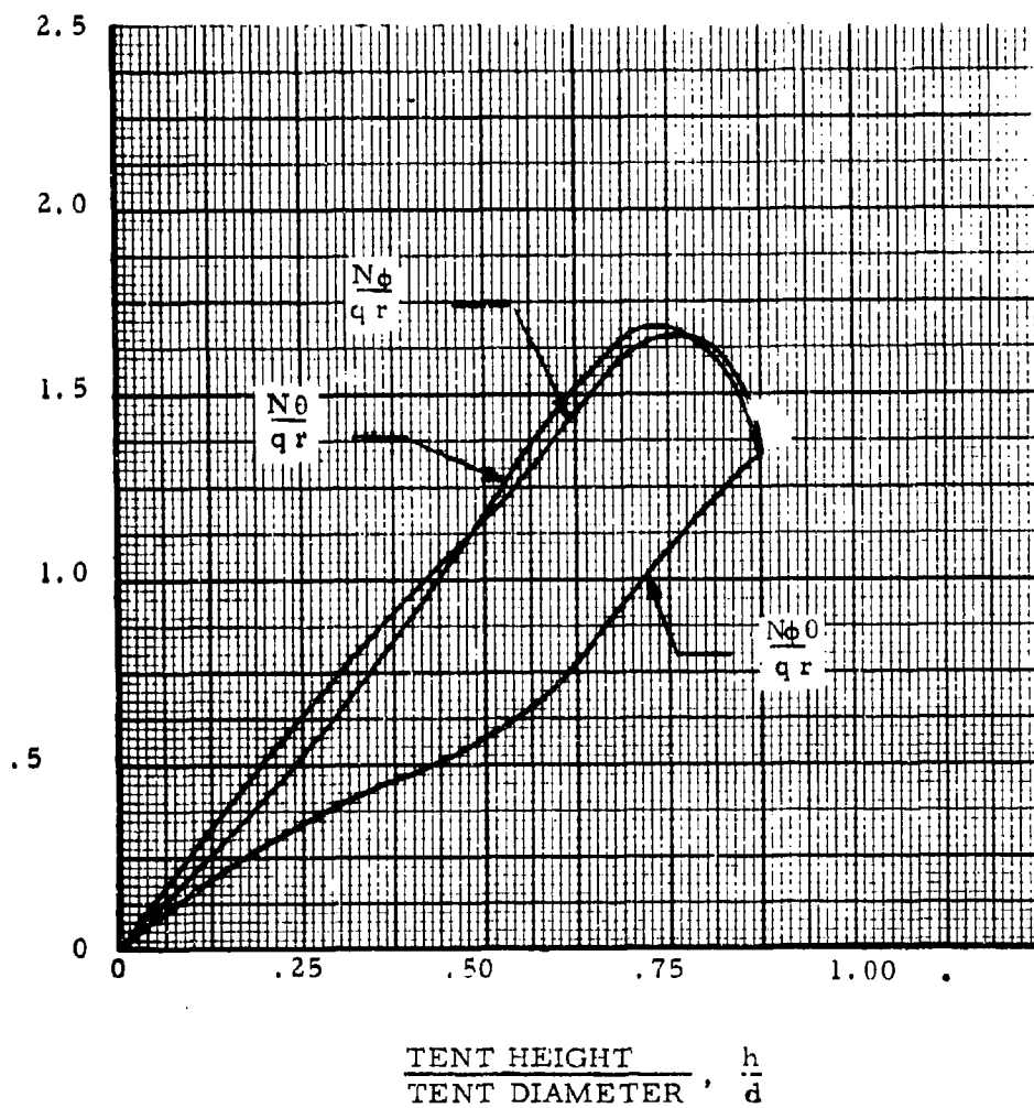
Figure 78. Variation of Peak Stress Coefficient with Shape at q = 3.0 Inches of Water Gage; Non-Porous Single-Wall Spheres
