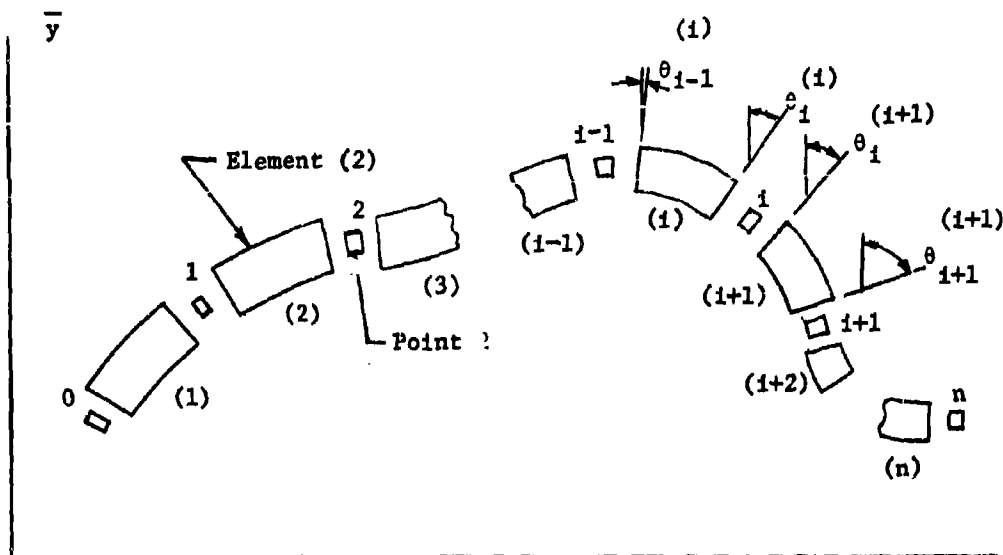
Figure 146. Finite Element Identification
