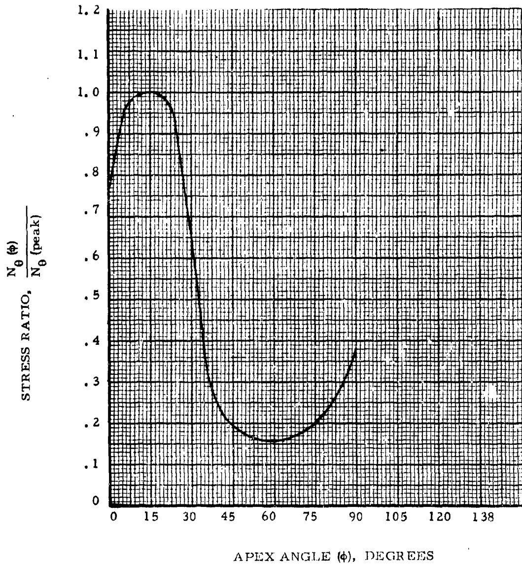
Figure 81. Stress Ratio, \frac{N_{\theta}(\phi)}{N_{\theta}(\text{peak})} Vs. Apex Angle, \phi ; Single-Wall Spheres, h/d = 1/2
