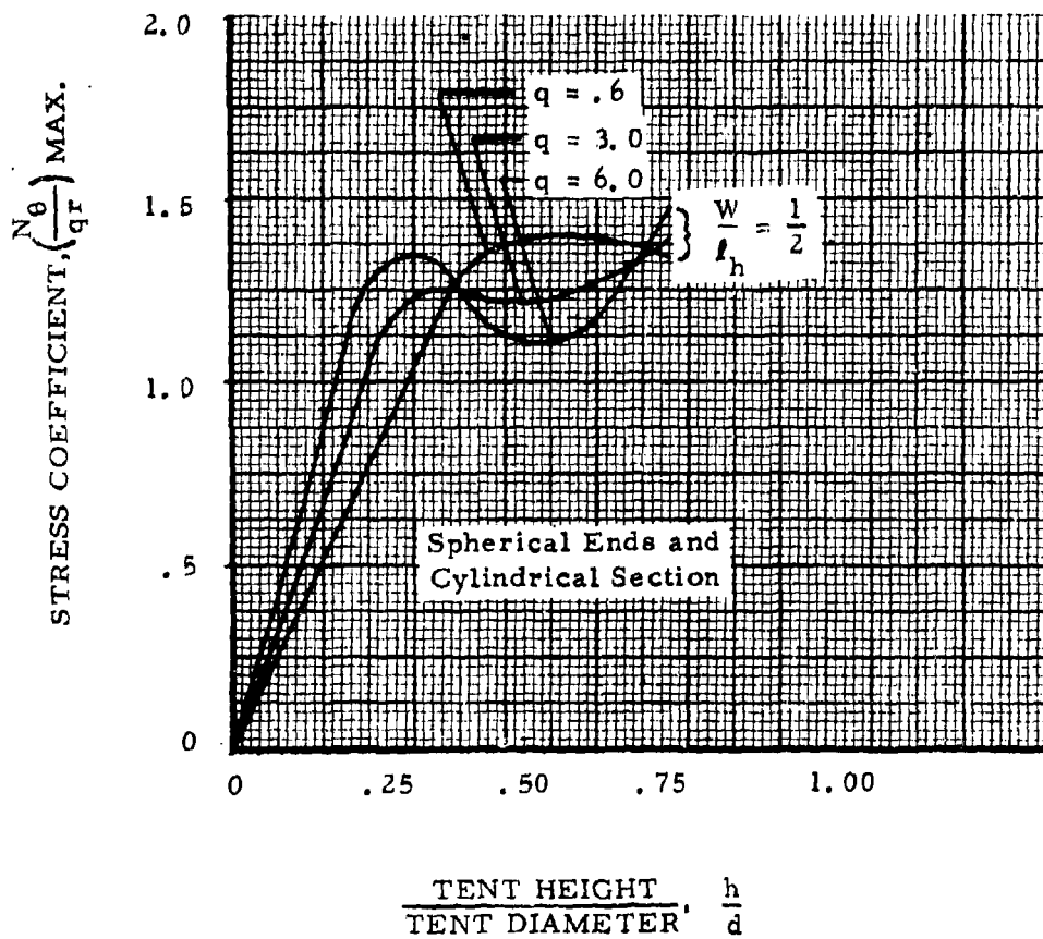
Figure 95. Maximum Design Stress Coefficient, \frac{N_{\theta}}{qr} , Specific Dynamic Pressure
