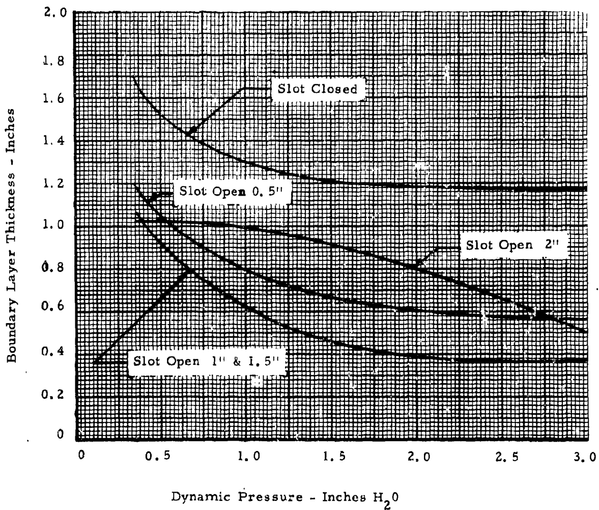
Figure 11. Boundary Layer Thickness Above the Ground Plane
