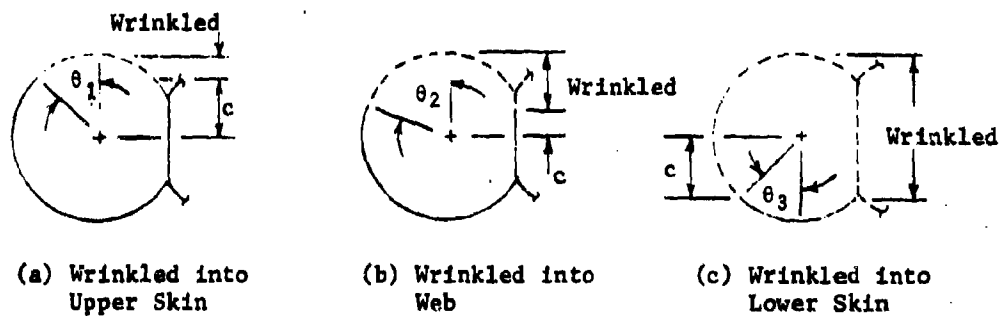
Figure 140. Stages of Wrinkling of Cellular Beams
