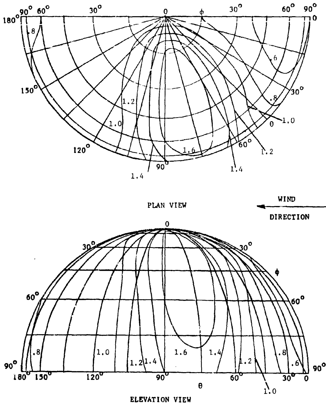
Figure 120. N_{\phi}/qr for Spherical End of Cylindrical Tent ( W/l_h = 1/2 , h/d = 1/2 )
