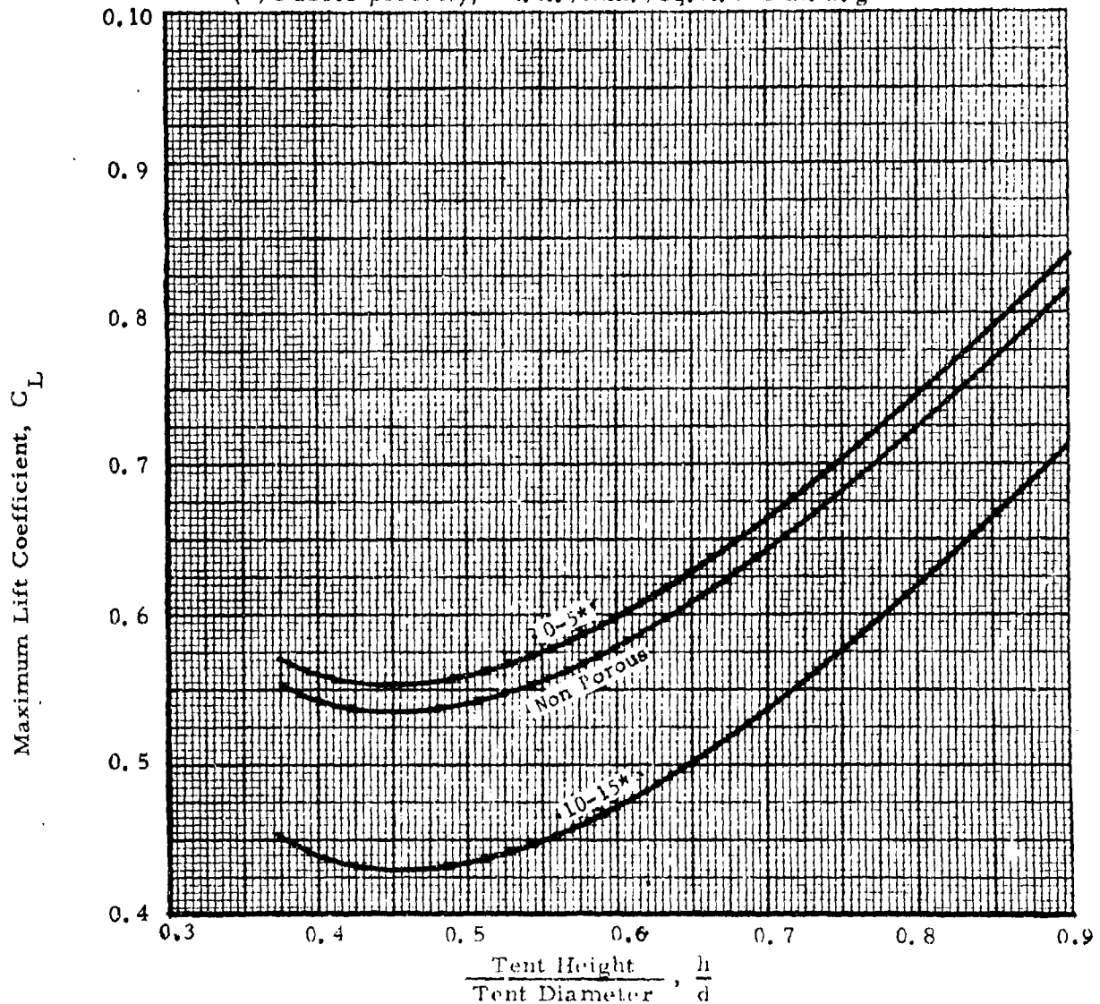
Figure 23. Variation of Lift Coefficient with Shape and Fabric Porosity (Cylindrical Single-Wall Tents; 1:2 \frac{W}{h} )
