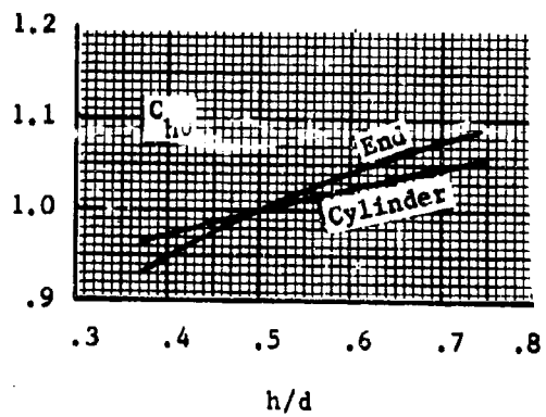
Figure 111. Correction Factors, (\theta) , for Cylindrical Tents with Ellipsoidal Ends
