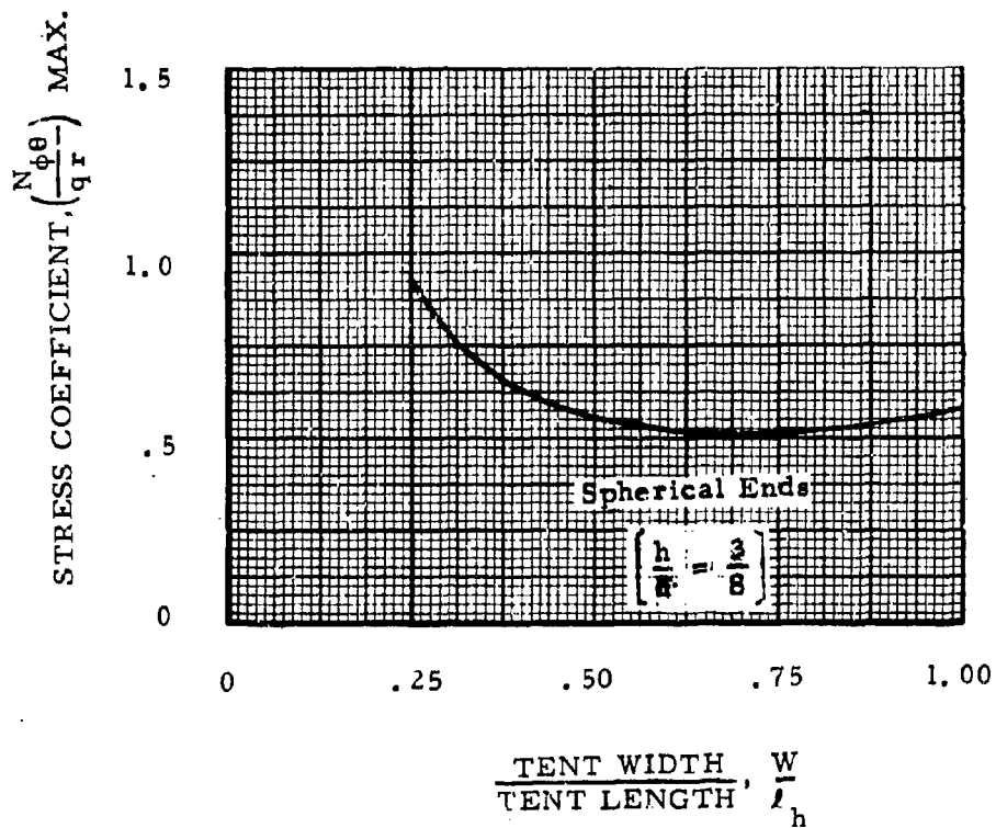
Figure 103. Maximum Design Stress Coefficient, \frac{N}{q r} \left( \frac{\phi \theta}{r} \right) , Dynamic Pressure Limit ( q = 6.0 ) Constant h/d = W/l_h Range ( W/l_h = .25 to 1.00 ), h/d = 3/8
