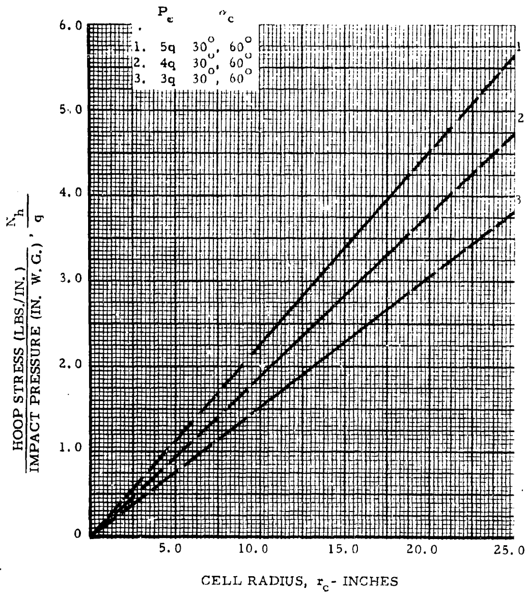
Figure 161. Variation of Ratio of Hoop Stress with Impact Pressure with Cell Radius; Double-Wall Cylinders
