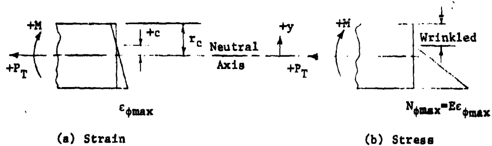
Figure 138. Stress and Strain of Cellular Beam
