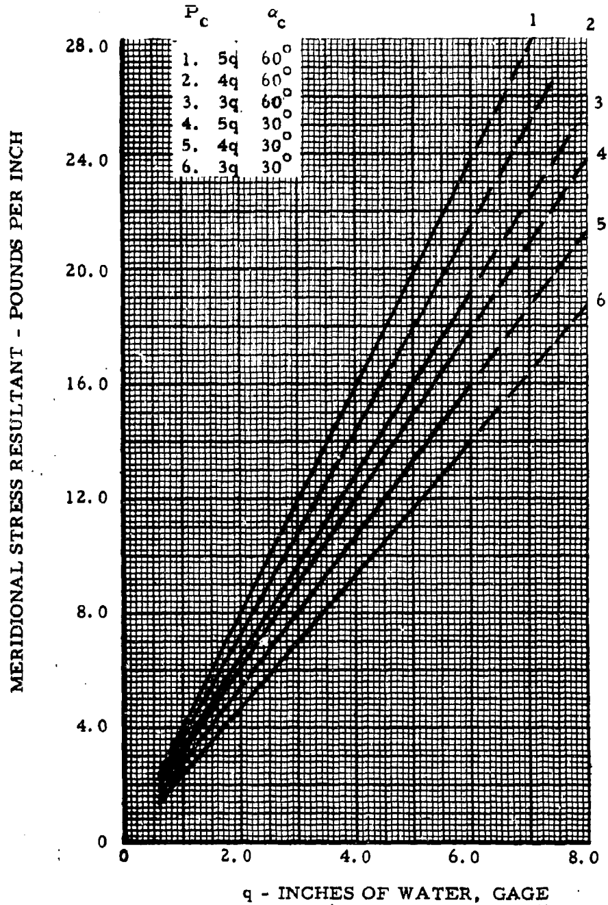
Figure 162. Variation of Meridional Stress Resultant with Impact Pressure, q ; Double-Wall Cylinders, w/d = 0.16 , h/d = .5
