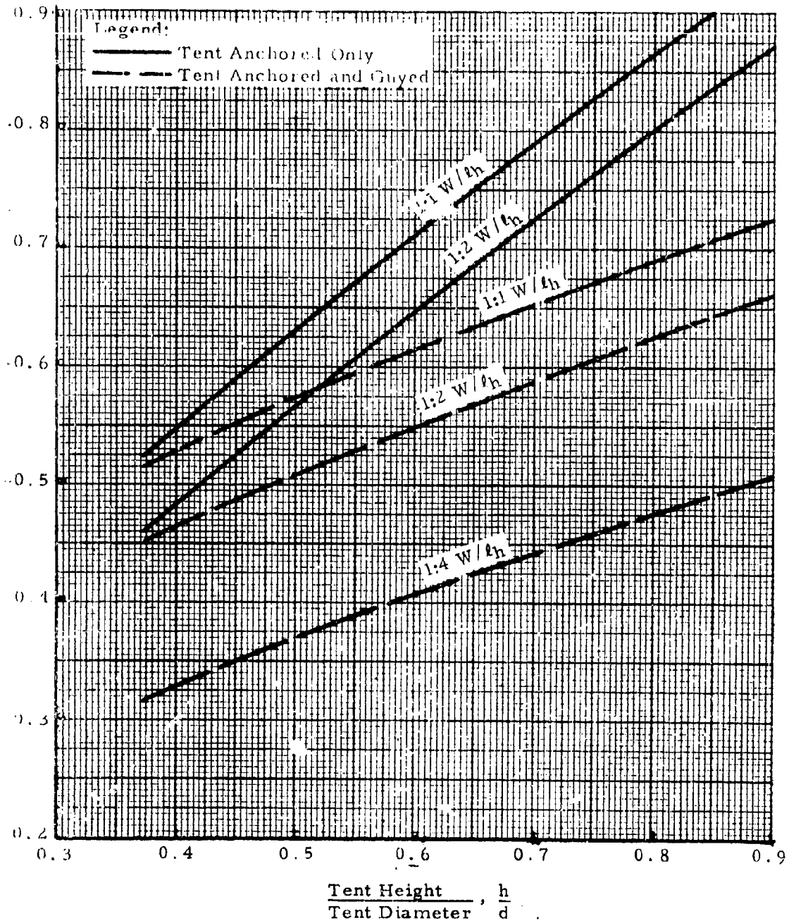
Figure 40. Variation of Moment Coefficient with Shape & Guying (Non-Porous Double-Wall Tents; 1:1, 1:2, 1:4 W/\ell_h )
