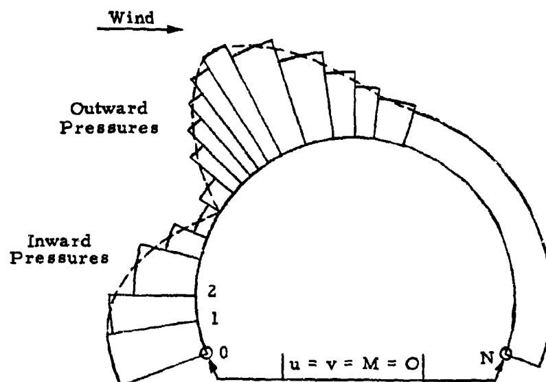
Figure 158. Loads and Boundary Conditions
