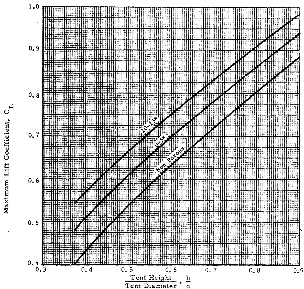
Figure 22. Variation of Lift Coefficient with Shape and Fabric Porosity (Spherical Single-Wall Tents)
