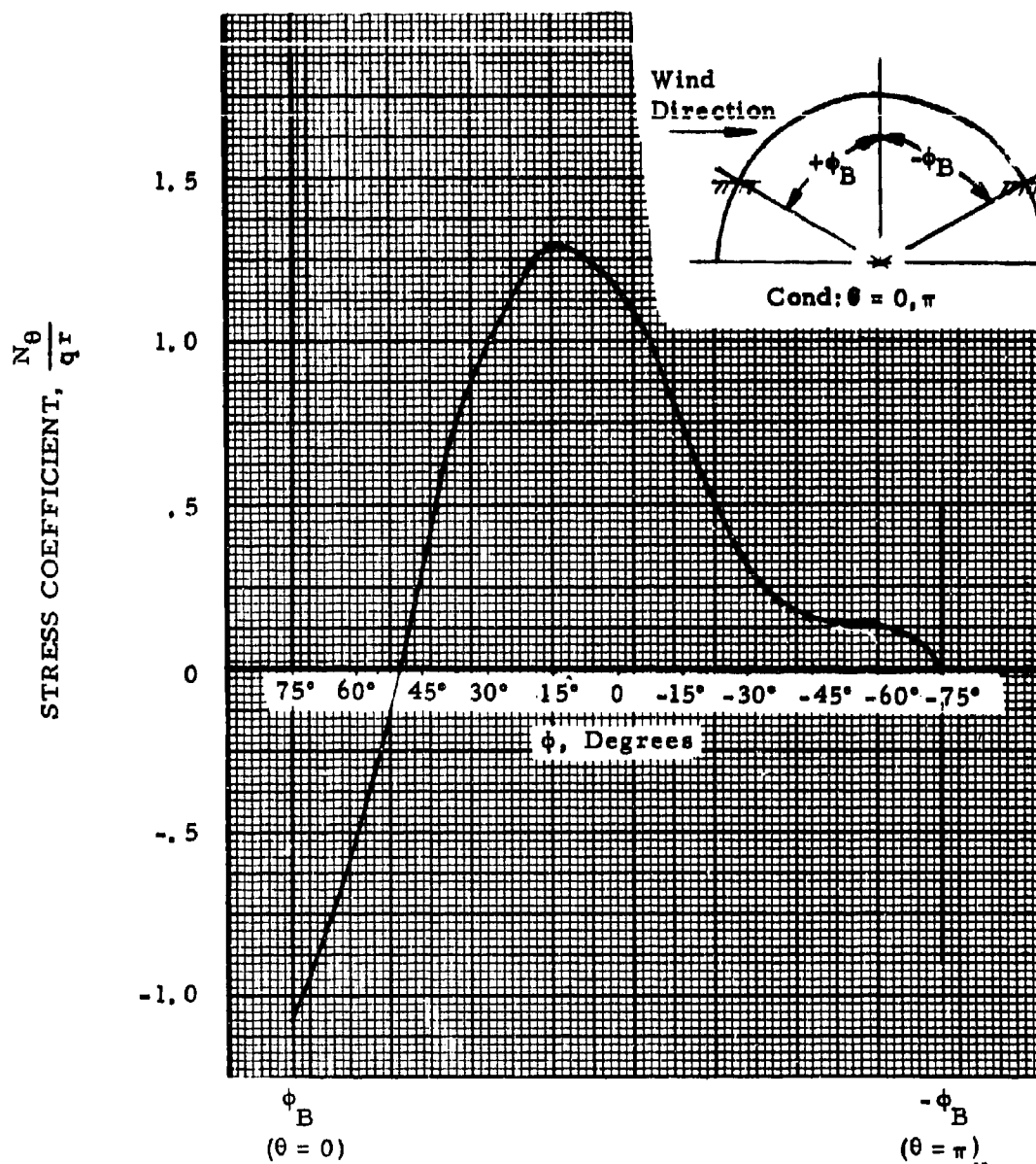
Figure 93. Typical Maximum Peripheral Stress Coefficient, \frac{N_\theta}{qr} , Distribution; Cylindrical - Spherical End Junction, W/l_h = 1/2 , h/d = 3/8
