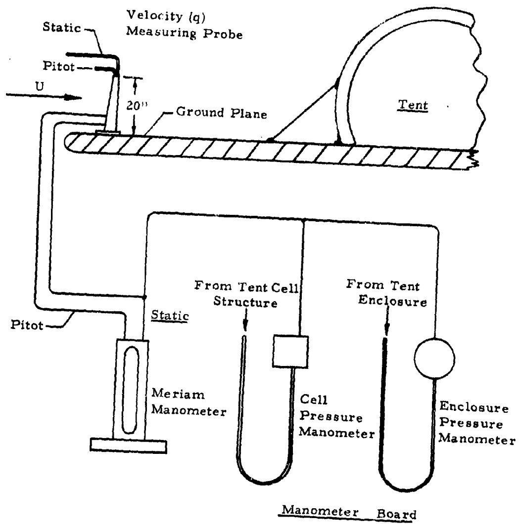
Figure 3. Pressure Instrumentation Schematic
