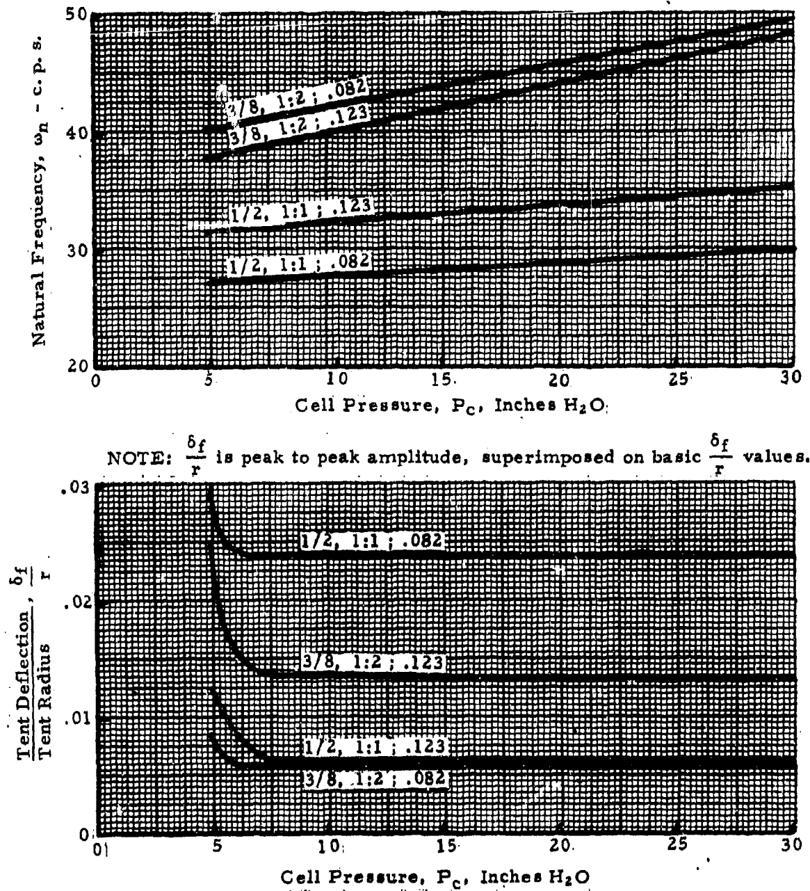
Figure 59. Tent Frequency and Amplitude of Vibration, Without Guy Lines Installed
