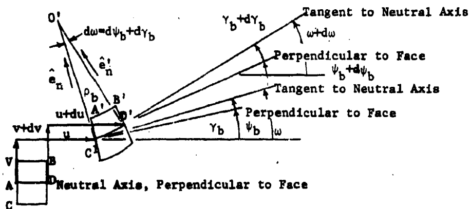
Figure 141. Nonlinear Load-Strain Relations
