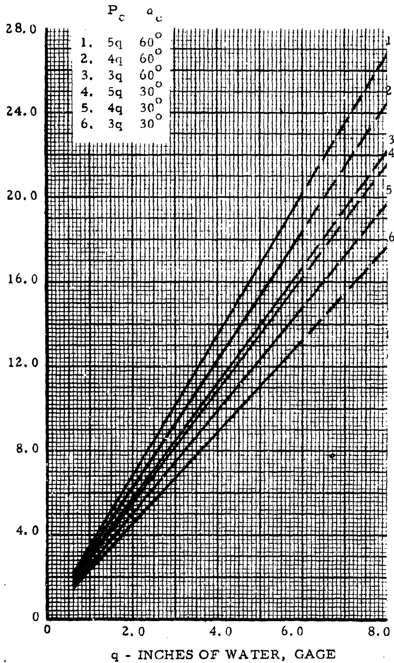
Figure 163. Variation of Meridional Stress Resultant with Impact Pressure, q ; Double-Wall Cylinders, w/d = 0.12 , h/d = .5
