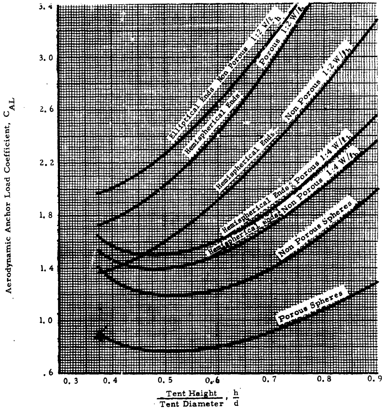
Figure 45. Variation of Anchor Load Coefficient With Shape, Single-Wall Tents
