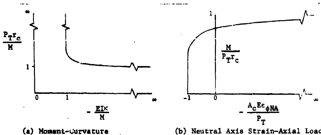
Figure 141. Nonlinear Load-Strain Relations
