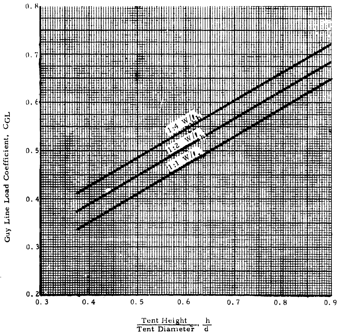
Figure 48 . Variation of Guy Line Load Coefficient With Shape
