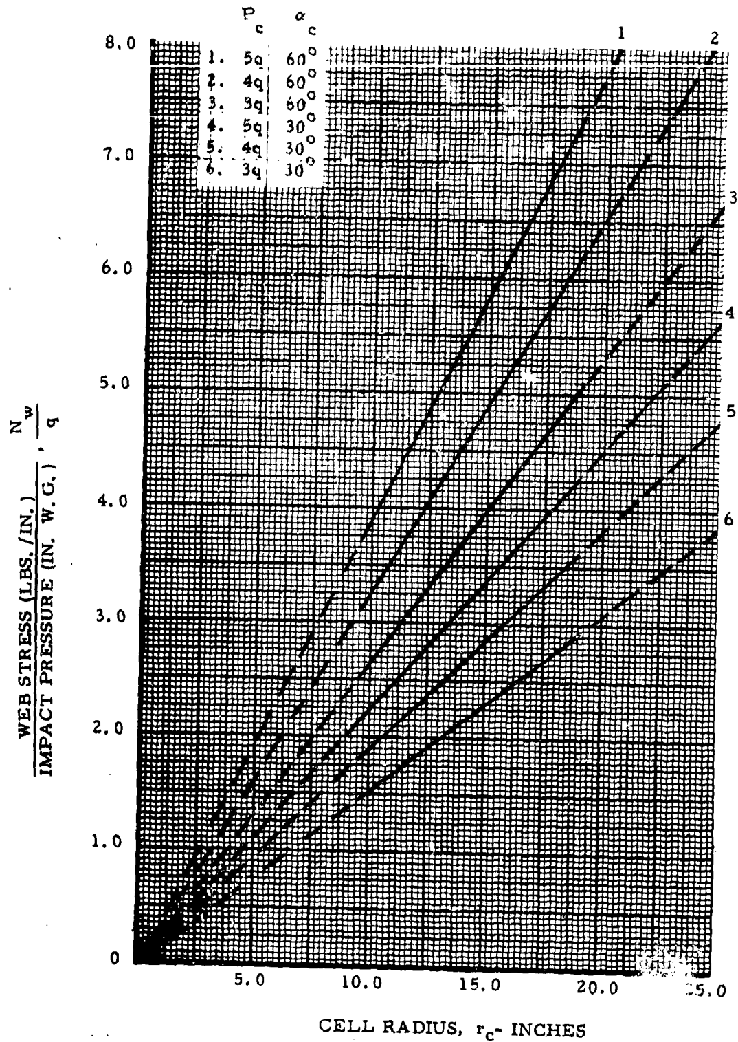
Figure 160. Variation of Ratio of Web Stress to Impact Pressure with Cell Radius; Double-Wall Cylinders
