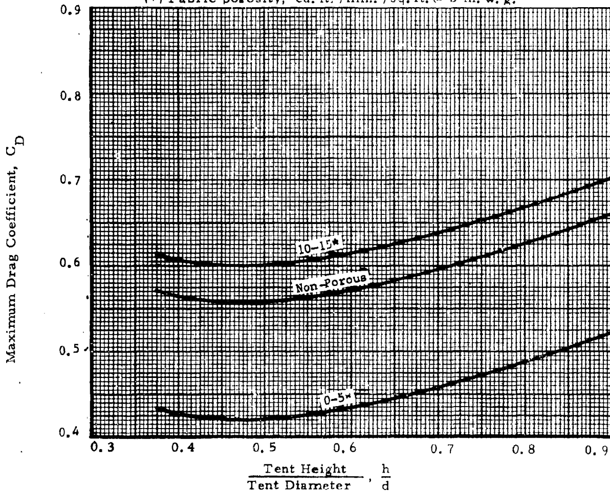
Figure 30. Variation of Drag Coefficient with Shape and Fabric Porosity (Cylindrical Single-Wall Tents, 1:4 \frac{W}{h} )
