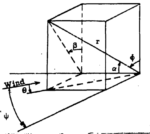
(c) Conversion from \alpha, \beta to \phi, \theta Coordinates
