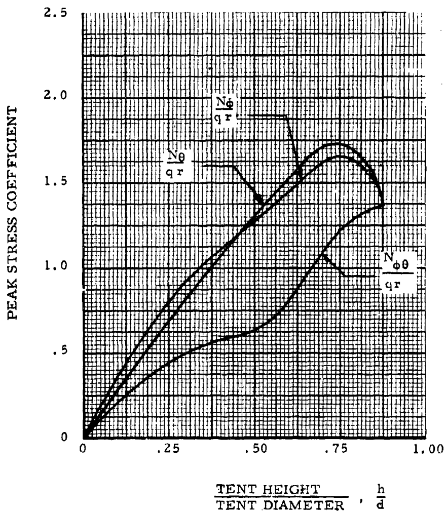
Figure 79. Variation of Peak Stress Coefficients with Shape at q = 6.0 Inches of Water Gage; Non-Porous Single-Wall Spheres
