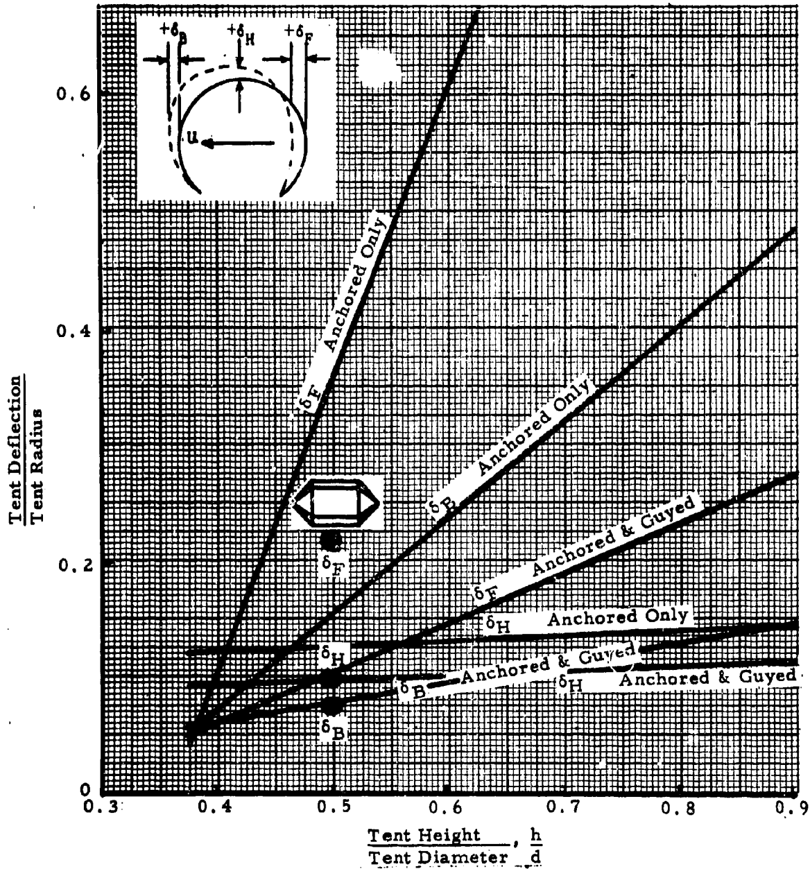
Figure 58. Variation of Tent Deflection with Shape (Non-Porous Double Wall Tents; 1:2 W/l h )
