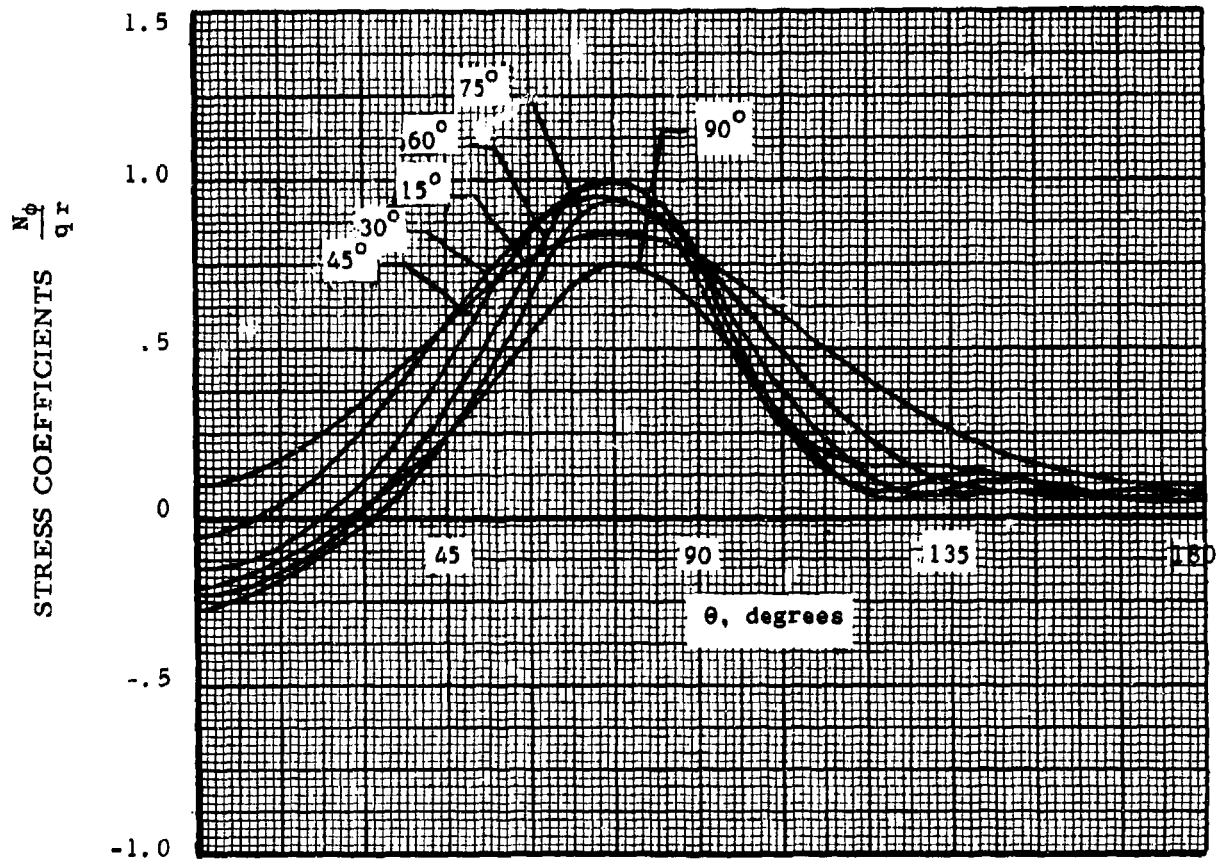
Figure 71. Typical Stress Coefficients, \frac{N_\phi}{q_r} ; Single-Wall Spheres, h/d = 1/2
