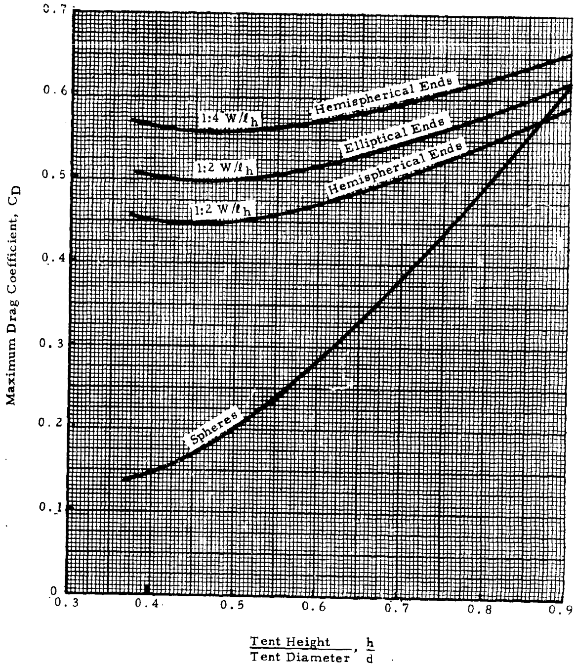
Figure 31. Variation of Drag Coefficient With Shape (Spherical and Cylindrical Single-Wall Tents; 1:2, 1:4 W/l_h )
