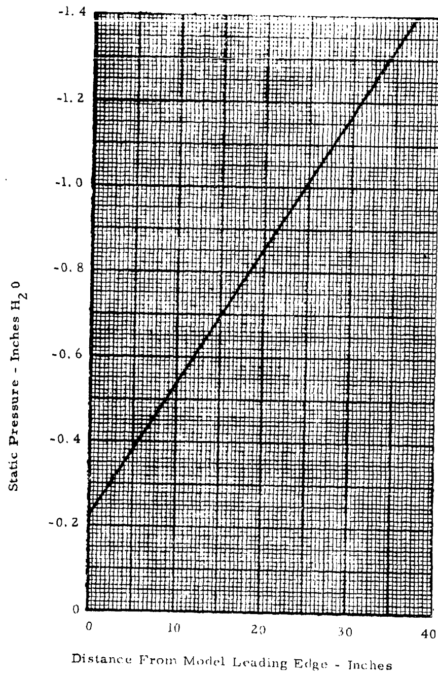
Figure 21. Wind Tunnel Static Pressure Gradient
