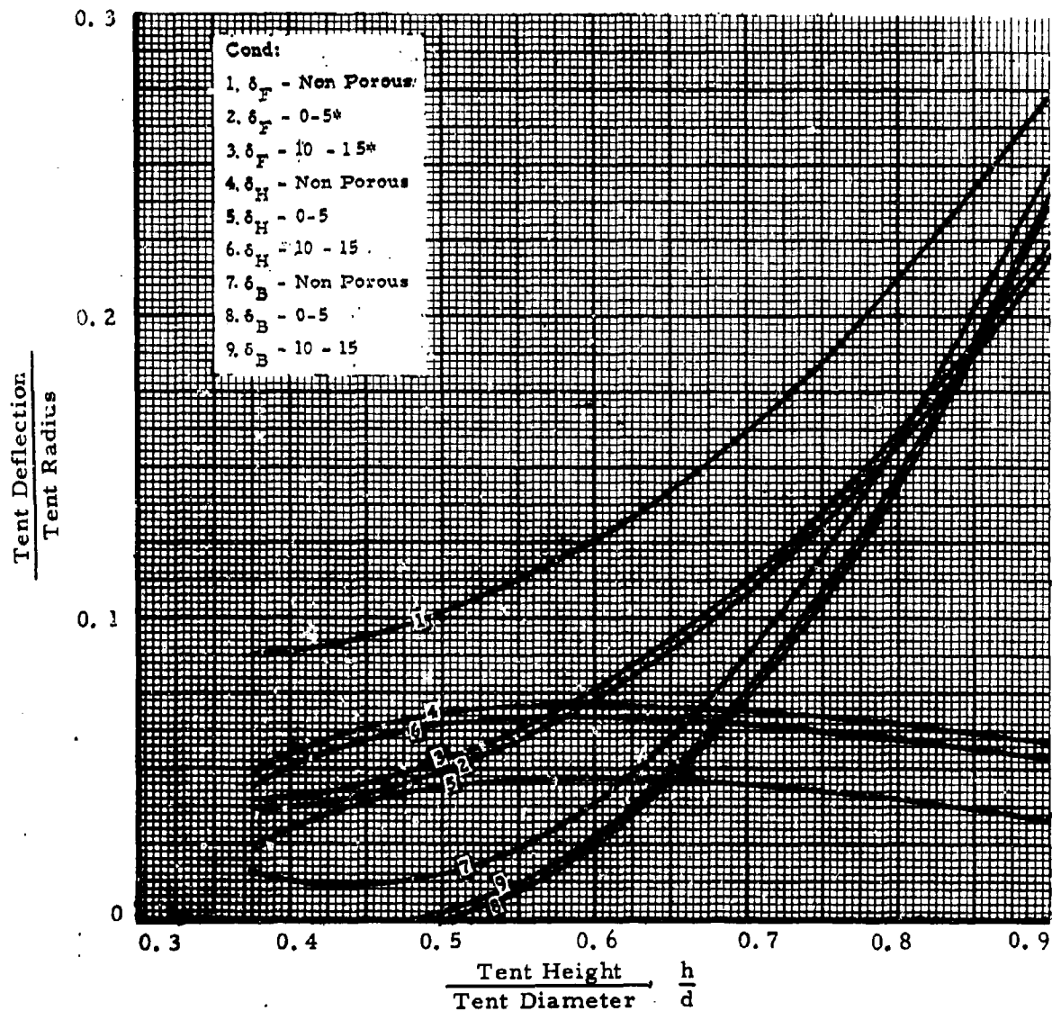
Figure 50. Variation of Tent Deflection with Shape and Fabric Porosity (Spherical Single-Wall Tents)
