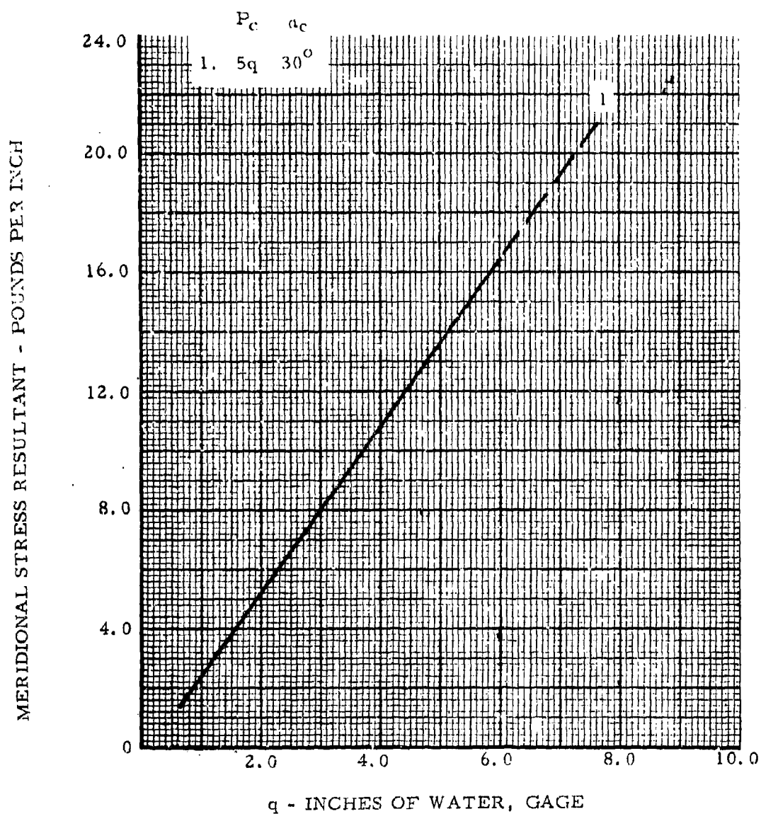
Figure 167. Variation of Meridional Stress Resultant with Impact Pressure, q ; Double-Wall Cylinders, w/d = 0.08 , 9^\circ Sloping Sides, h/d = 0.8
