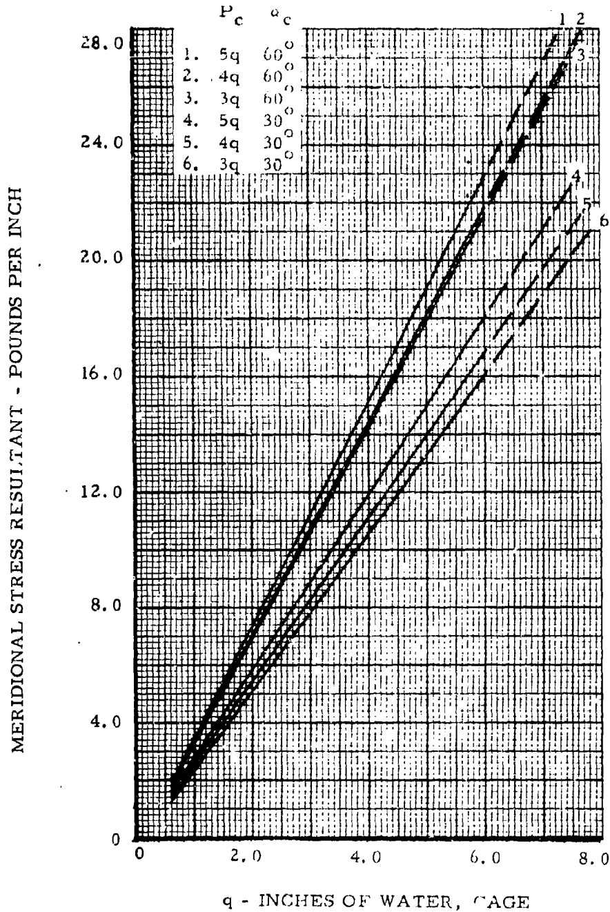
Figure 169. Variation of Meridional Stress Resultant with Impact Pressure, q ; Double-Wall Cylinders, w/d = 0.12 , h/d = 0.75
