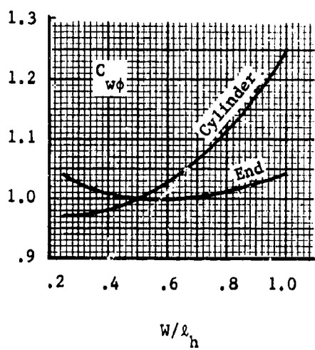
Figure 110. Correction Factors, (\phi) , for Cylindrical Tents with Ellipsoidal Ends
