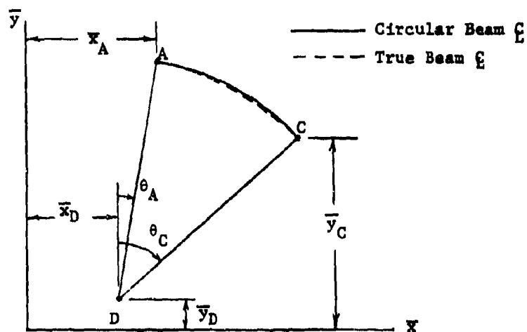
Figure 152. Beam Element Geometry
