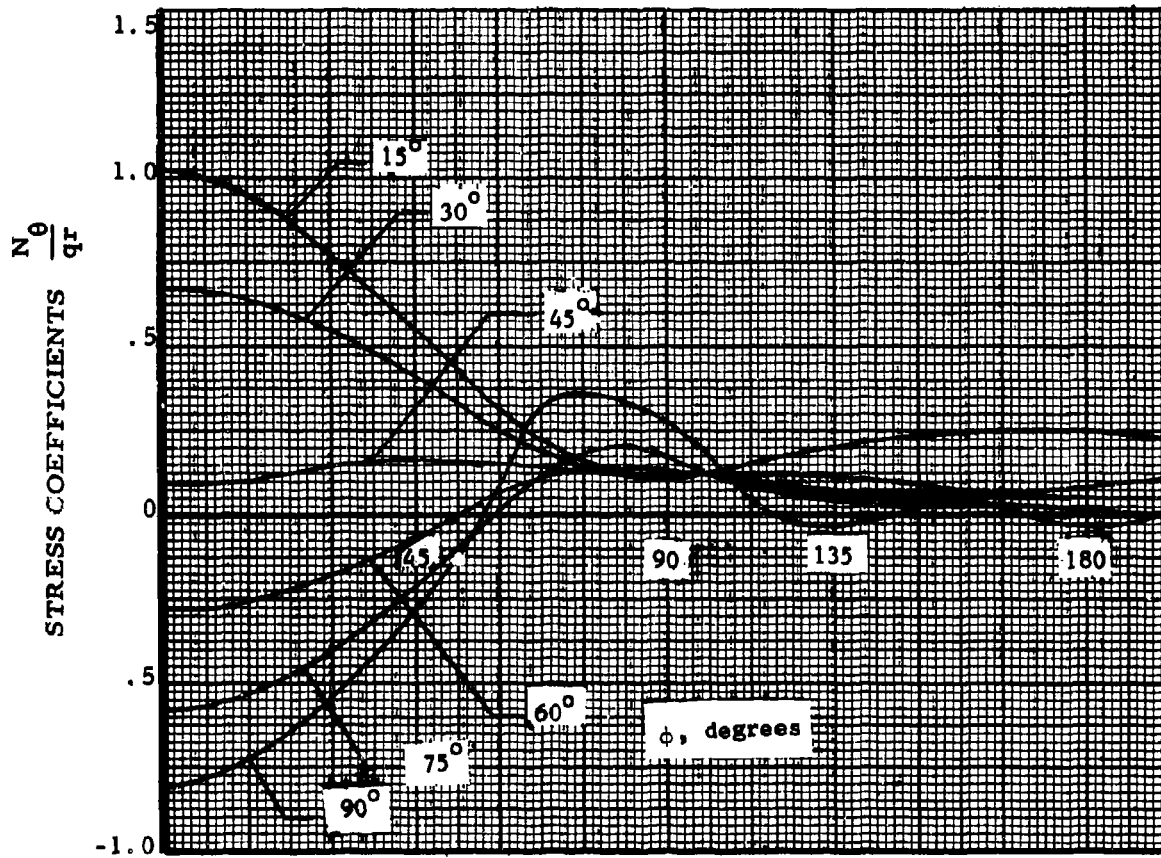
Figure 72. Typical Stress Coefficients, \frac{N_{\theta}}{q_r} ; Single-Wall Spheres, h/d = 1/2
