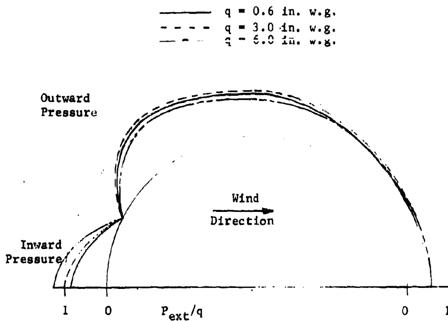
Figure 136. Pressure Distribution on Unguyed Double-Wall Tents ( h/d = 1/2 , W/\ell_h = 1/2 )
