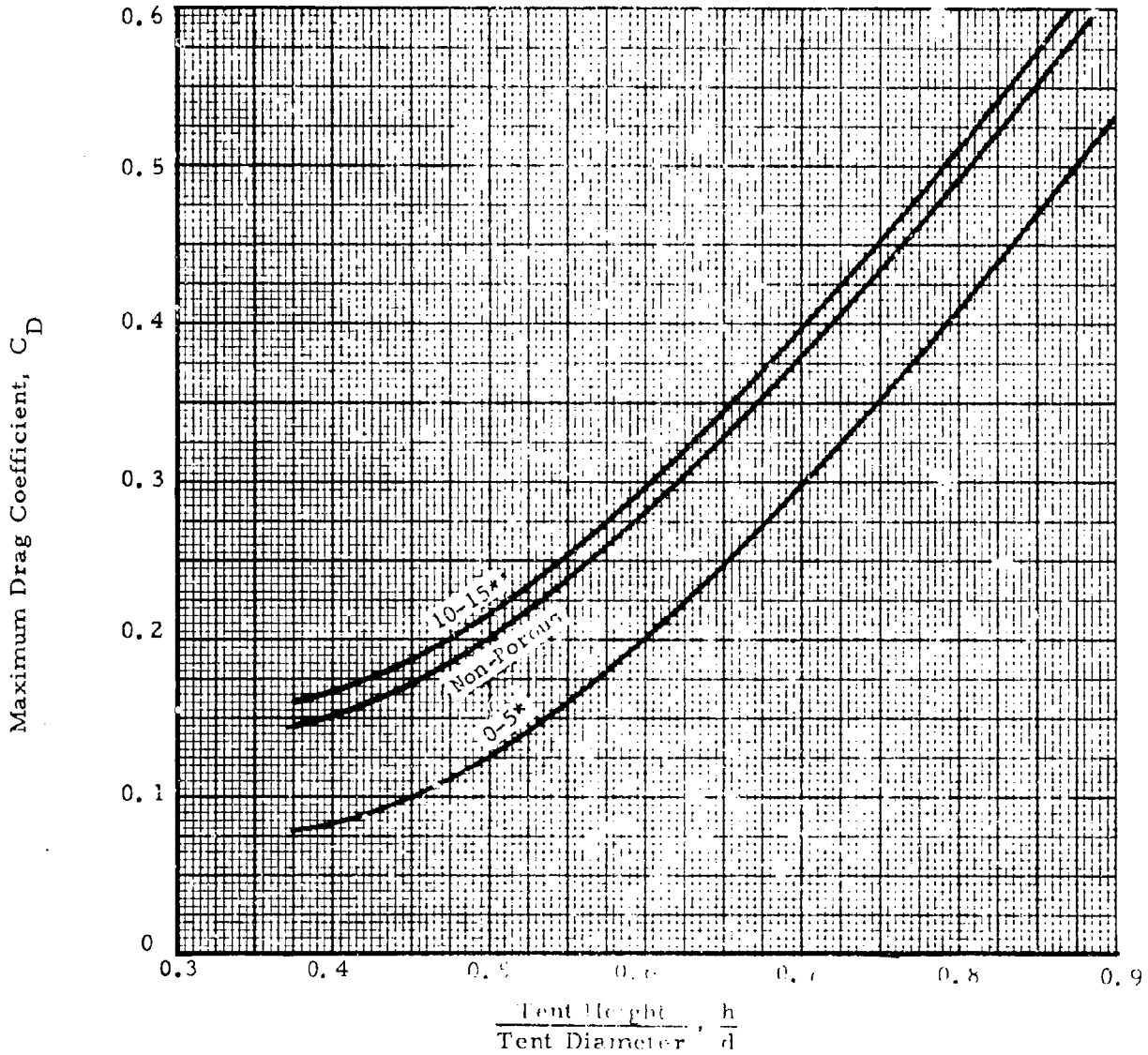
Figure 28. Variation of Drag Coefficient with Shape and Fabric Porosity (Spherical Single-Wall Tents)
