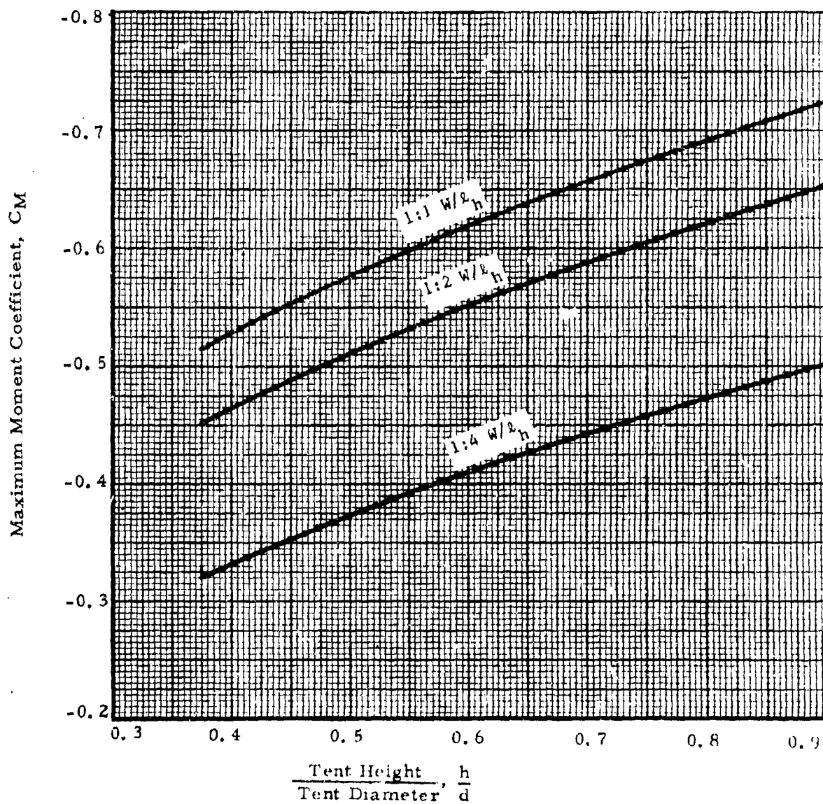
Figure 39. Variation of Moment Coefficient with Shape (Non-Porous Double-Wall Tents; 1:1, 1:2, 1:4, W/2h )
