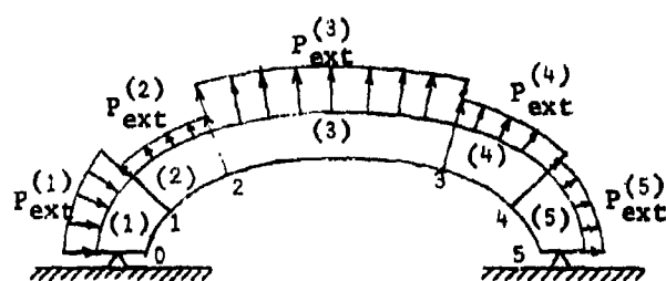
Figure 151. Five Element Beam
