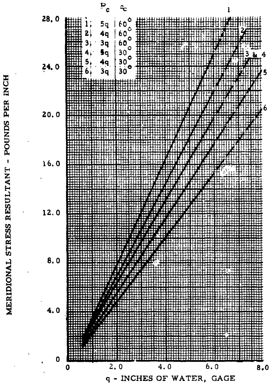
Figure 165. Variation of Meridional Stress Resultant with Impact Pressure, q ; Double-Wall Cylinders, w/d = 0.16 , 90^\circ Sloping Sides, h/d = 0.8
