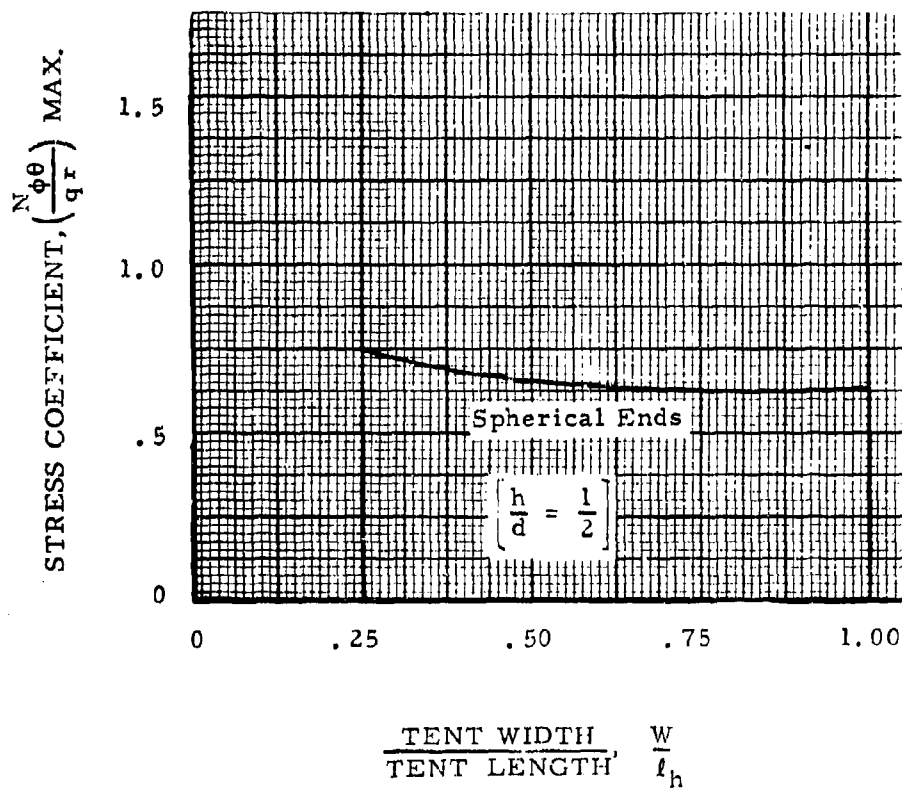
Figure 104. Maximum Design Stress Coefficient, \frac{N_{\phi\theta}}{qr} , Dynamic Pressure Limit ( q = 6.0 ) Constant h/d = W/l_h Range ( W/l_h = .25 to 1.00 ), h/d = 1/2
