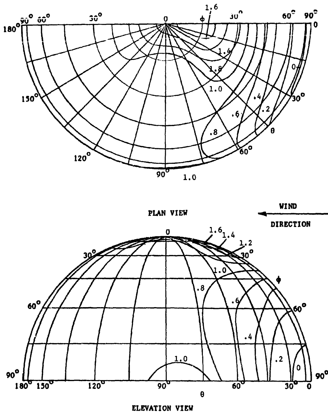
Figure 121. N_\theta/q_r for Spherical End of Cylindrical Tent ( W/l_h = 1/2 , h/d = 1/2 )
