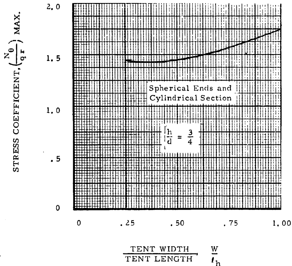
Figure 102. Maximum Design Stress Coefficient, \frac{N_e}{q r} , Dynamic Pressure Limit ( q = 6.0 ) Constant h/d = W/l_h Range ( W/l_h = .25 to 1.00), h/d = 3/4
