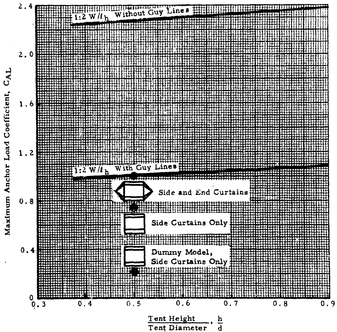
Figure 47. Variation of Base Anchor Load Coefficient with Shape, Double-Wall Tents
