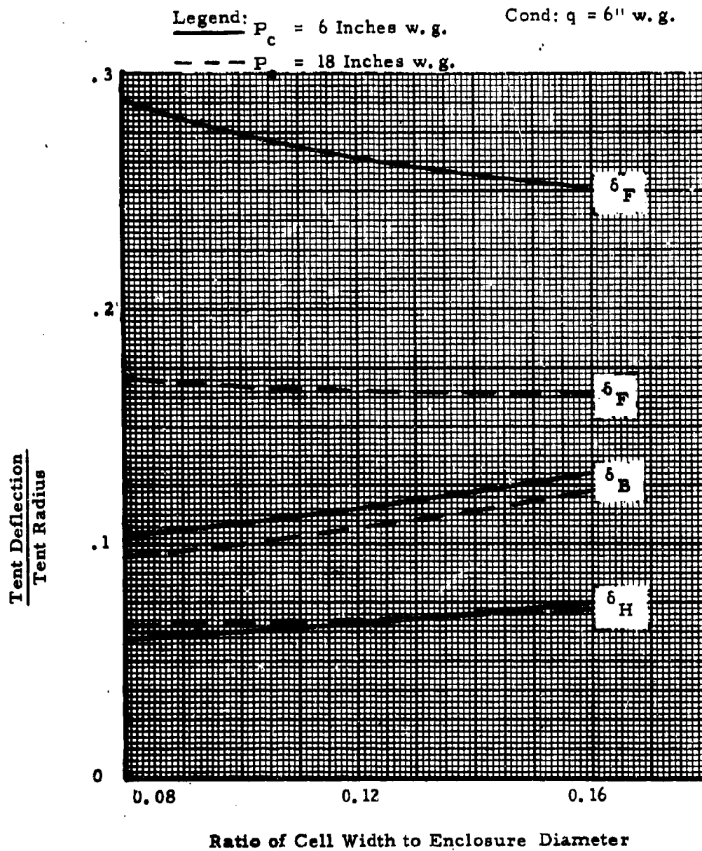
Figure 54. Effect of Cell Size on Tent Deflection
