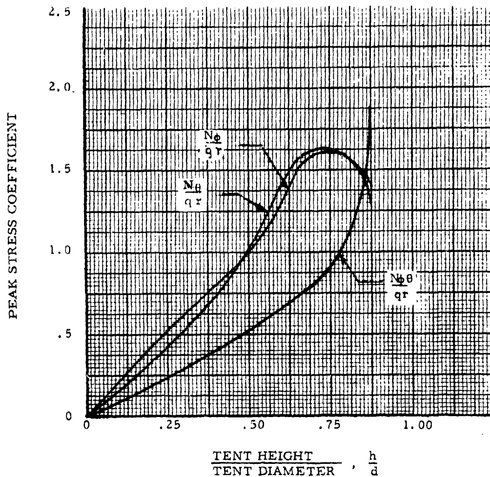
Figure 77. Variation of Peak Stress Coefficient with Shape at q = 0.6 Inches of Water Gage; Non Porous Single-Wall Spheres
