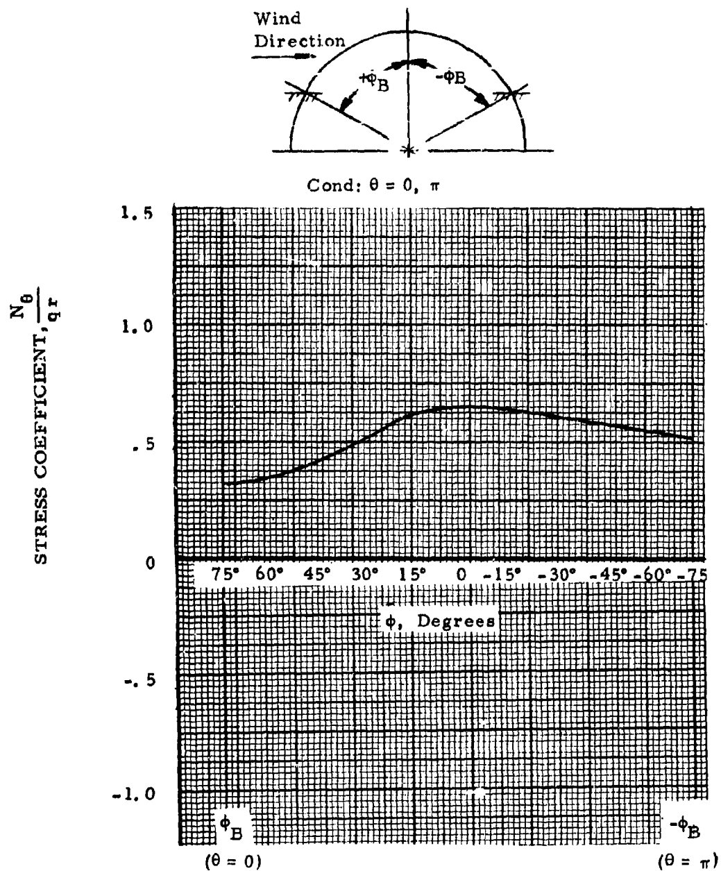
Figure 92. Typical Maximum Peripheral Stress Coefficient, \frac{N_{\theta}}{q \cdot r} , Distribution; Cylindrical - Spherical End Junction, W/l_h = 1/2 , h/d = 3/8
