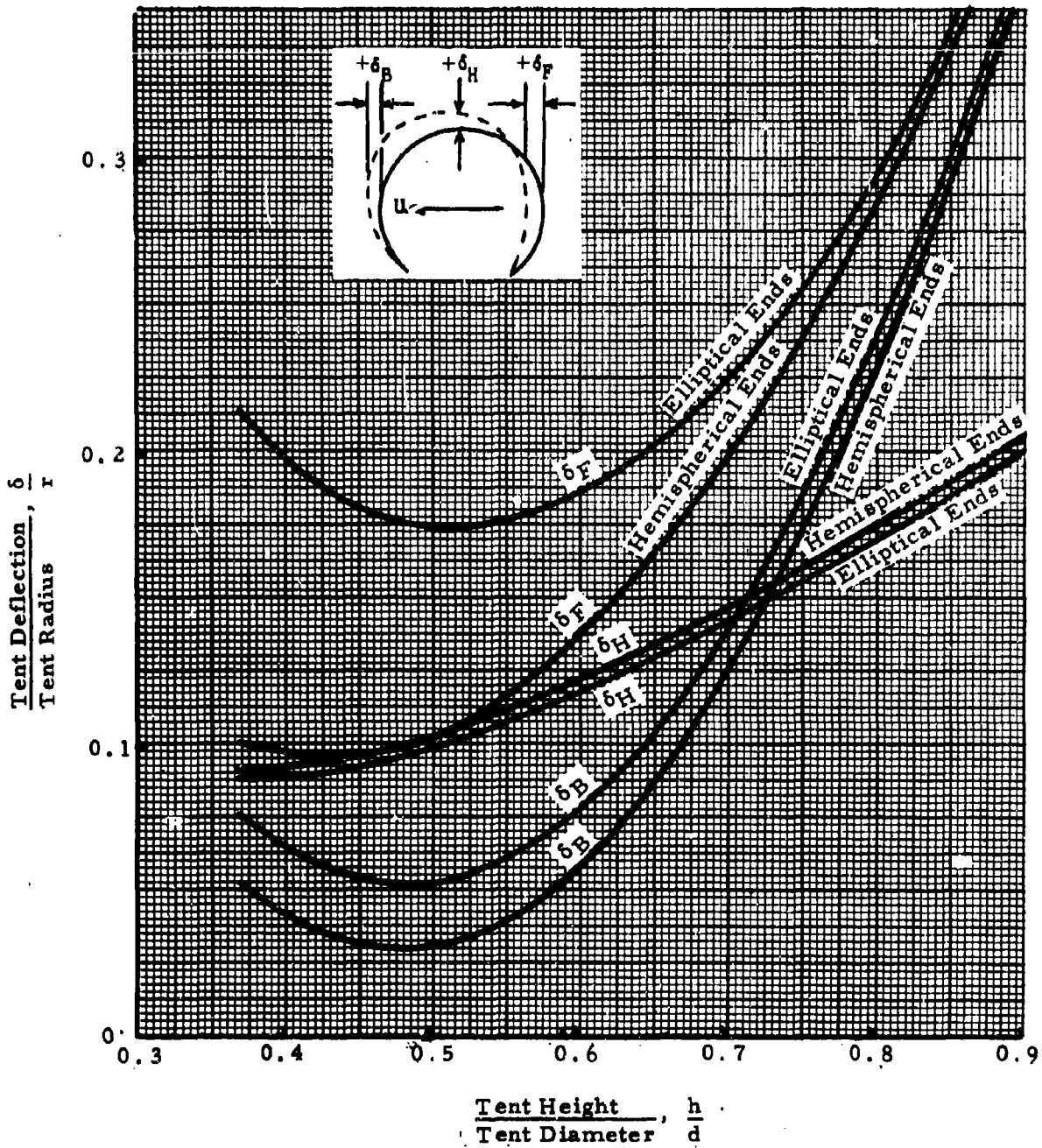
Figure 52. Comparison of Non-Porous Tent Deflection with Shape (Cylindrical Single-Wall Tents, 1:2 W/ \lambda_h )
