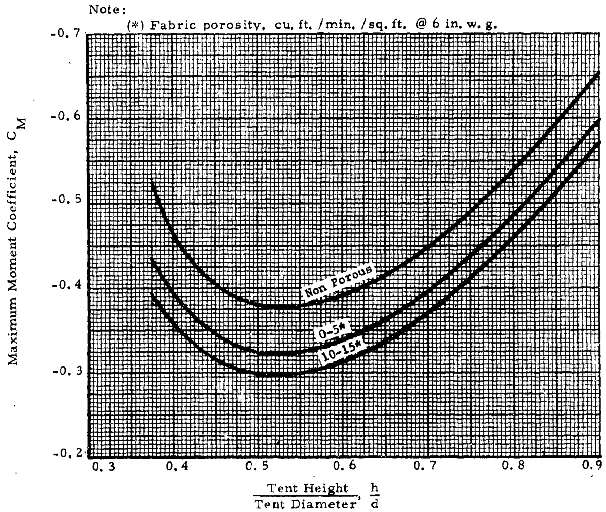
Figure 37. Variation of Moment Coefficient with Shape and Fabric Porosity (Cylindrical Single-Wall Tents, 1:4 \frac{W}{h} )
