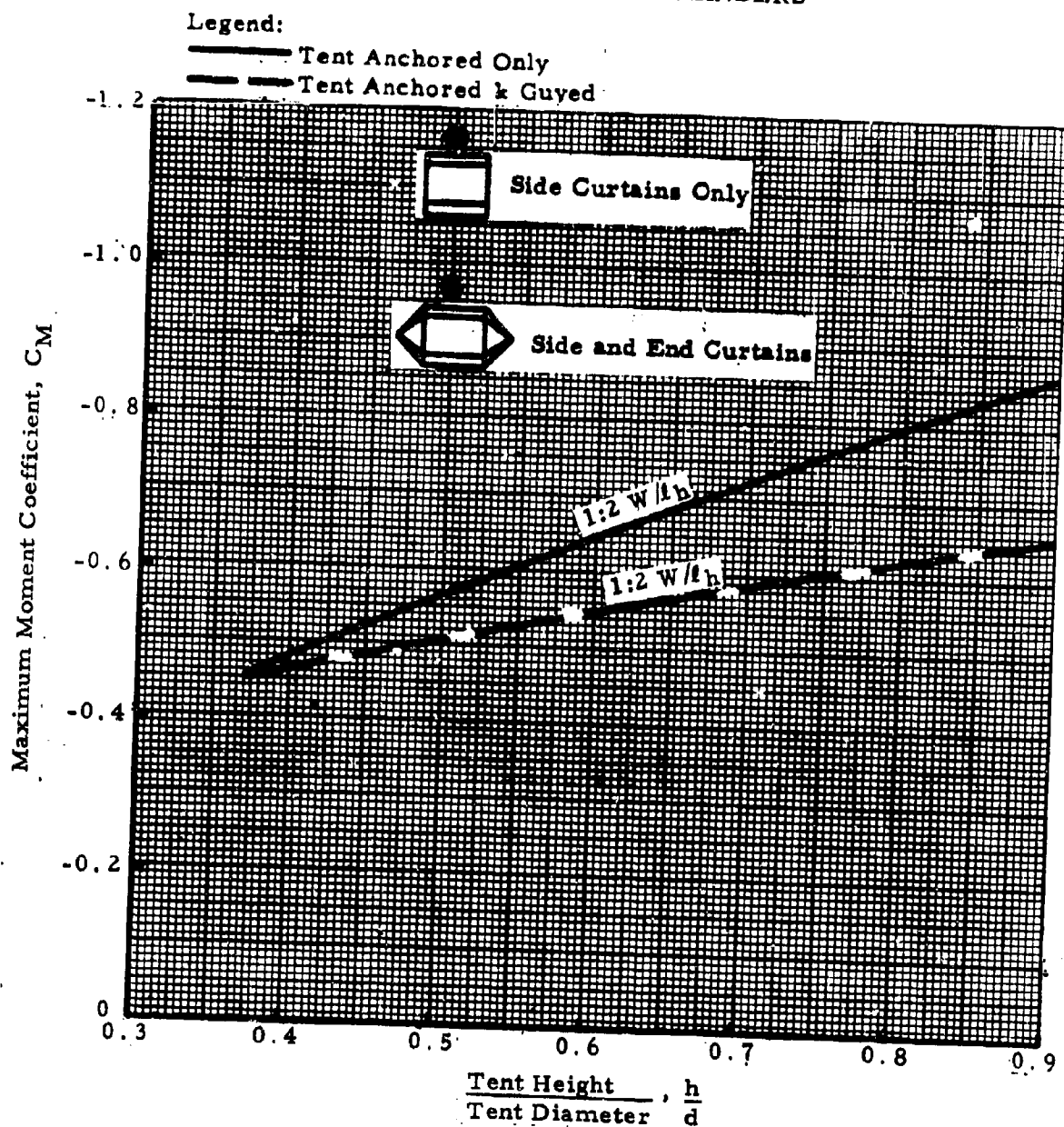
Figure 41. Variation of Moment Coefficient with Shape (Non-Porous Double-Wall Tents; 1:2 W/l h )
