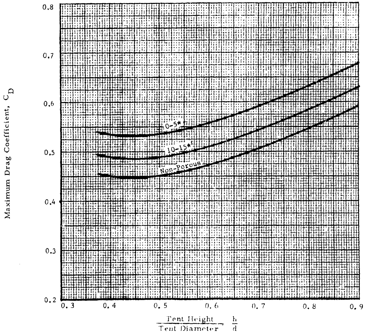
Figure 29. Variation of Drag Coefficient with Shape and Fabric Porosity (Cylindrical Single-Wall Tents, 1:2 W/h )
