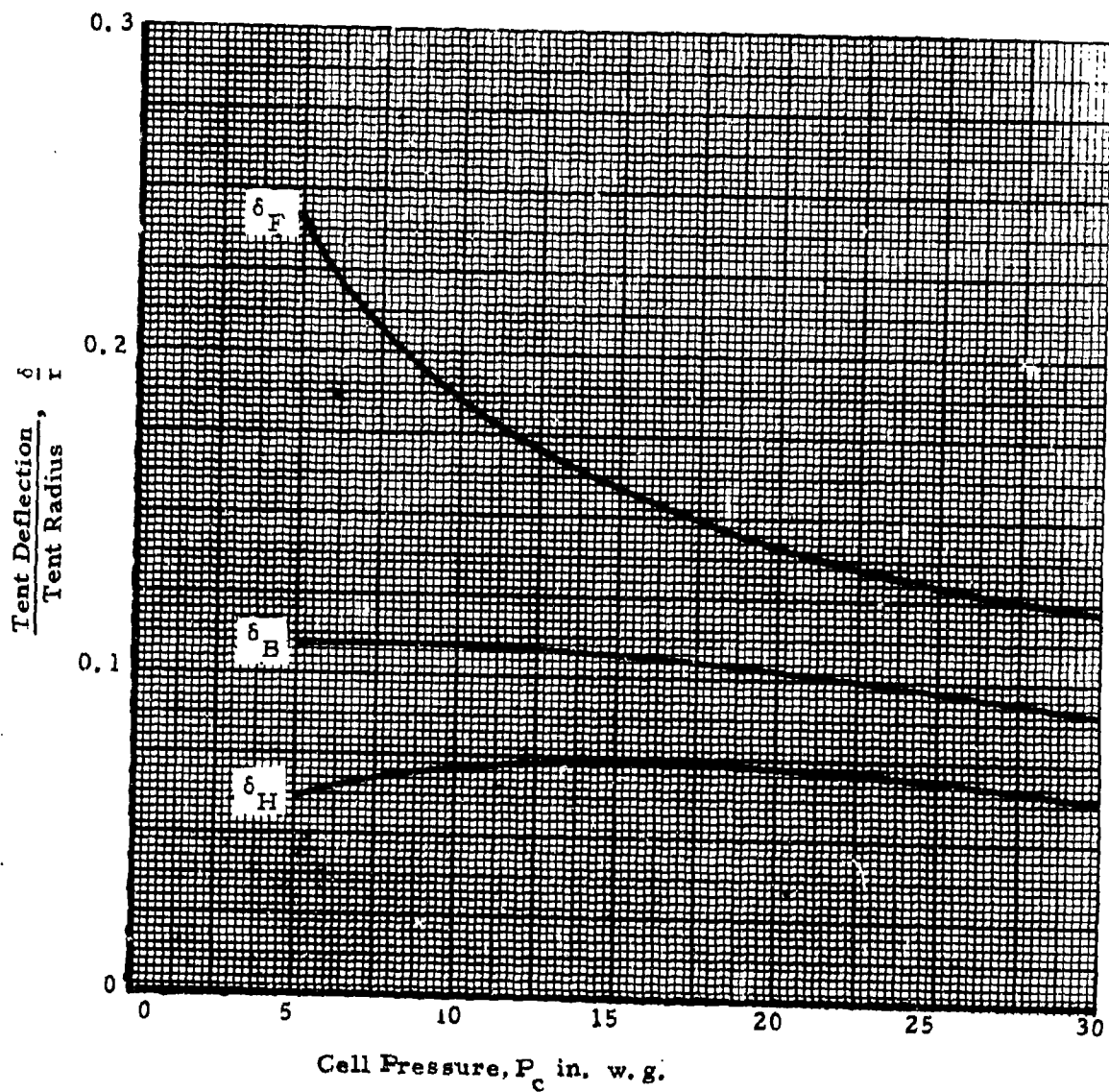
Figure 55. - Variation of Tent Deflection with Cell Pressure. Guy Lines Attached at 0.80 and 0.40 Tent Height
