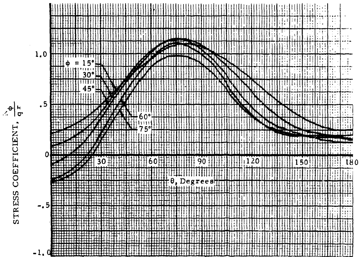
Figure 84. Typical Calculated Stress Coefficients, \frac{N_\phi}{q_r} ; Spherical Ends, h/d = 3/8 , P_e = 4/5q , q = .6
