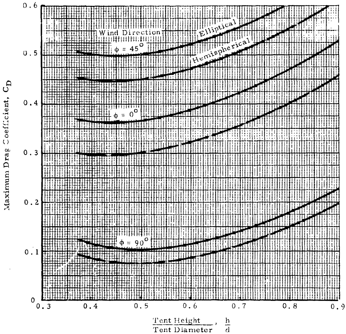
Figure 32. Variation of Drag Coefficient with Shape and Wind Direction; (Cylindrical Single-Wall Tents, 1:2 W/l h )
