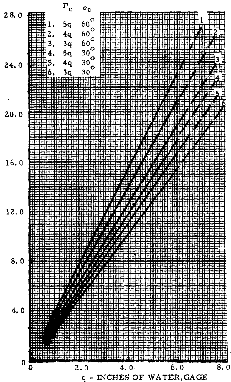
Figure 166. Variation of Meridional Stress Resultant with Impact Pressure, q ; Double-Wall Cylinders, w/d = 0.12 , 9^\circ Sloping Sides, h/d = 0.8
