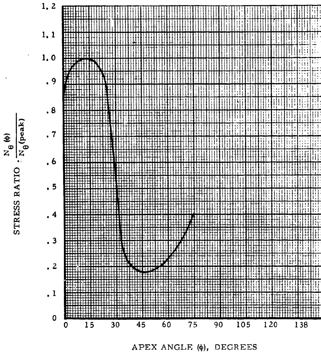
Figure 80. Stress Ratio, \frac{N_{\theta}(\phi)}{N_{\theta}(\text{peak})} Vs. Apex Angle, \phi ; Single-Wall Spheres, h/d = 3/8
