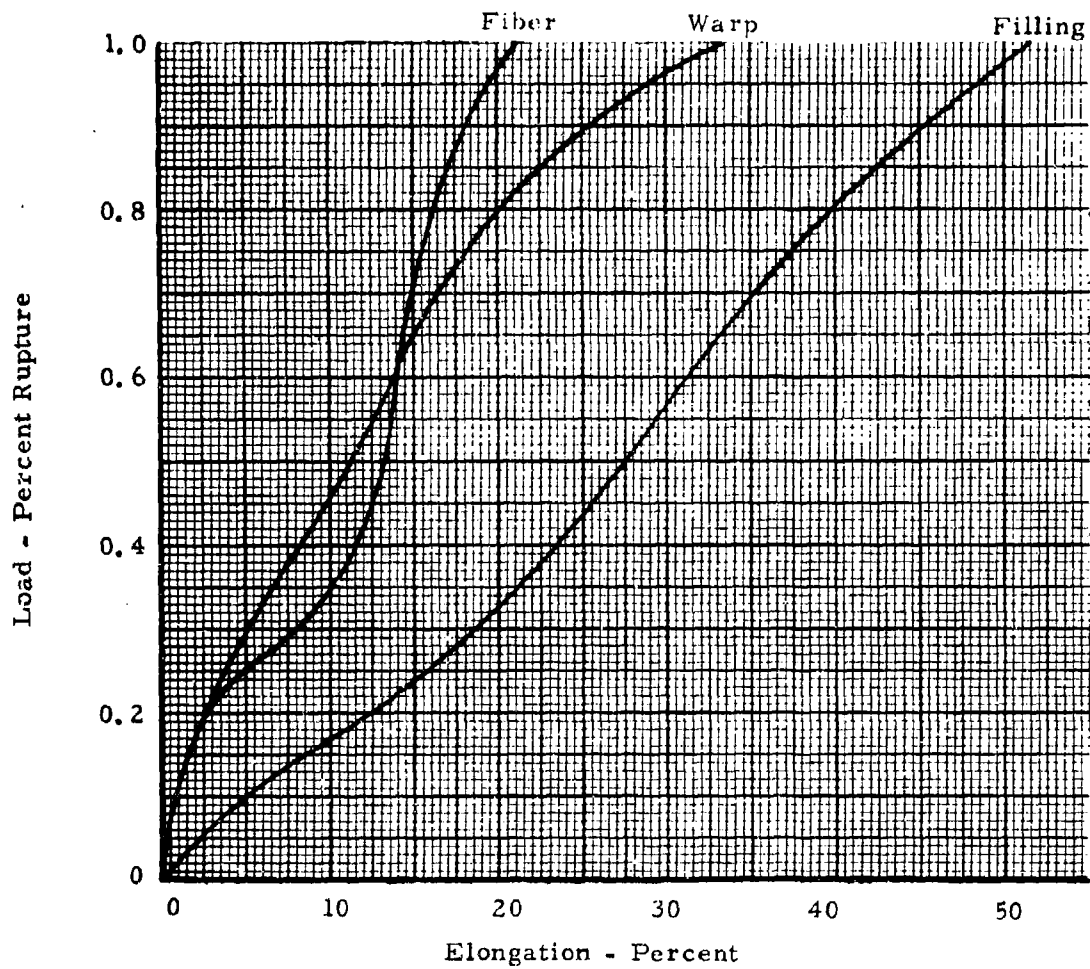
Figure 173. Load - Elongation Diagram of Fiber and Plain Weave Fabric; Polyester
