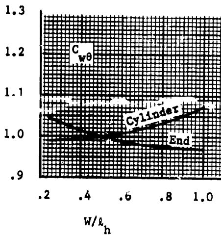
Figure 111. Correction Factors, (\theta) , for Cylindrical Tents with Ellipsoidal Ends
