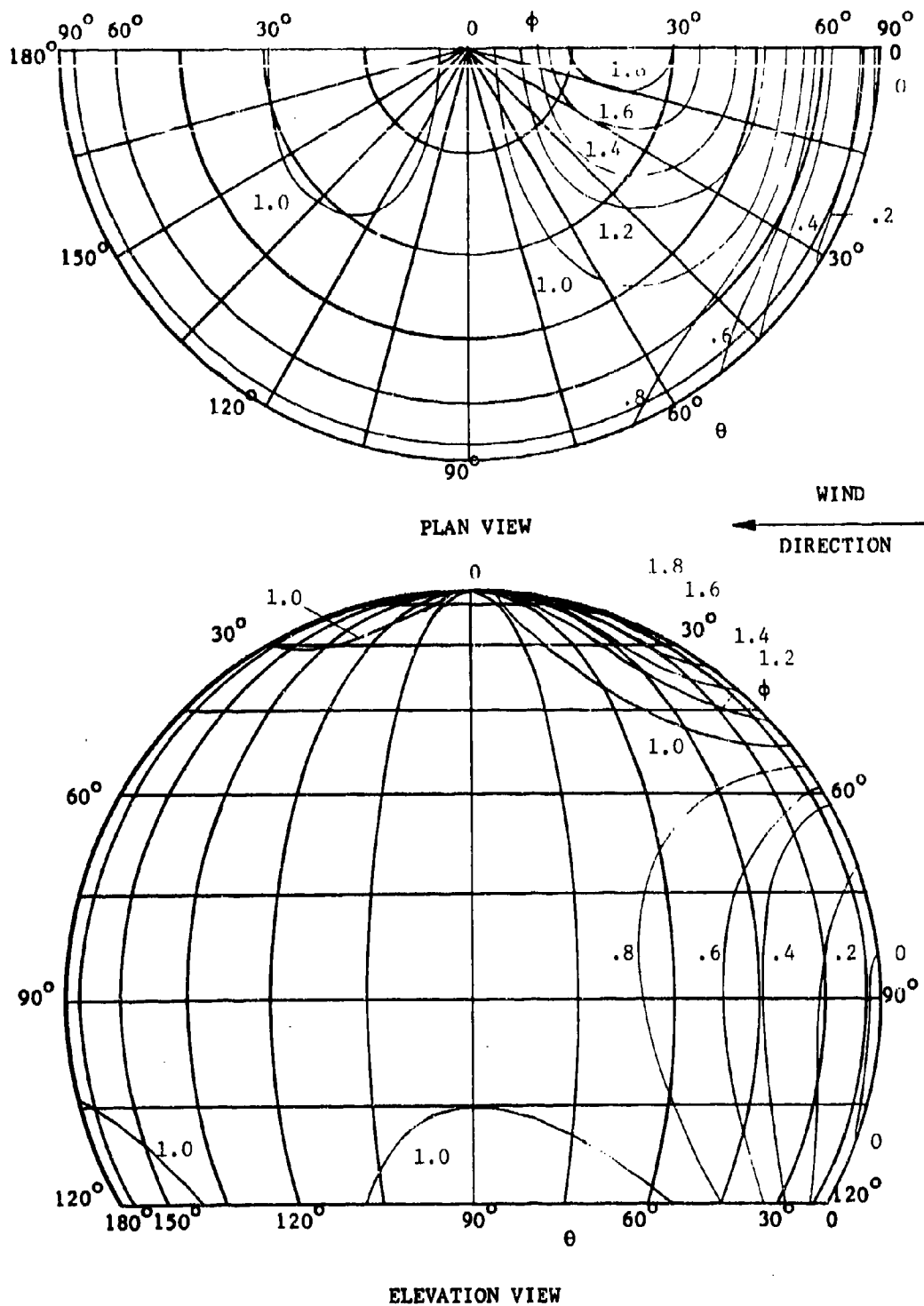
Figure 118. N_\theta/q_r for Spherical Tent ( h/d = 3/4 )
