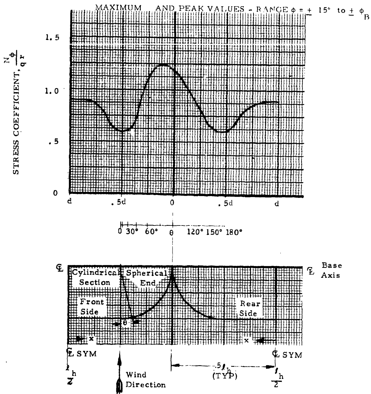
Figure 90. Typical Annular - Longitudinal Stress Coefficient, \frac{N_\phi}{q r} , Distribution; Cylindrical Tents with Spherical Ends, W/l_h = 1/2 , h/d = 3/8
