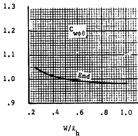
Figure 112. Correction Factors, (\phi\theta) , for Cylindrical Tents with Ellipsoidal Ends
