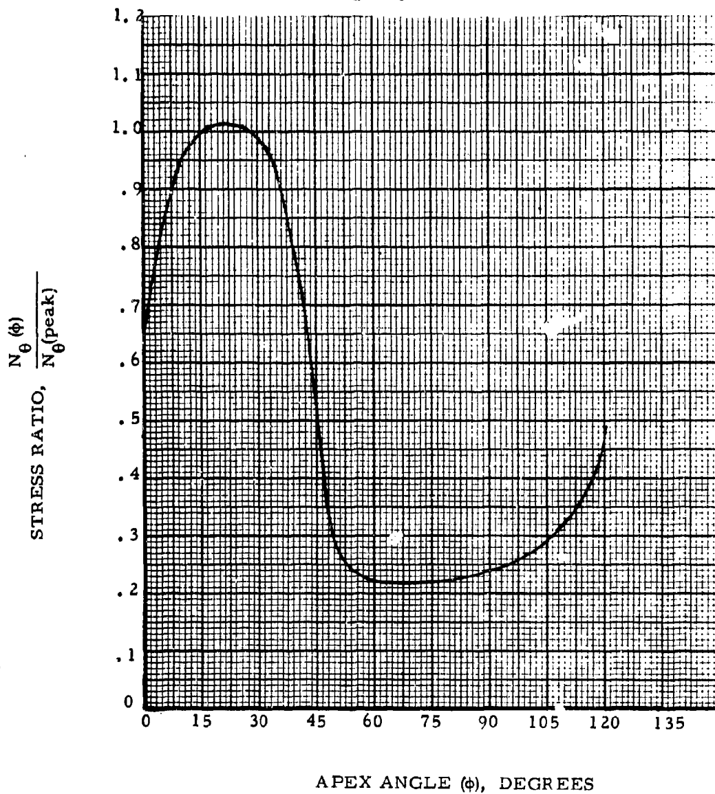
Figure 82. Stress Ratio, \frac{N_{\theta}(\phi)}{N_{\theta}(\text{peak})} Vs. Apex Angle, \phi ; Single-Wall Spheres, h/d = 3/4
