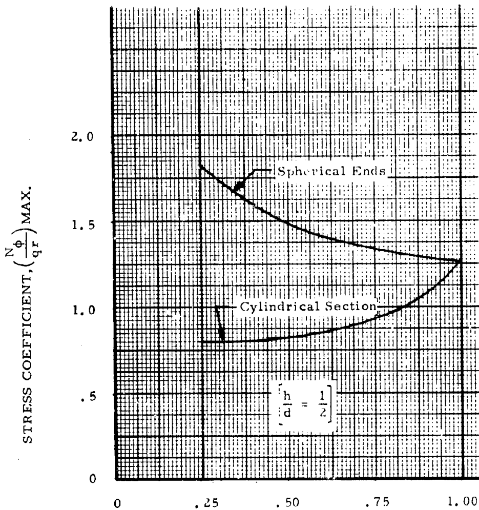
Figure 98. Maximum Design Stress Coefficient, \frac{N}{qr} , Dynamic Pressure Limit ( q = 6.0 ) Constant h/d = W/l_h Range ( W/l_h = .25 to 1.00 ), h/d = 1/2
