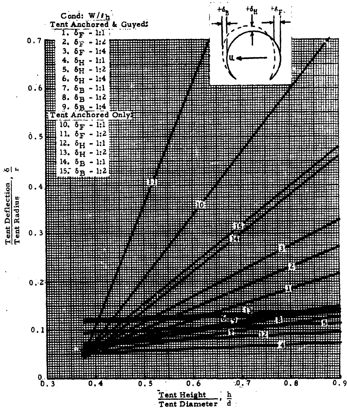
Figure 57. Variation of Tent Deflection with Shape (Non-Porous Double-Wall Tents 1:1, 1:2, 1:4 ( W/l_h ))
