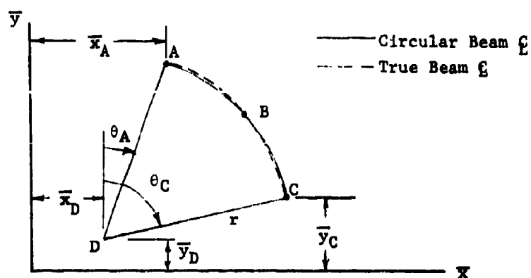
Figure 148. Beam Element Geometry
