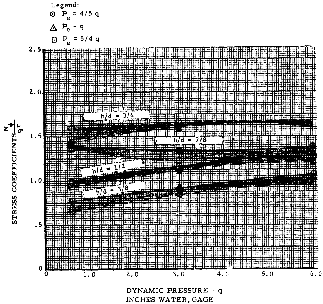
Figure 74. Calculated Peak Stress Coefficients, \frac{N_\phi}{q r} ; Single-Wall Spheres
