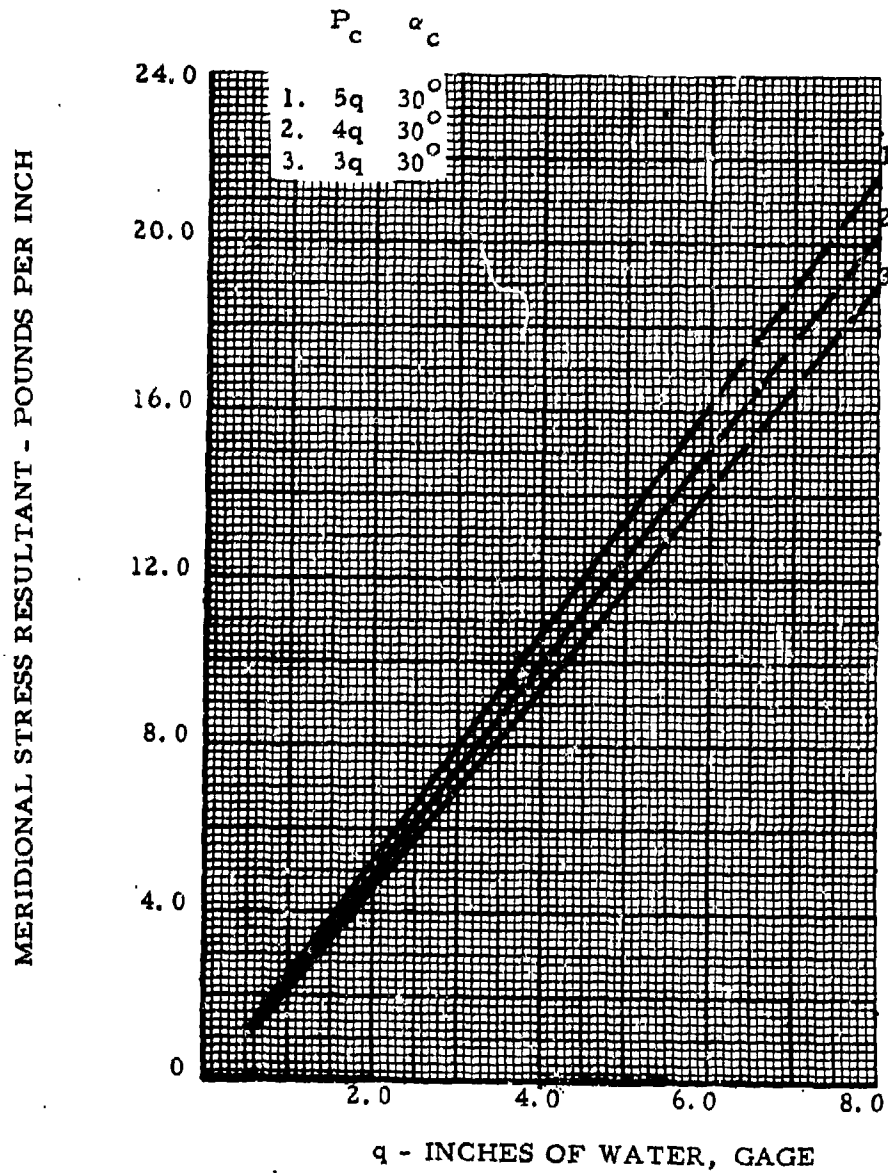
Figure 164. Variation of Meridional Stress Resultant with Impact Pressure, q ; Double-Wall Cylinders, w/d = 0.08 , h/d = .5
