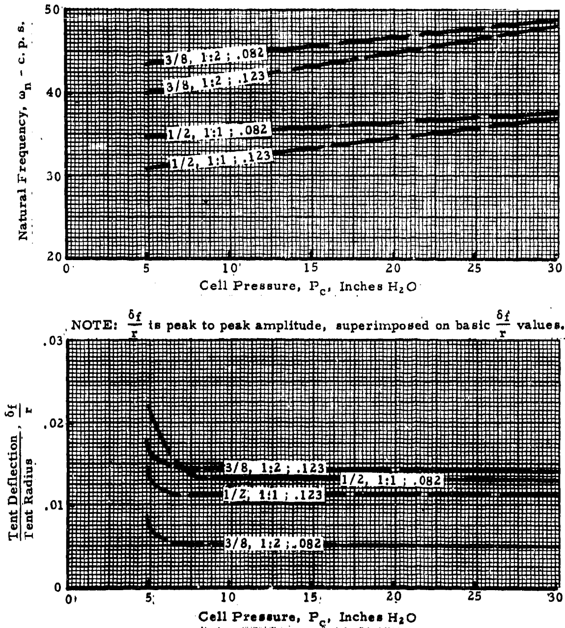
Figure 60. Tent Frequency and Amplitude of Vibration, Guy Lines Installed
