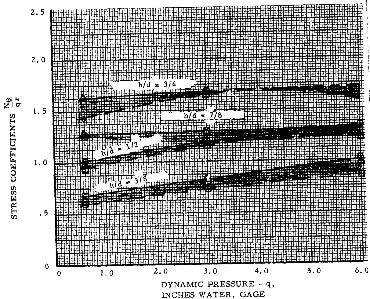
Figure 75. Calculated Peak Stress Coefficients, \frac{N_\theta}{q r} ; Single-Wall Spheres
