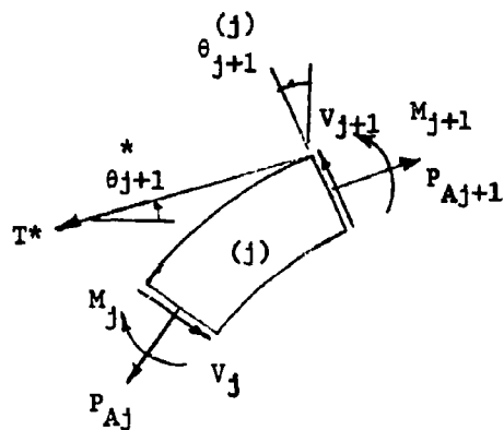
Figure 156. Equilibrium at Guy Wire
