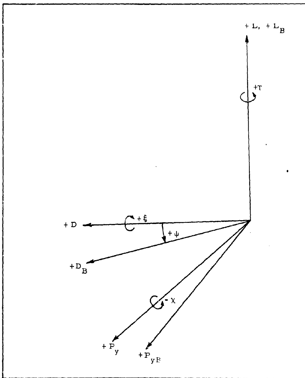
Figure 16. Coordinate System for Transformation from Wind Axes to Body Axes
