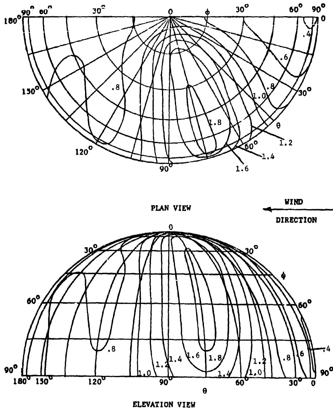
Figure 115. N_\phi/q_r for Spherical Tent ( h/d = 1/2 )
