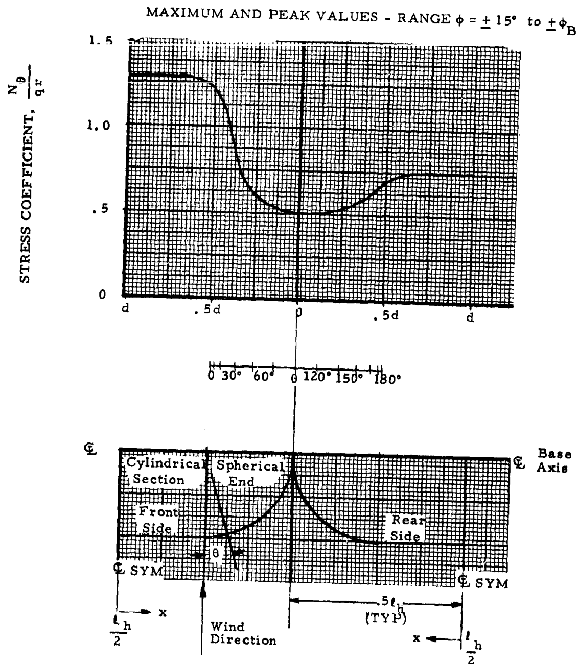
Figure 91. Typical Annular - Longitudinal Stress Coefficient, \frac{N_\theta}{qr} , Distribution; Cylindrical Tents with Spherical Ends, W/l_h = 1/2 , h/d = 3/8
