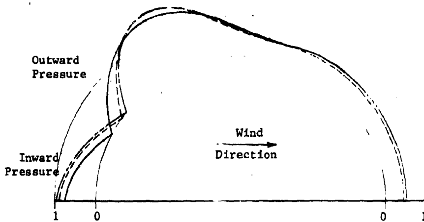
Figure 137. Pressure Distribution on Guyed Double-Wall Tents ( h/d = 1/2 , W/\ell_h = 1/2 )
