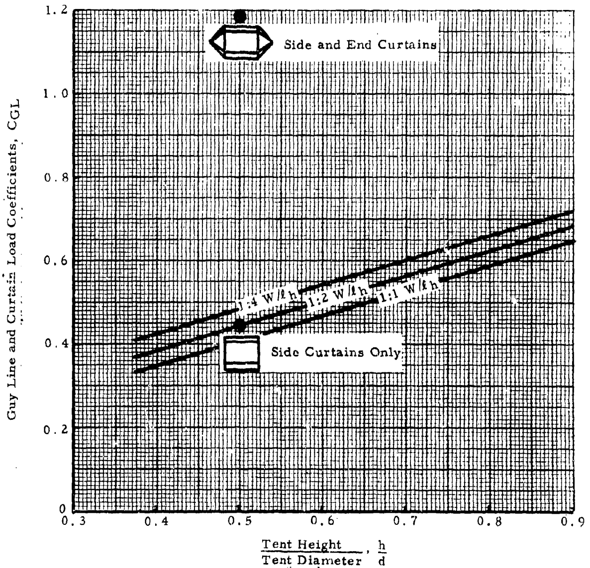
Figure 49. Variation of Guy Line Load Coefficient with Shape
