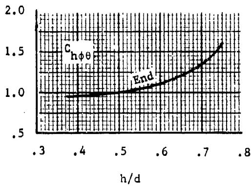
Figure 112. Correction Factors, (\phi\theta) , for Cylindrical Tents with Ellipsoidal Ends
