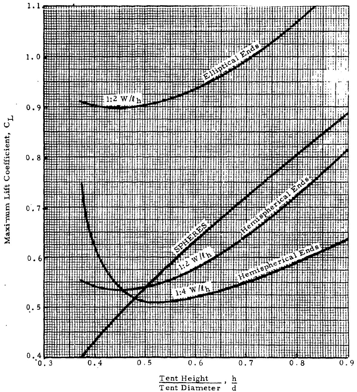
Figure 25. Variation of Lift Coefficient with Shape (Non-Porous Spherical and Cylindrical Single-Wall Tents; 1:2, 1:4, W/l_h )
