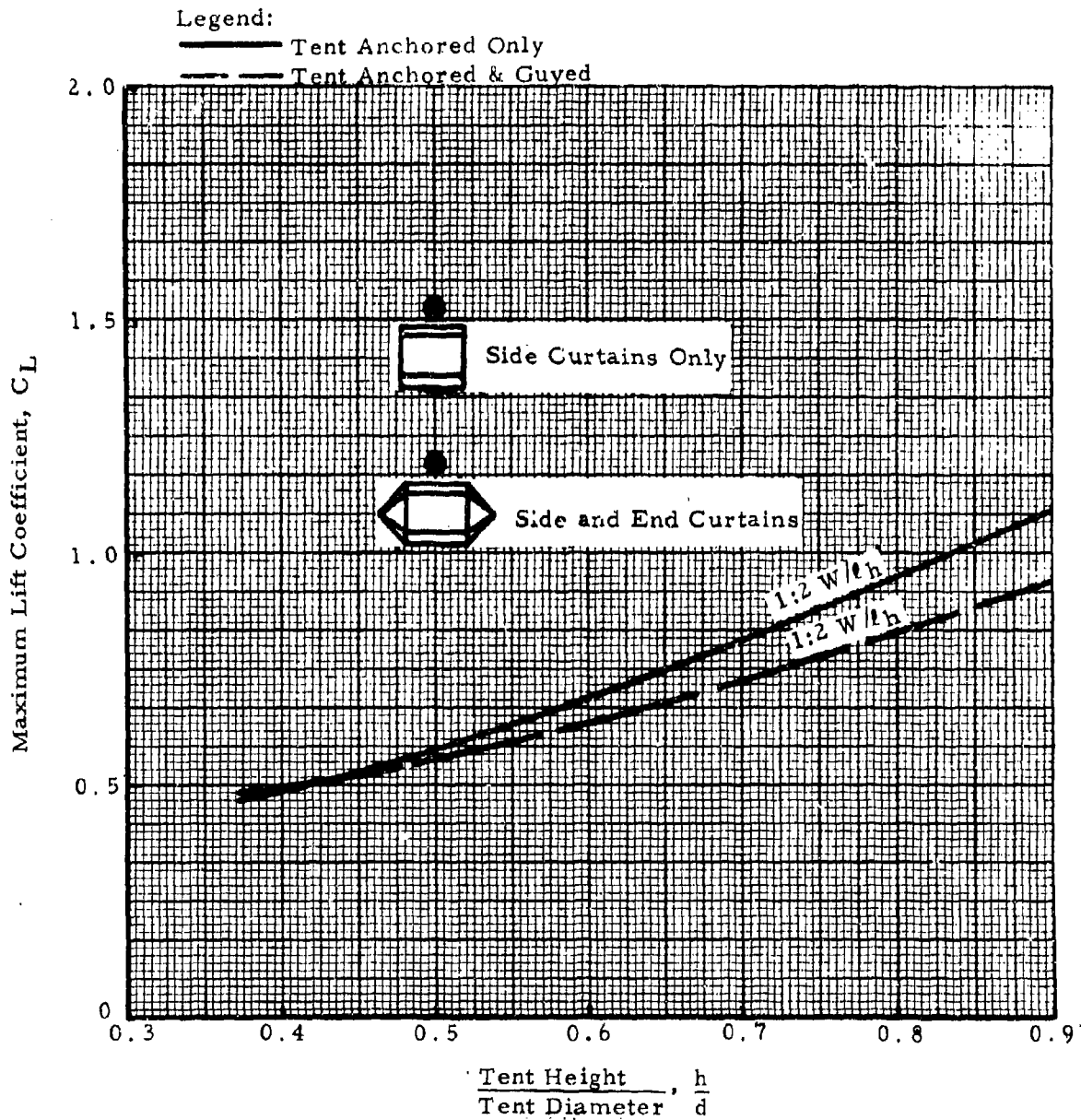
Figure 27. Variation of Lift Coefficient with Shape (Non-Porous Double-Wall Tents; 1:2 W/h)
