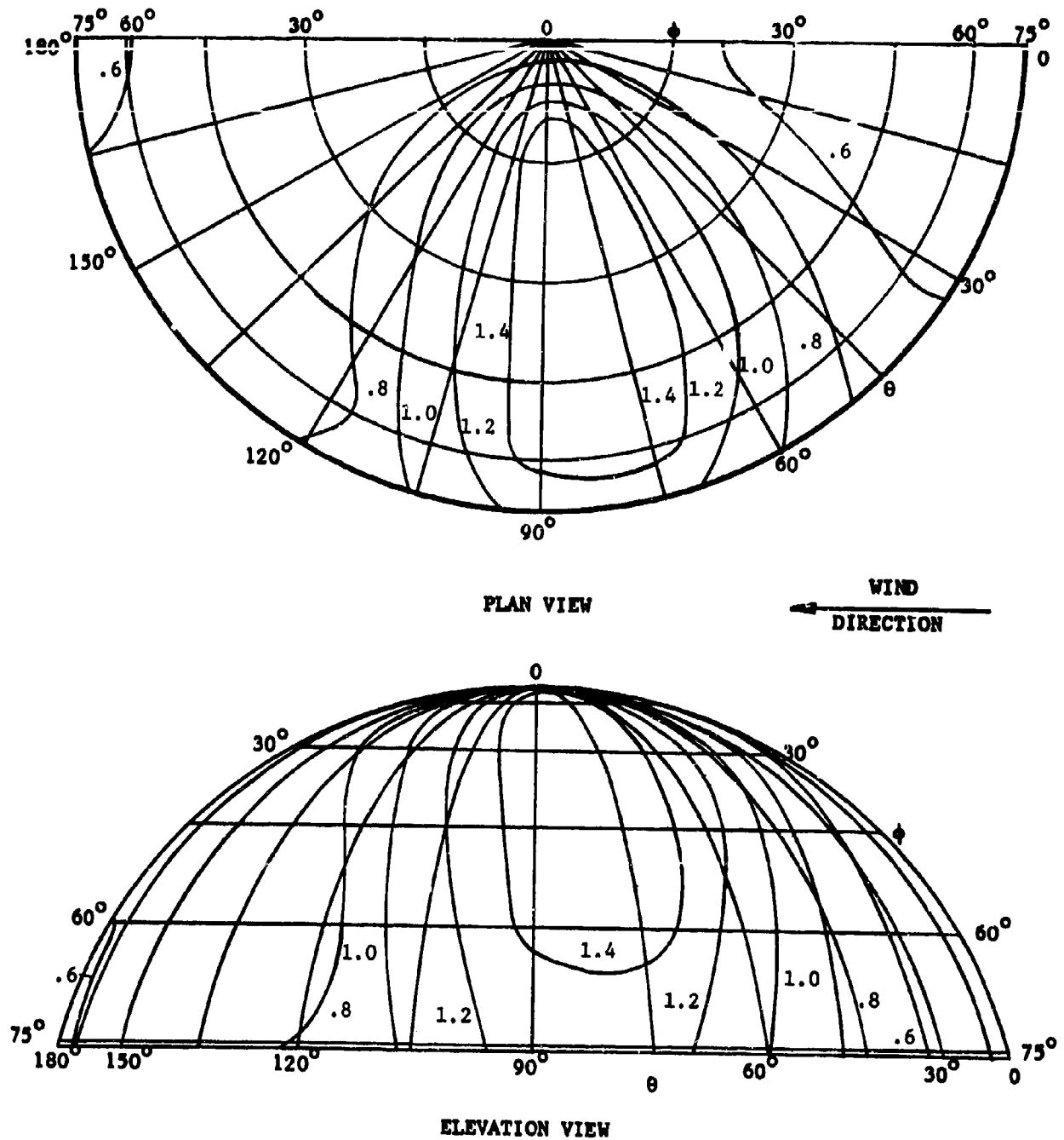
Figure 113. N_\phi/q_r for Spherical Tent ( h/d = 3/8 )
