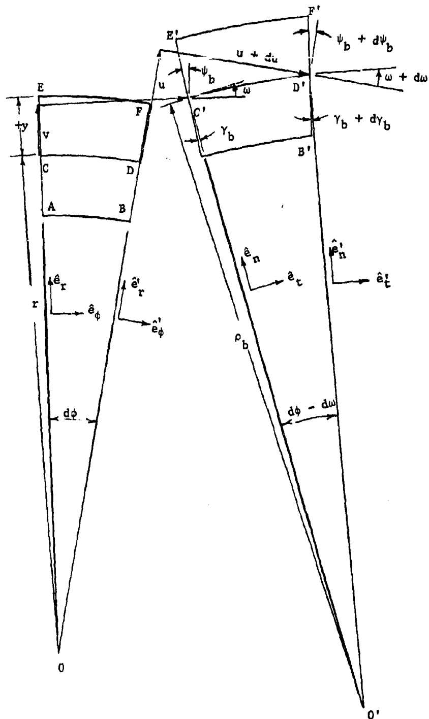
Figure 144. Deformation of Circular Beam Element
