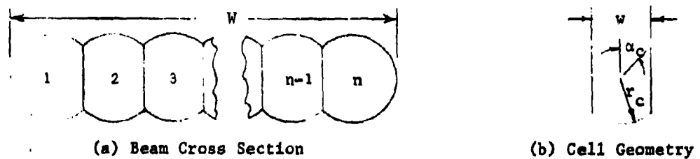
Figure 139. Cellular Beam Cross Section
