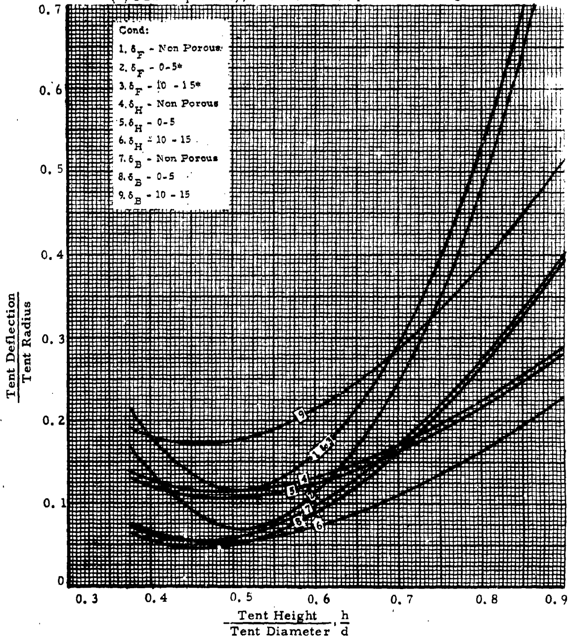
Figure 53 Variation of Tent Deflection with Shape and Fabric Porosity (Cylindrical Single-Wall Tents, 1:4 W/h)
