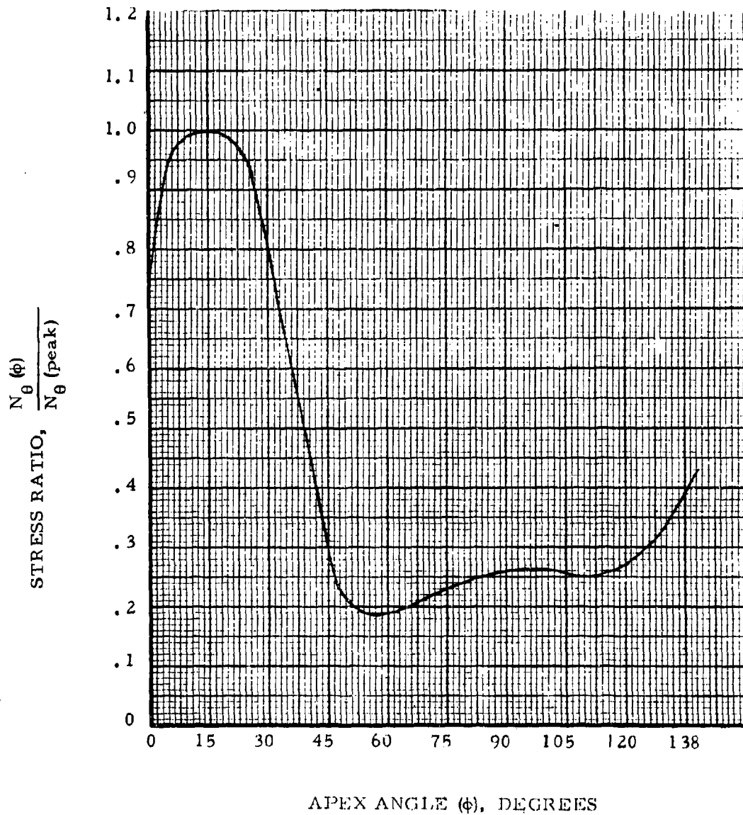
Figure 83. Stress Ratio, \frac{N_{\theta}(\phi)}{N_{\theta}(\text{peak})} Vs. Apex Angle, \phi ; Single-Wall Spheres, h/d = 7/8
