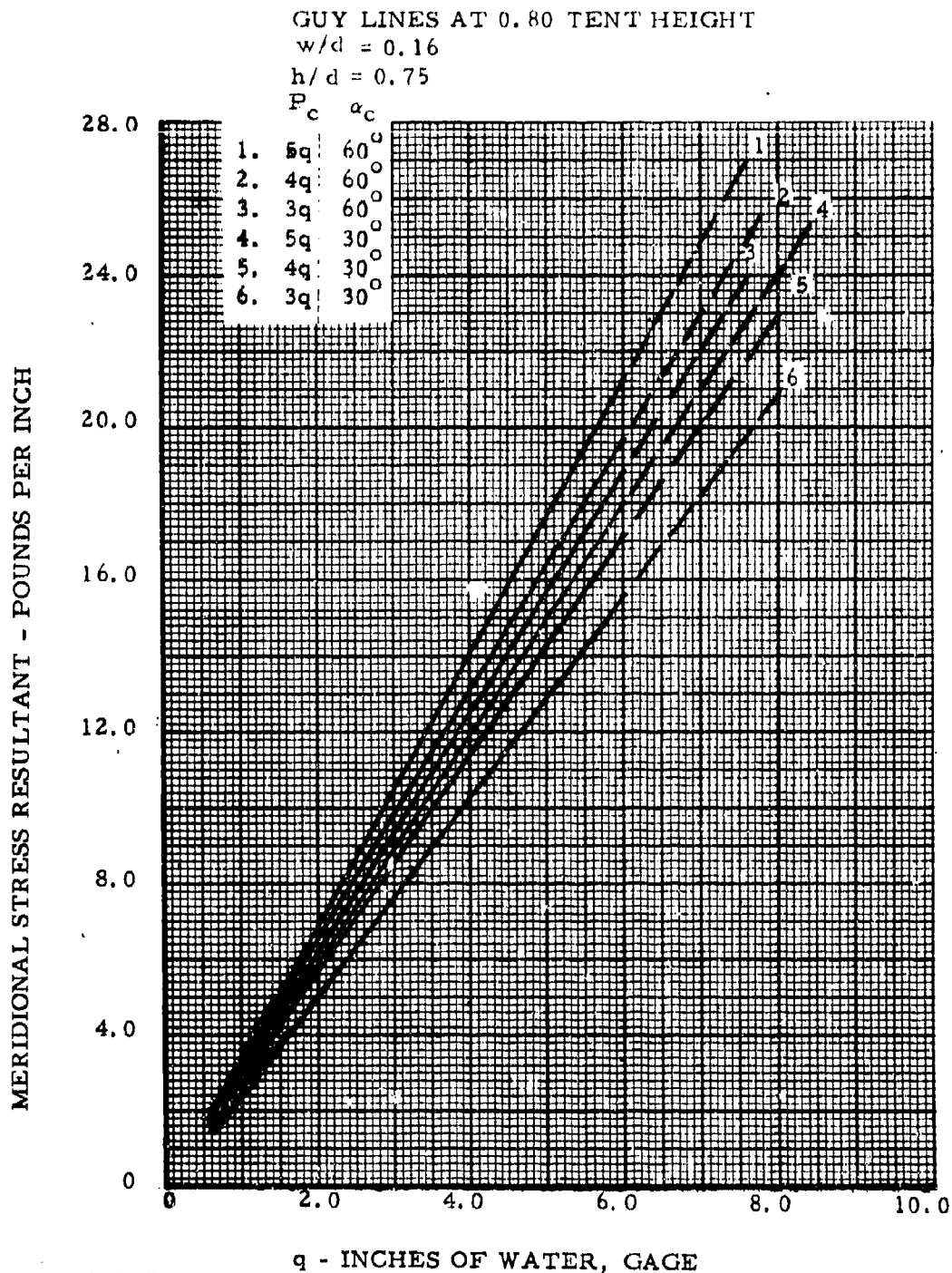
Figure 168. Variation of Meridional Stress Resultant with Impact Pressure, q ; Double-Wall Cylinders, w/d = 0.16 , h/d = 0.75
