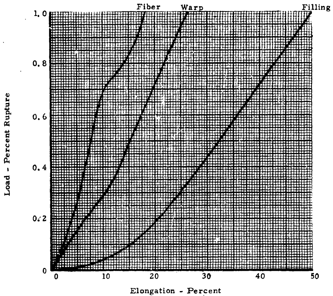
Figure 172. Load - Elongation Diagram of Fiber and Plain Weave Fabric; Nylon
