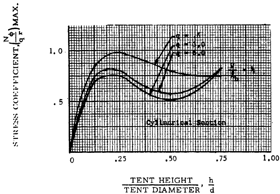
Figure 94. Maximum Design Stress Coefficient, \frac{N}{q_r} , Specific Dynamic Pressure
