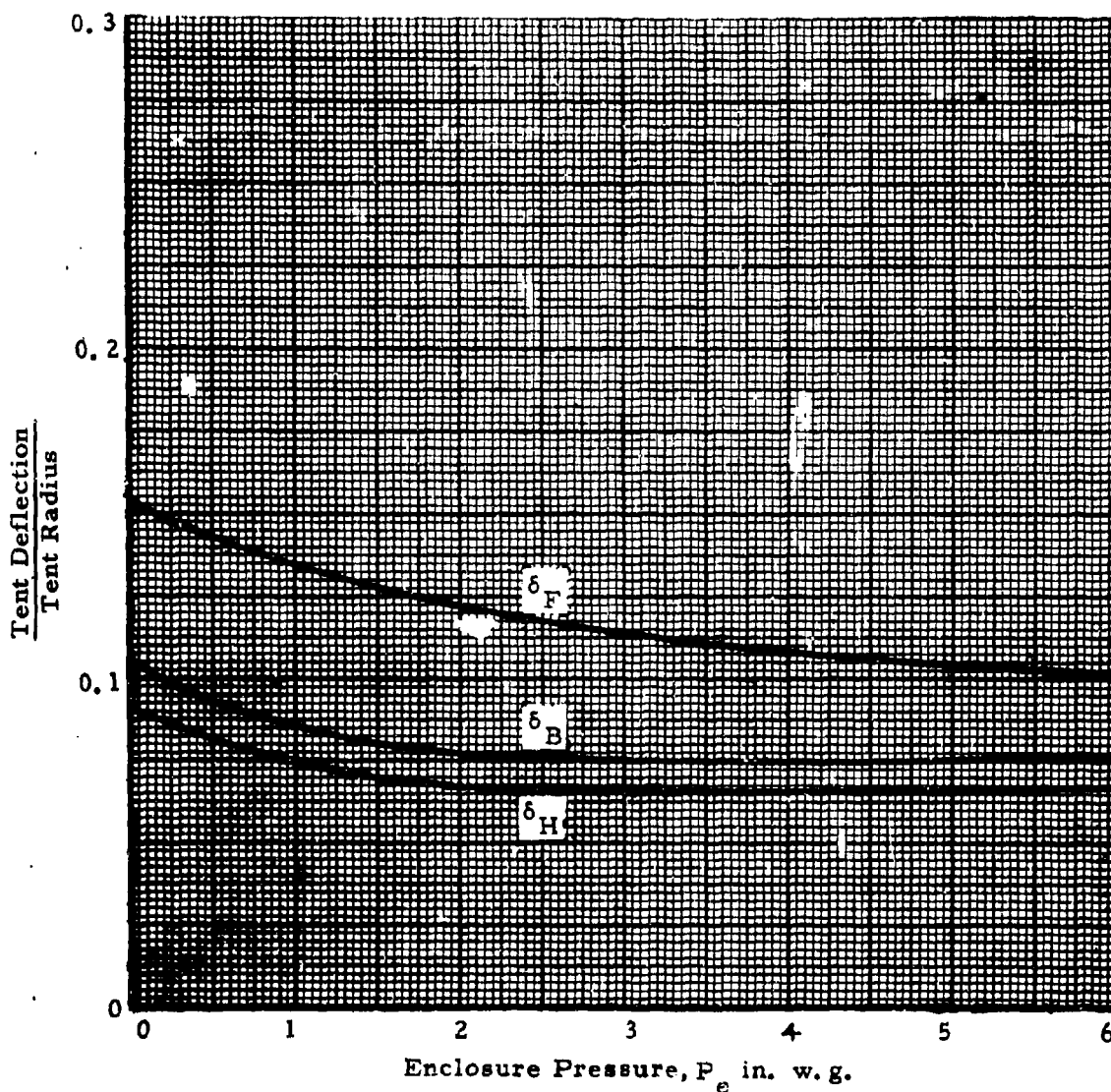
Figure 56. Variation of Tent Deflection With Enclosure Pressure. No Guy Lines, Constant Cell Pressure = 5.0'' w. g., Broadside to Wind ( \psi = 0^\circ )
