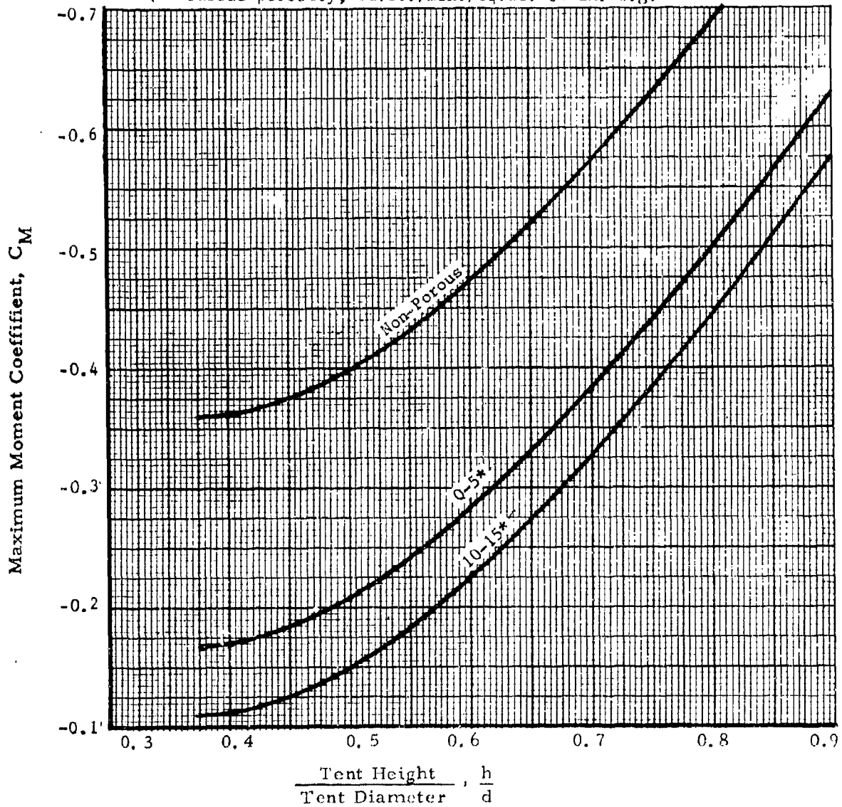
Figure 36. Variation of Moment Coefficient with Shape and Fabric Porosity (Cylindrical Single-Wall Tents, 1:2 W/h )
