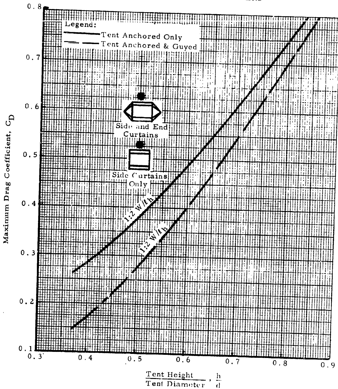
Figure 34. Variation of Drag Coefficient with Shape (Non-Porous Double-Wall Tents; 1:2 W/h)
