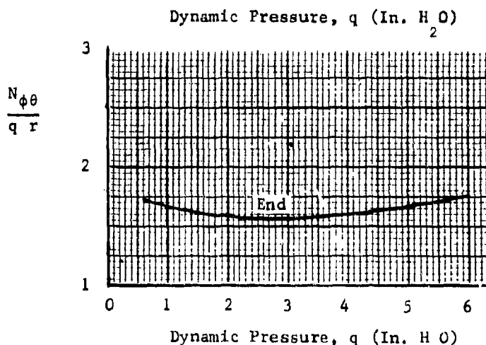
Figure 109. Basic Maximum Stress Coefficients for Cylindrical Tents with Ellipsoidal Ends, b/R = 1/2
