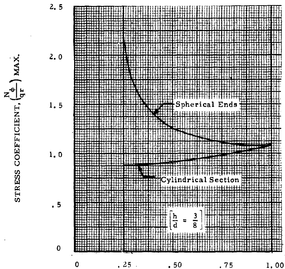
Figure 97. Maximum Design Stress Coefficient, \frac{N_{\phi}}{q_r} , Dynamic Pressure Limit ( q = 6.0 ) Constant h/d = W/l_h Range ( W/l_h = .25 to 1.00 ), h/d = 3/8
