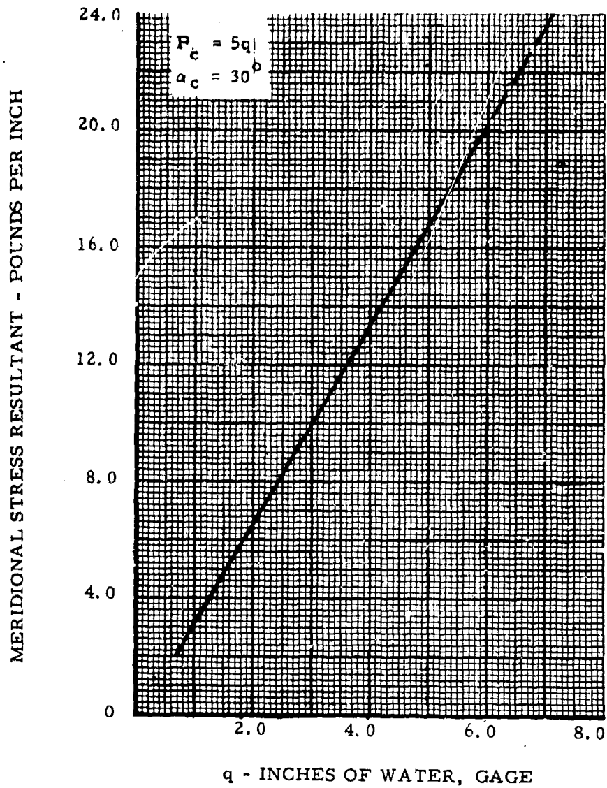
Figure 170. Variation of Meridional Stress Resultant with Impact Pressure, q ; Double-Wall Cylinders, w/d = 0.08 , h/d = 0.75
