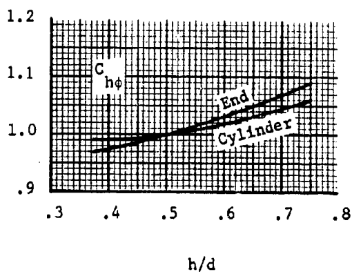
Figure 110. Correction Factors, (\phi) , for Cylindrical Tents with Ellipsoidal Ends
