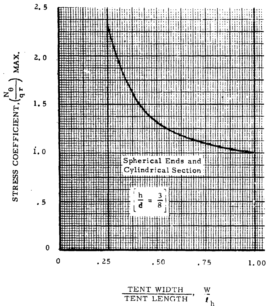
Figure 100. Maximum Design Stress Coefficient, \frac{N_{\theta}}{qr} , Dynamic Pressure
