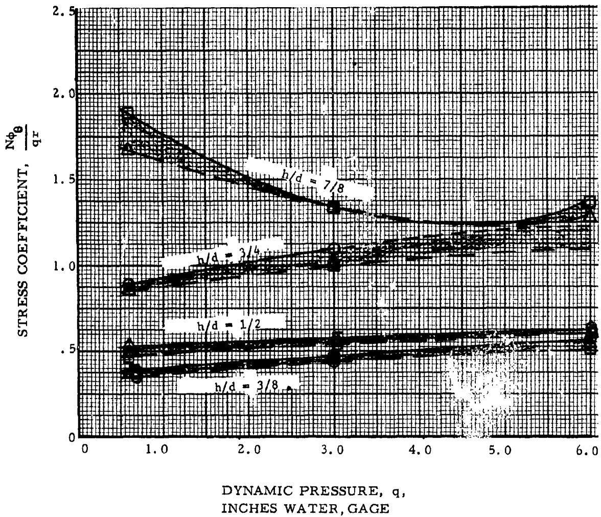
Figure 76. Calculated Peak Stress Coefficients, \frac{N_{\phi\theta}}{qr} ; Single-Wall Spheres
