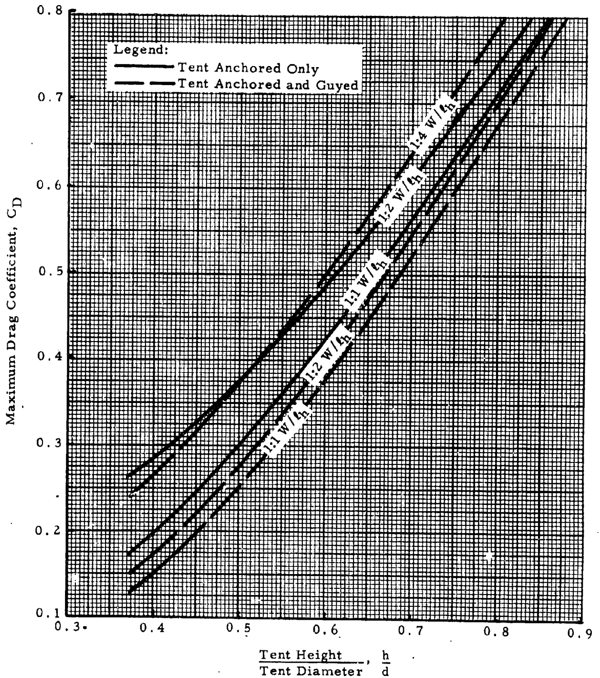
Figure 33. Variation of Drag Coefficient with Shape (Non-Porous Double-Wall Tents; 1:1, 1:2, 1:4 W/t_h )
