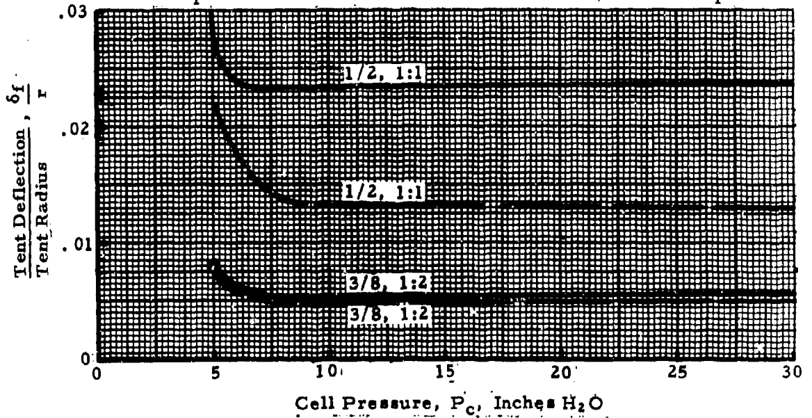
Figure 61. Tent Frequency and Amplitude of Vibration, Comparison of Guyed & Unguyed Conditions
