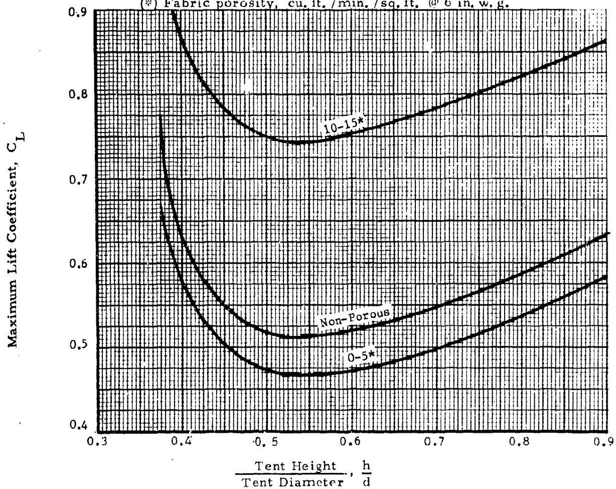
Figure 24. Variation of Lift Coefficient with Shape and Fabric Porosity (Cylindrical Single-Wall Tents, 1:4 W/h )
