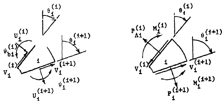
Figure 150. Point Geometry and Equilibrium
