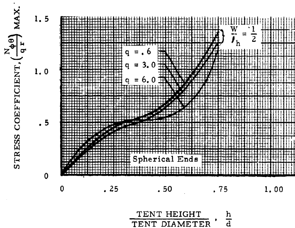
Figure 96. Maximum Design Stress Coefficient, \frac{N_{\phi\theta}}{q_r} , Specific Dynamic Pressure
