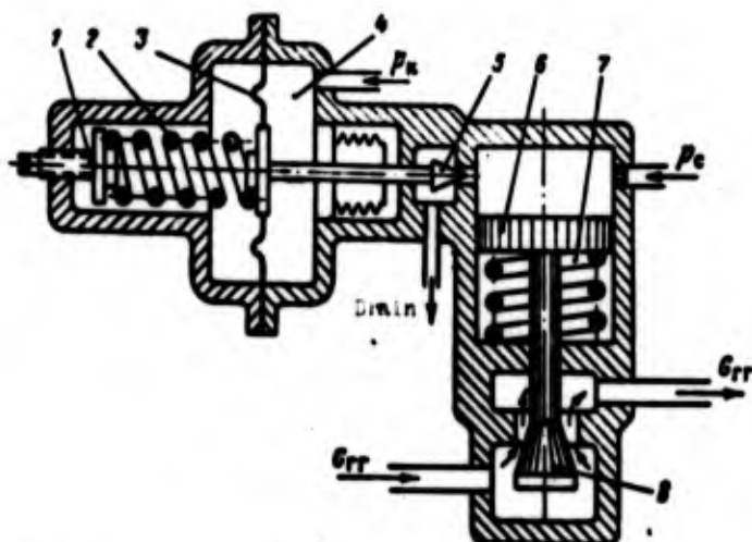
Fig. 17.1. Schematic diagram of a thrust regulator with hydraulic static servomotor: 1 - regulator adjusting screw; 2 - sensing device spring; 3 - sensing device diaphragm; 4 - gas feed cavity with pressure p_k ; 5 - servomotor controlling element; 6 - servomotor piston; 7 - servomotor spring; 8 - regulating element.
