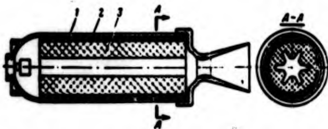
Fig. 18.1. Diagram of an RDTT with inserted charge: 1 - armoring; 2 - combustion chamber case; 3 - charge.
