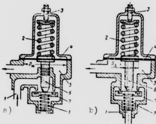
Fig. 15.14. Diagrams of reduction gears: a) direct action; b) reverse action; 1 - inlet channel; 2 - spring; 3 - regulating screw; 4 - diaphragm; 5 - outlet cavity of the reduction gear; 6 - valve rod; 7 - valve; 8 - locking spring.
