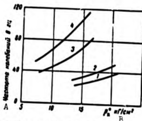
Fig. 6.2. Oscillation frequency as a function of chamber pressure for two fuels and two values of L^* . 1, 2) \text{HNO}_3 + octane; 3, 4) \text{HNO}_3 + furfuryl alcohol; 1, 3) L^* = 3.55 m; 2, 4) L^* = 2.35 m. A) Oscillation frequency, Hz; B) \text{kgf/cm}^2 .
