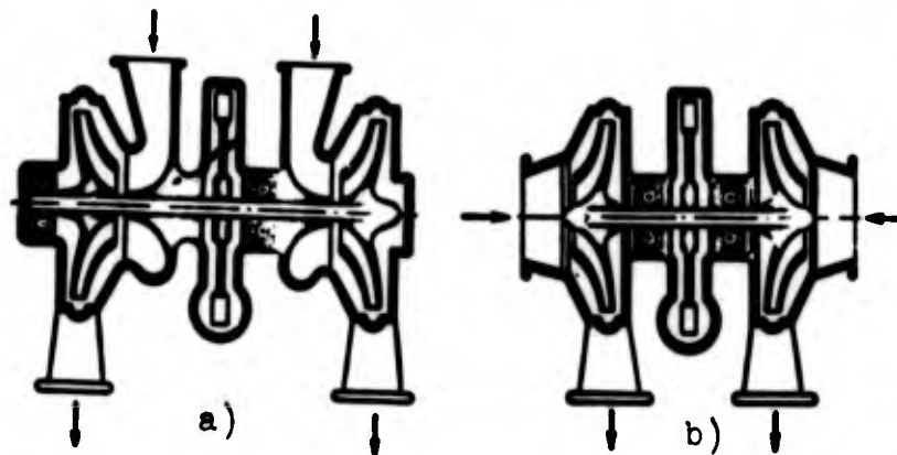
Fig. 14.3. Diagrams of TNA with turbine in the middle of the rotor: a) pumps have inlets inside; b) pumps have inlets outside.
