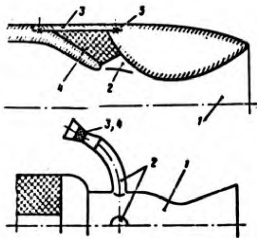
Fig. 5.20. Two thrust-reversible arrangements. 1) Main nozzle; 2) additional reversal nozzle; 3) caps; 4) heat insulation; 5) break-away charge.
