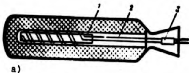
Fig. 18.22. Corded igniters: a) made of explosive wire; b) made of pyrotechnic cord; 1 - plastic tube; 2 - detonating cord; 3 - low energy detonator; 4 - pyrotechnic cord.
