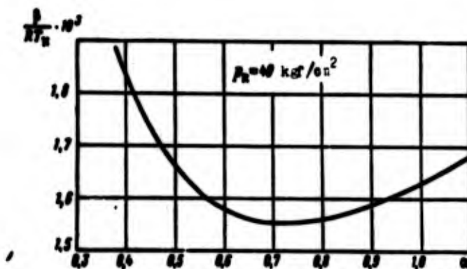
Fig. 16.5. Dependence of complex of parameters \beta/RT_n on excess oxidant ratio.
