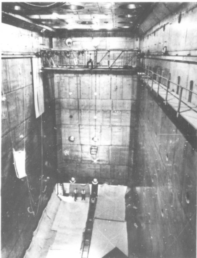
WATER TANK - 100 FEET LONG, 75 FEET DEEP, 35 FEET WIDE WATER DEPTH - MAXIMUM OF 65 FEET CONSTRUCTION - STAINLESS STEEL LINED TANK, SUPPORTED BY REINFORCED CONCRETE
