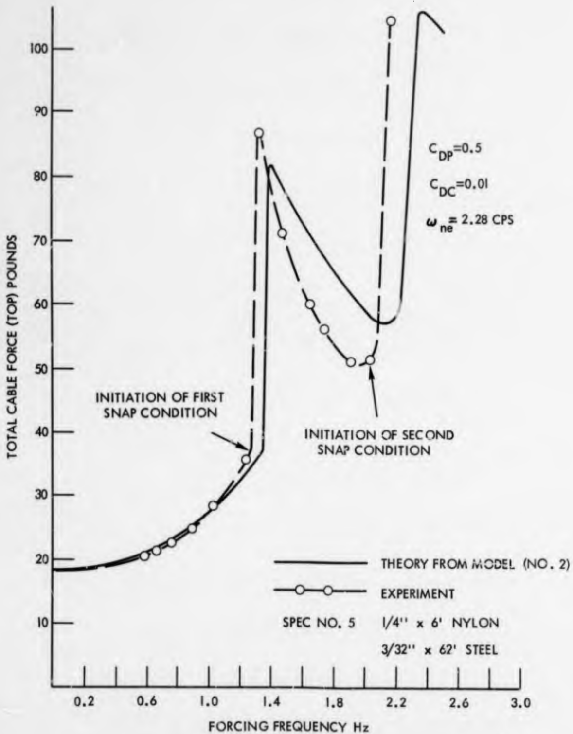
FIG. 12 MAXIMUM CABLE FORCE VERSUS FREQUENCY FOR SPECIMEN NO. 5 IN WATER SHOWING COMPARISON OF EXPERIMENT WITH MODEL (NO. 2) ( X_0 = 2'' )
