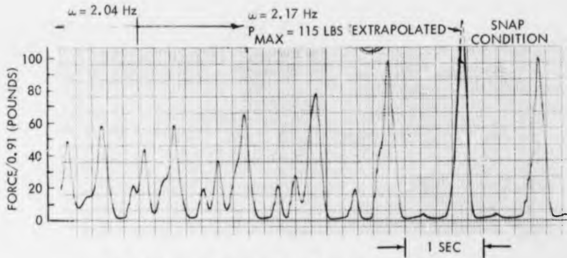
(d) FORCE GOING THROUGH SECOND RESONANCE CONDITION
