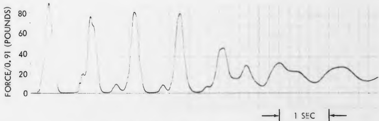
(f) RAPID DROPOFF IN FORCE WHILE REDUCING FORCING FREQUENCY FROM 1.17 HZ TO 0.91 HZ
