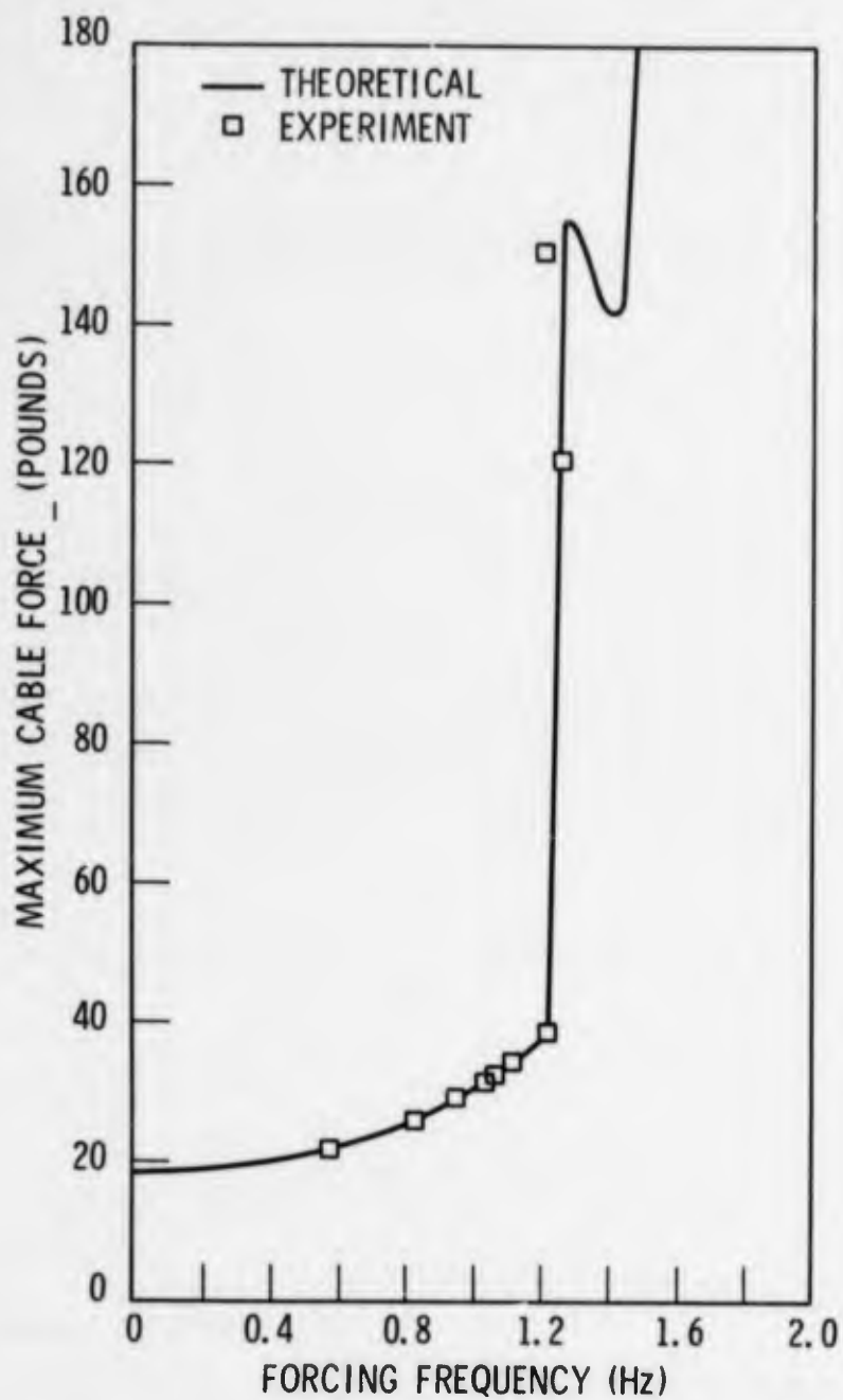
FIG. 9 FORCE AT TOP OF 1/16" STEEL CABLE (SPECIMEN NO. 2) VERSUS FORCING FREQUENCY - COMPARISON OF EXPERIMENT WITH DIGITAL PROGRAM (MODEL NO 2)
