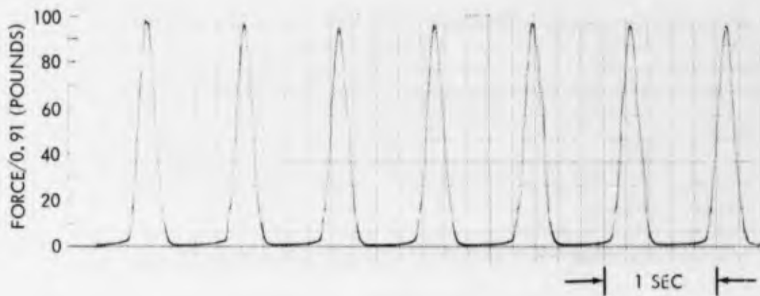
(e) SNAP CONDITION AFTER DECREASE OF FREQUENCY FROM MAXIMUM
