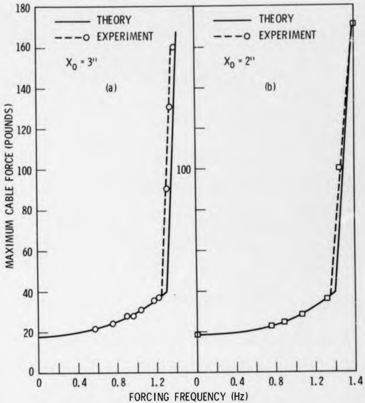
FIG. 10 FORCE AT TOP OF 3/32" STEEL CABLE (SPECIMEN NO. 1) VERSUS FORCING FREQUENCY - COMPARISON OF EXPERIMENT WITH DIGITAL PROGRAM (MODEL NO. 2)
