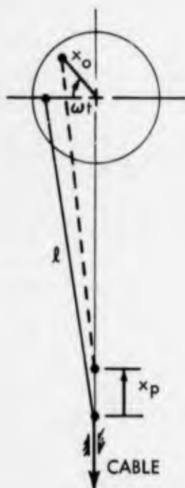
FIG. 2 ILLUSTRATION OF DRIVING MOTION APPLIED TO TOP OF CABLE
