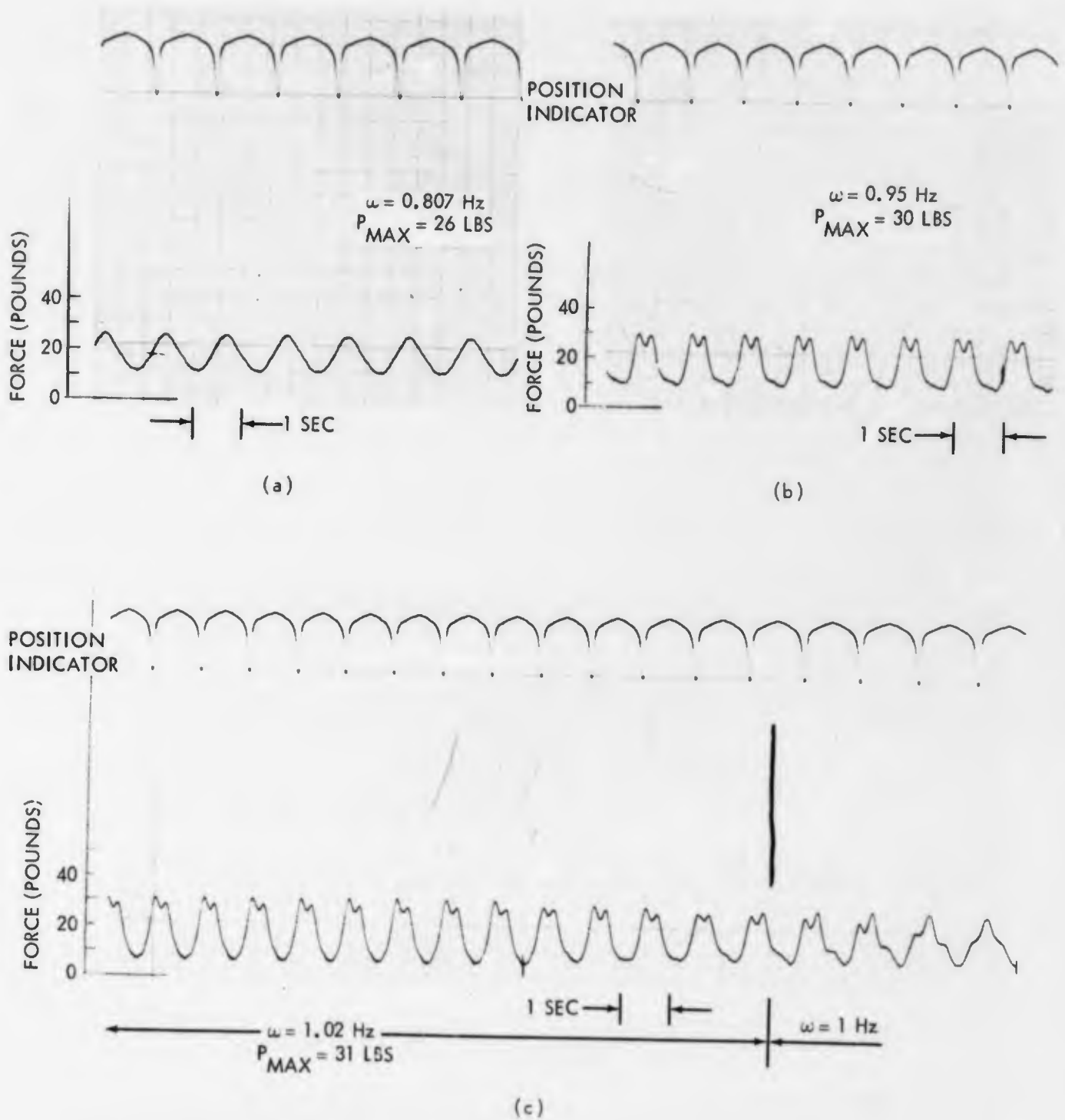
FIG. 7 EXPERIMENTAL FORCE RESPONSE AT TOP OF 1/16" STEEL CABLE IN WATER ( SPECIMEN NO. 2 ) AT VARIOUS FORCING FREQUENCIES ( X_0 = 3" )
