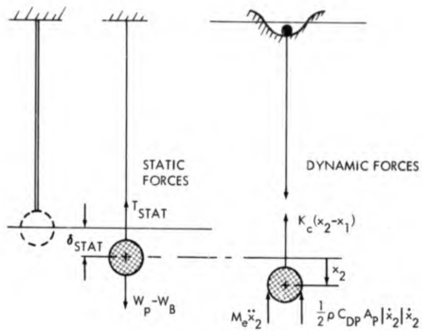
FIG. 1 STATIC AND DYNAMIC FORCES AND DISPLACEMENTS FOR ANALOG MODEL
