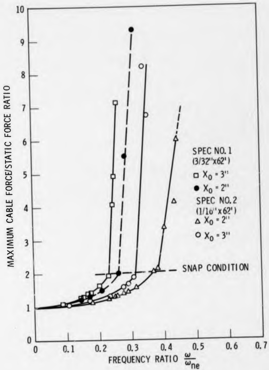
FIG. 13 EXPERIMENTAL FORCE RATIO P_{MAX}/T_{STAT} VERSUS FREQUENCY RATIO FOR 1/16" AND 3/32" STEEL CABLES
