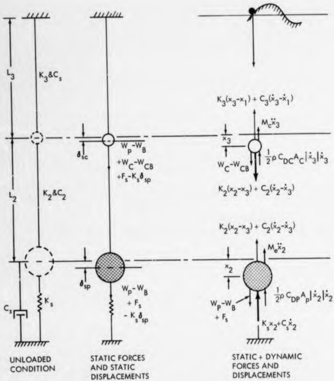
FIG. 4 ILLUSTRATION OF FORCES AND DISPLACEMENTS IN SEGMENTED CABLE SYSTEM - MODEL (NO. 2)
