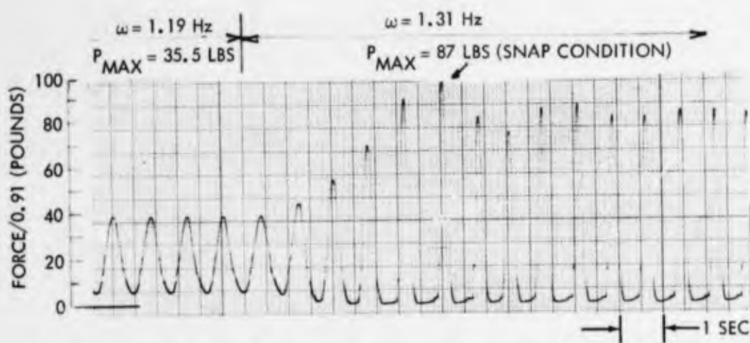
(b) FORCE RESPONSE GOING THROUGH RESONANCE - SNAP LOADING IS INITIATED
