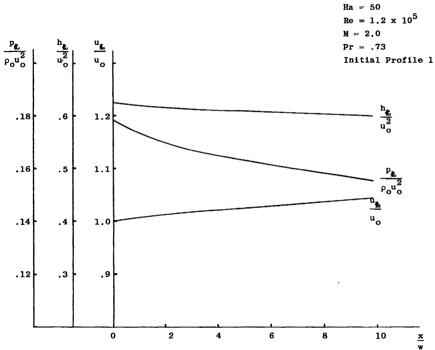
Figure 33. Centerline Distributions of Velocity, Enthalpy, Pressure.
