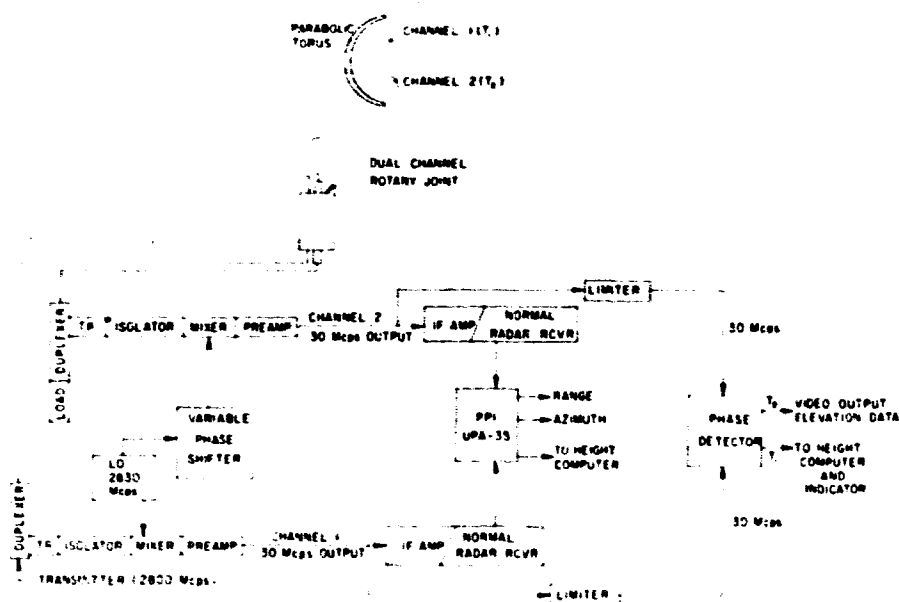
Figure 2. Block Diagram Showing Details of 3-D Radar
