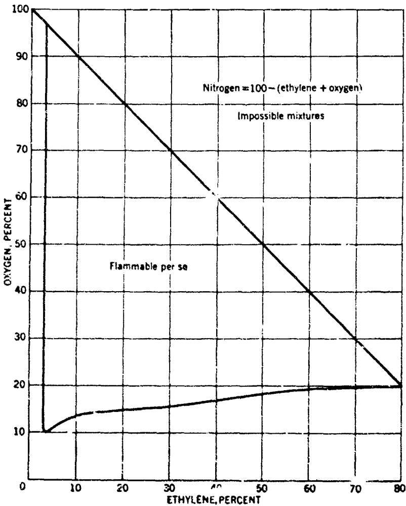
FIGURE 39. Flammability of Ethylene-Oxygen-Nitrogen Mixtures.
