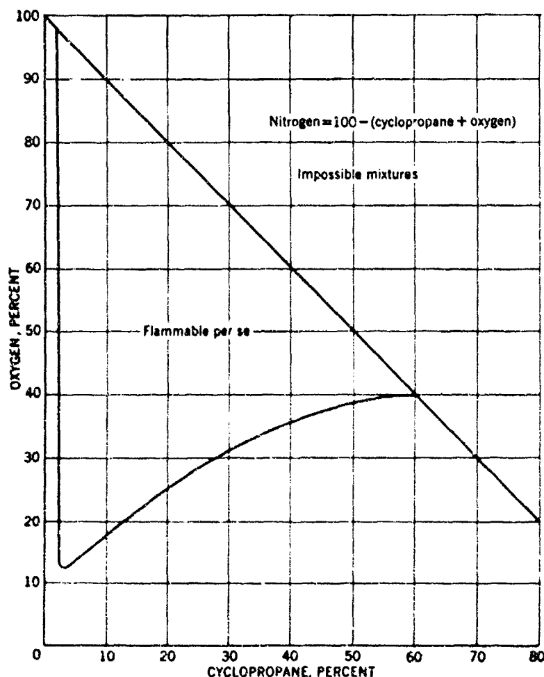
FIGURE 44.—Flammability of Cyclopropane-Oxygen-Nitrogen Mixtures.
