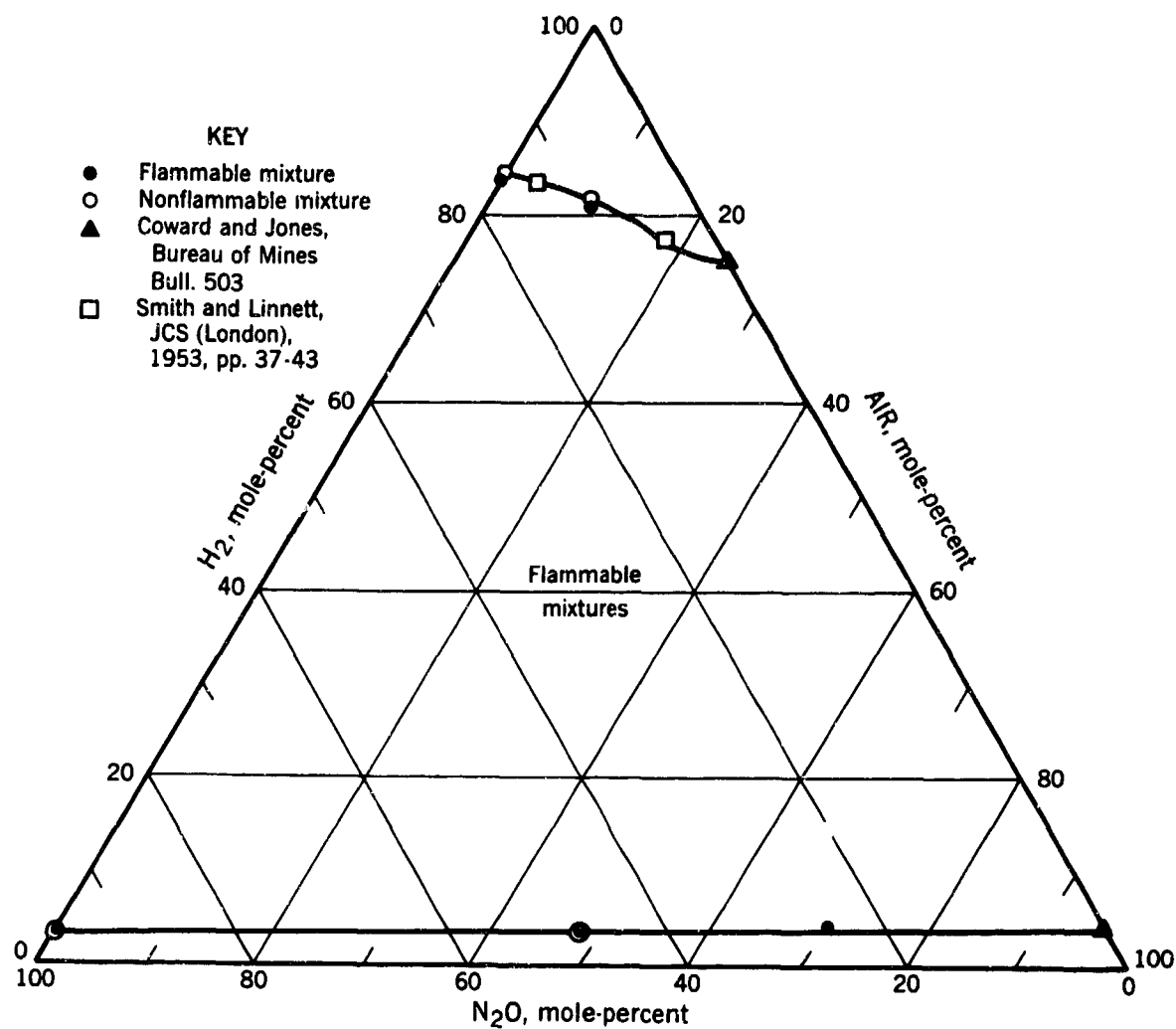
FIGURE 113.—Limits of Flammability of H 2 -N 2 O-Air at Approximately 28° C and 1 Atmosphere.
