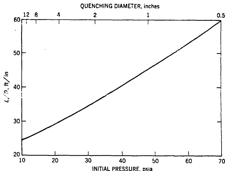
FIGURE 66.—Maximum L/D ratio Required for Transition of a Deflagration to a Detonation in Acetylene Vapor at 60^\circ F and from 10 to 70 Psia.
