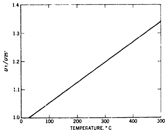
FIGURE 24.—Effect of Temperature on U/U_{25^\circ} Ratio of Paraffin Hydrocarbons in Air at Atmospheric Pressure in the Absence of Cool Flames.
