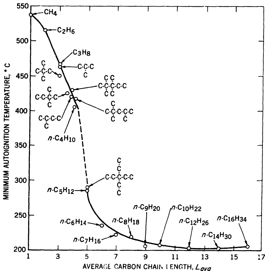
FIGURE 43.—Minimum Autoignition Temperatures of Paraffin Hydrocarbons in Air as a Function of Average Carbon Chain Length.
