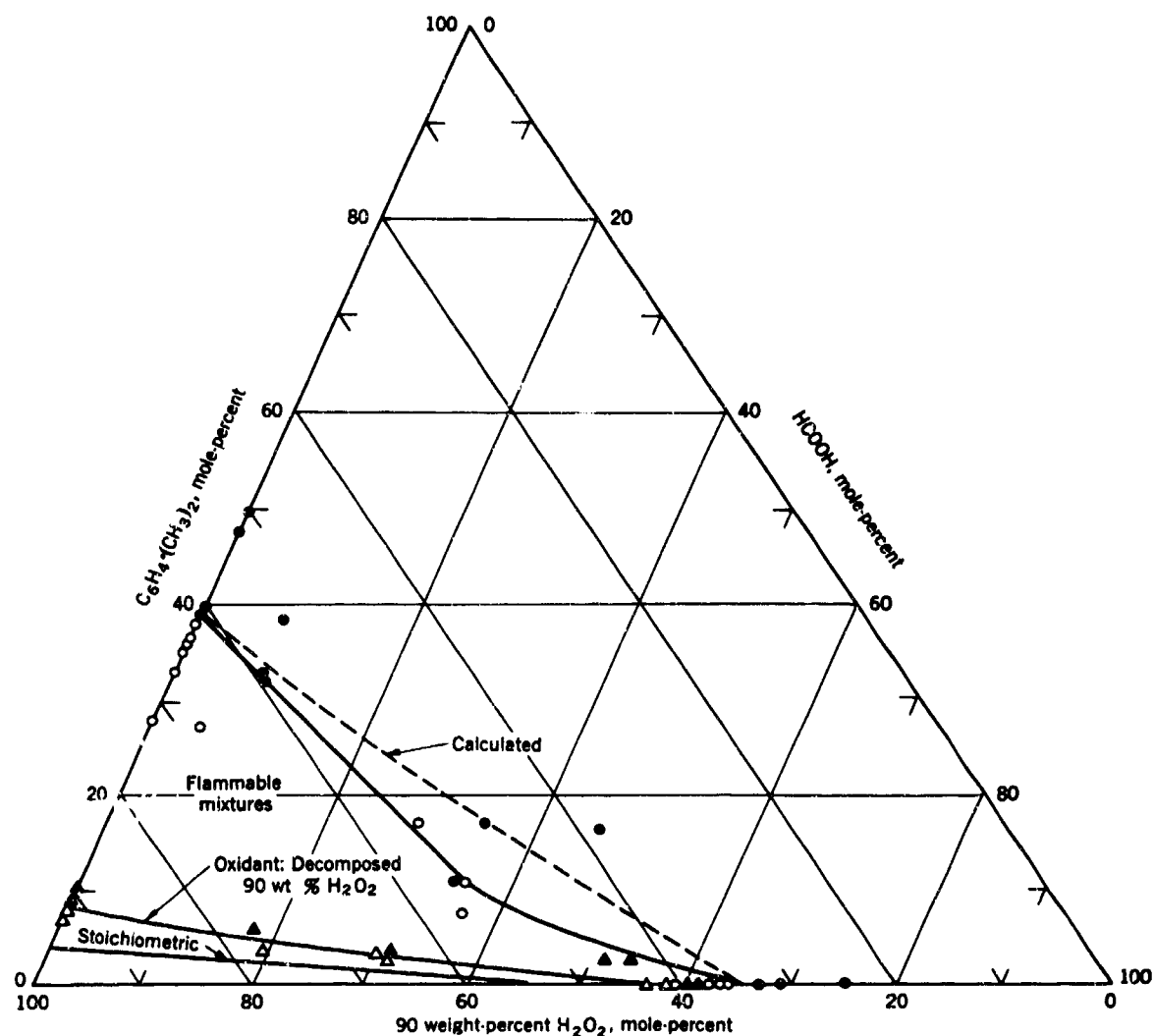
FIGURE 70.—Limits of Flammability of 90-Weight-Percent \text{H}_2\text{O}_2 - \text{C}_6\text{H}_{12}-(\text{CH}_3)_7\text{HCOOH} at 154^\circ\text{C} and 1 Atmosphere Pressure.
