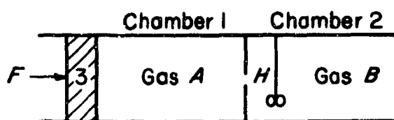
Figure 5.—Simplified mixer.
