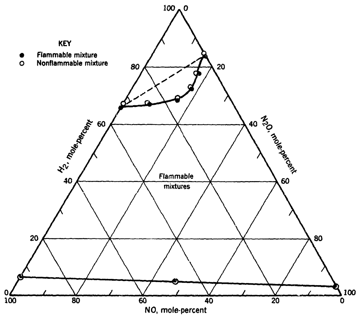
FIGURE 112.—Limits of Flammability of \text{H}_2 - \text{NO} - \text{N}_2\text{O} at Approximately 28° C and 1 Atmosphere.
