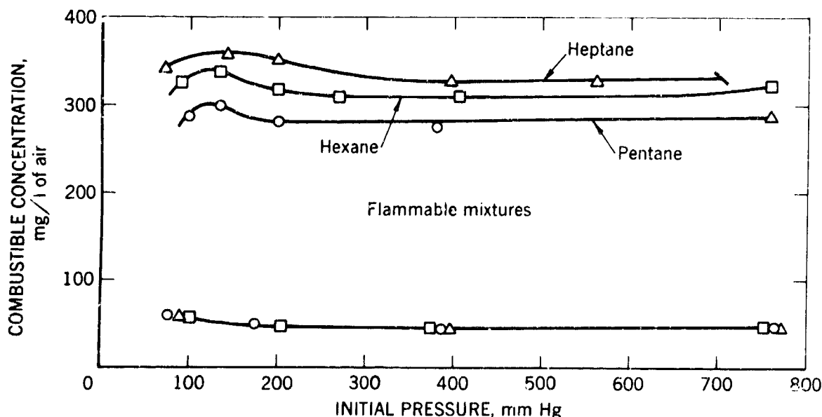
FIGURE 25.—Effect of Pressure on Limits of Flammability of Pentane, Hexane, and Heptane in Air at 26^\circ\text{C} .
