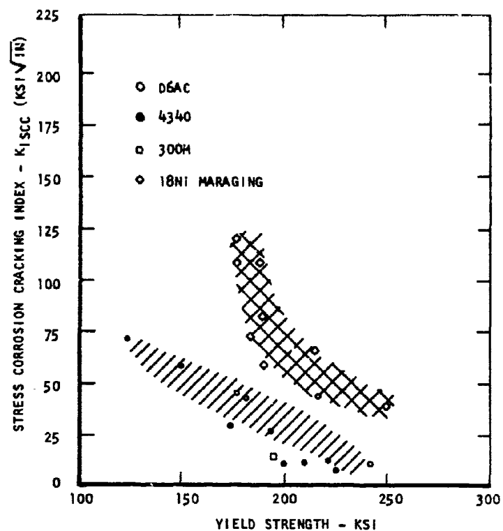
Fig.17 Variation of K_{Isc} with yield strength for a variety of high strength steels (Ref.9)
