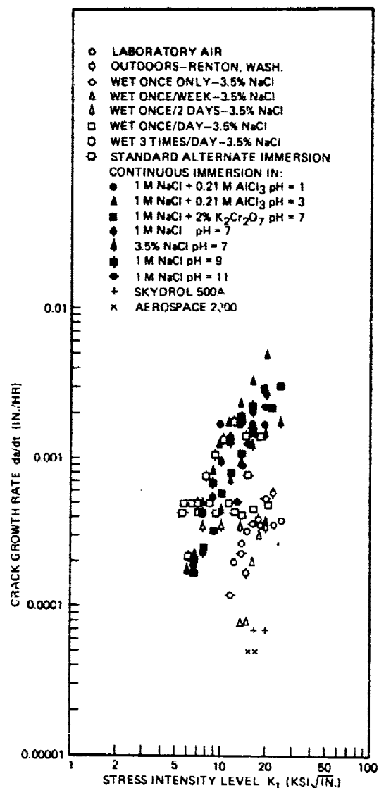
Figure 6. Evaluation of Environments Using the Double Cantilever Beam Specimen for 7075-T651 Aluminum Alloy (6)
