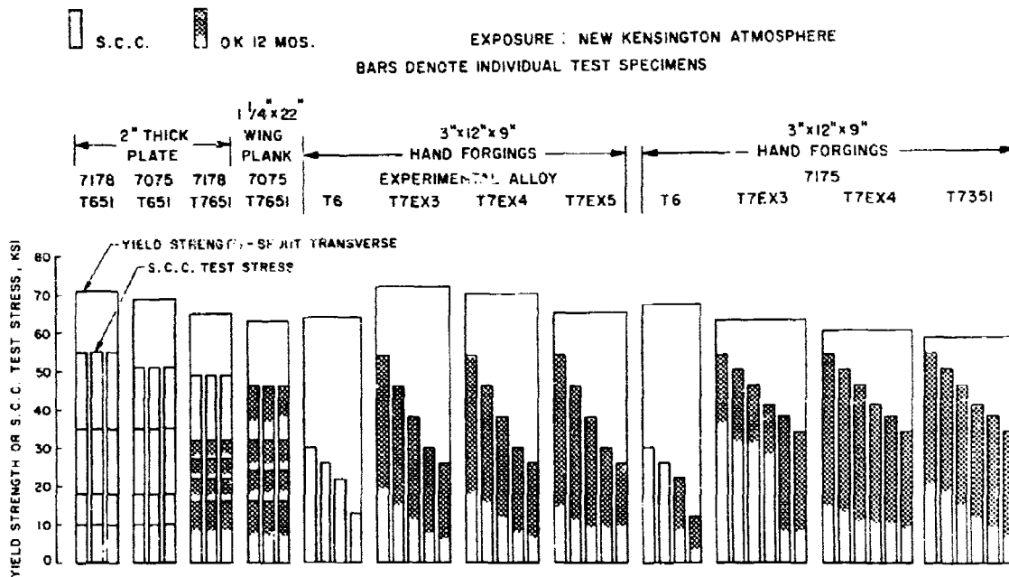
Fig. 26 This bar chart illustrates preliminary stress-corrosion cracking results (one year exposure in an industrial atmosphere) of recent alloy and temper developments in the TXXX alloys
