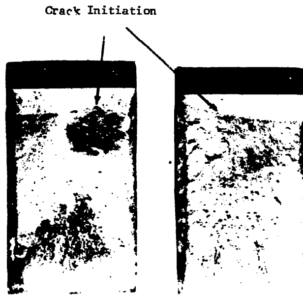
Fig. 6 Examples of irregular fracture surfaces of HP 9-4-45 steel, precracked bend specimens
