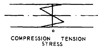
Fig. 12 Stress distribution resulting from the bending of a beam
