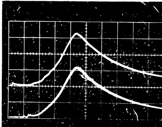
Figure 33 - VENTED BOMB RECORDS FOR TEST NO. 6
