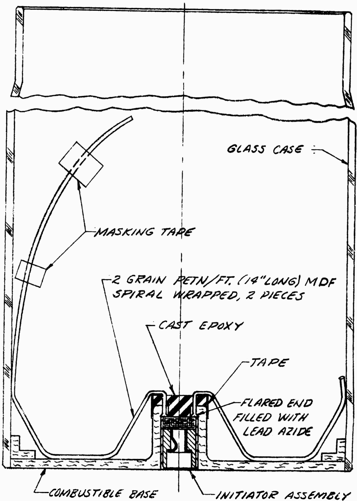
FIGURE 20 MDF INSTALLATION INTO PROTOTYPE GLASS CASE
