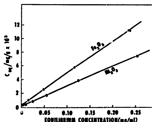
Figure 5. Langmuir plots for the sodium dinonylnaphthalenesulfonate isotherms on nickel and iron oxide powders.
