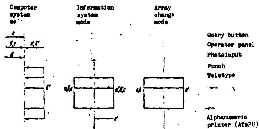
Fig. 2. Operator-machine exchange diagram of the UVS "Dnepr-2."
