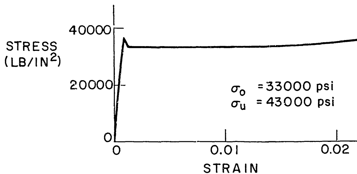
(a) MILD STEEL
