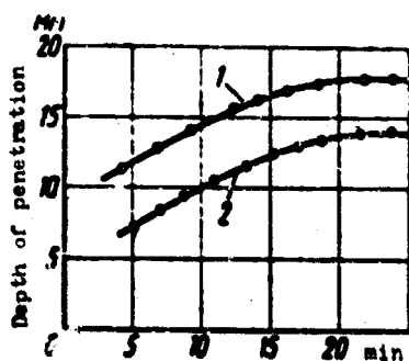
Fig. 14. Depth of penetration of glues EPTs and EORTs into the lap cavity of riveted transparent samples (with organic glass): 1 - glue EORTs; 2 - glue EPTs.
