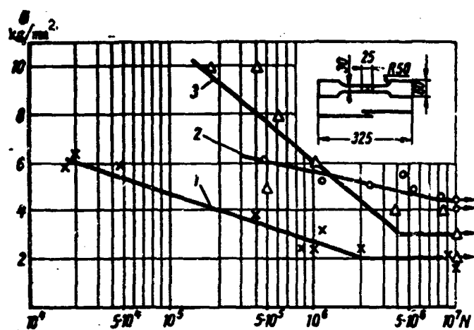
Fig. 28. Fatigue strength of single-row overlap connections of alloy D16T (1.5 + 1.5 mm): 1 - welded; 2 - glue-welded (glue VK 1SM); 3 - the same (glue KLN-1). Glue introduced after welding.
