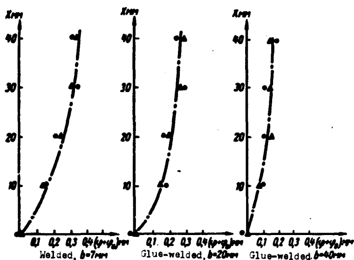
Fig. 24. Change of form of elastic line of loaded parts depending on width of weld: \Delta — measurement by optical method; \bullet — measurement by indicator deflectometer.
