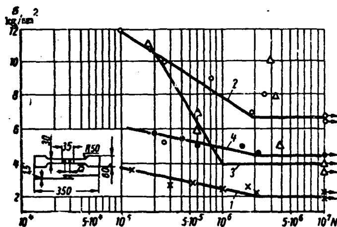
Fig. 29. Fatigue strength of two-row overlapped connections of alloy D16T (1.5 + 1.5 mm): 1 - welded; 2 - glue-welded (glue VK 1MS); 3 - the same (glue KLN 1); 4 - the same (glue FL 4S). Glue introduced after welding.
