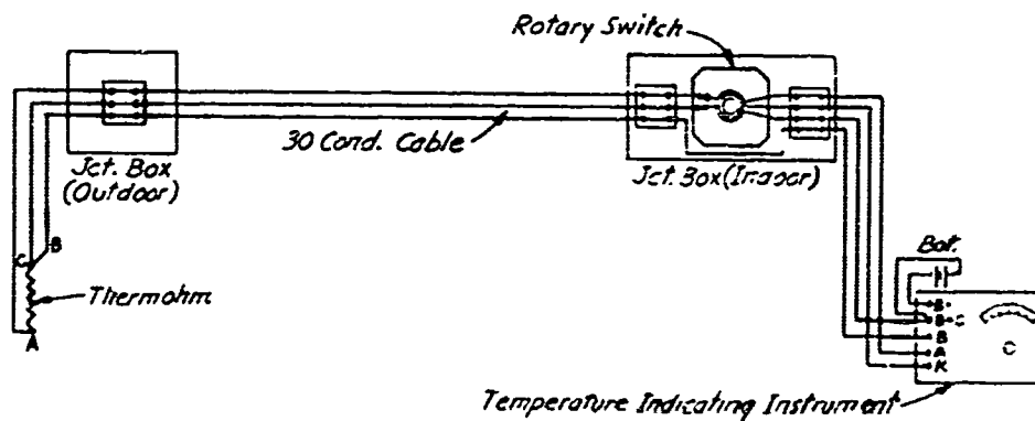
TYPICAL WIRING DIAGRAM SHOWING CIRCUIT FOR ONE THERMOHM
