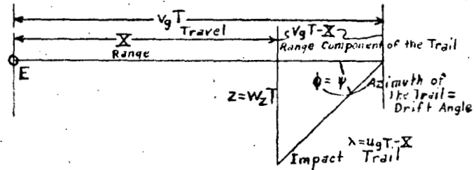
Standard Bombing Table Conditions
