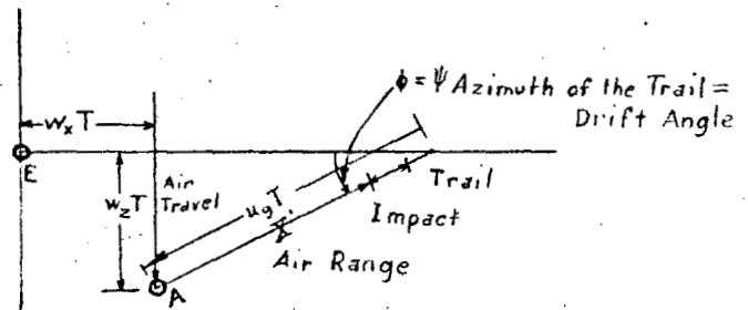
Standard Bombing Table Conditions
