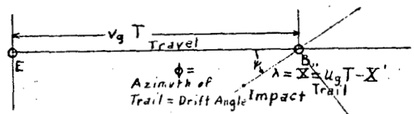
Plan Showing Elements of the Trajectory for Air Reference Frame
