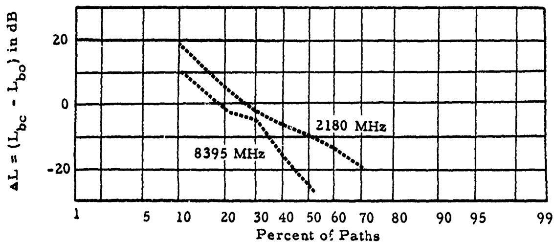
Figure 39. Cumulative distributions of basic transmission loss, observed and predicted, and of \Delta L , Virginia, f=2180 and 8395 MHz.
