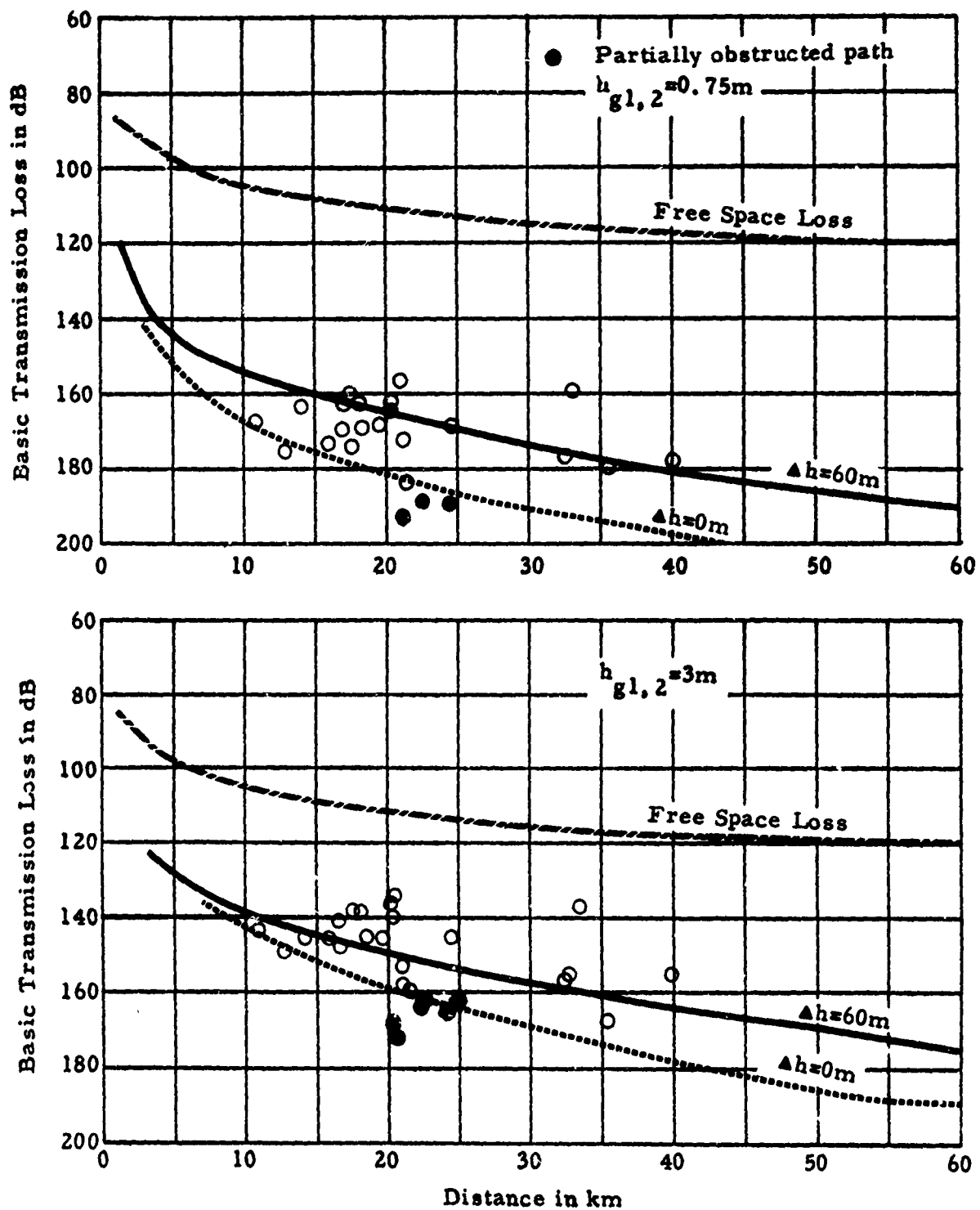
Figure 18. Basic transmission loss, measured and predicted, lava flows, Idaho, median \Delta h = 60\text{m} , f = 416\text{MHz} .
