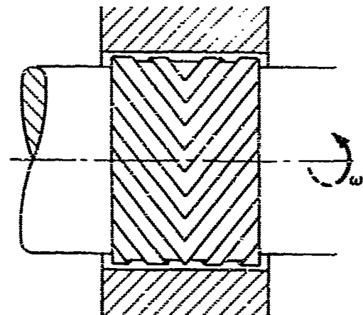
(a) Herringbone Grooved Journal Bearing
