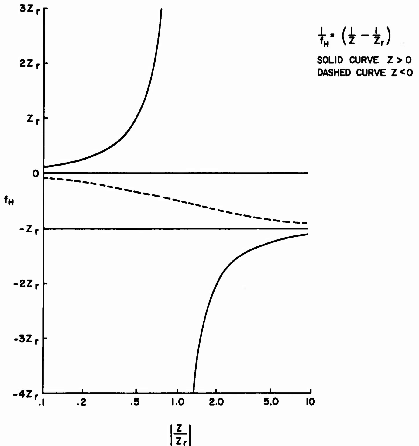
Figure 8. Variation of Focal Length with Reconstruction Radius of Curvature (Real Image Mode).
