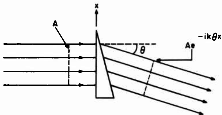
Figure 3. Transform Properties of a Prism.
