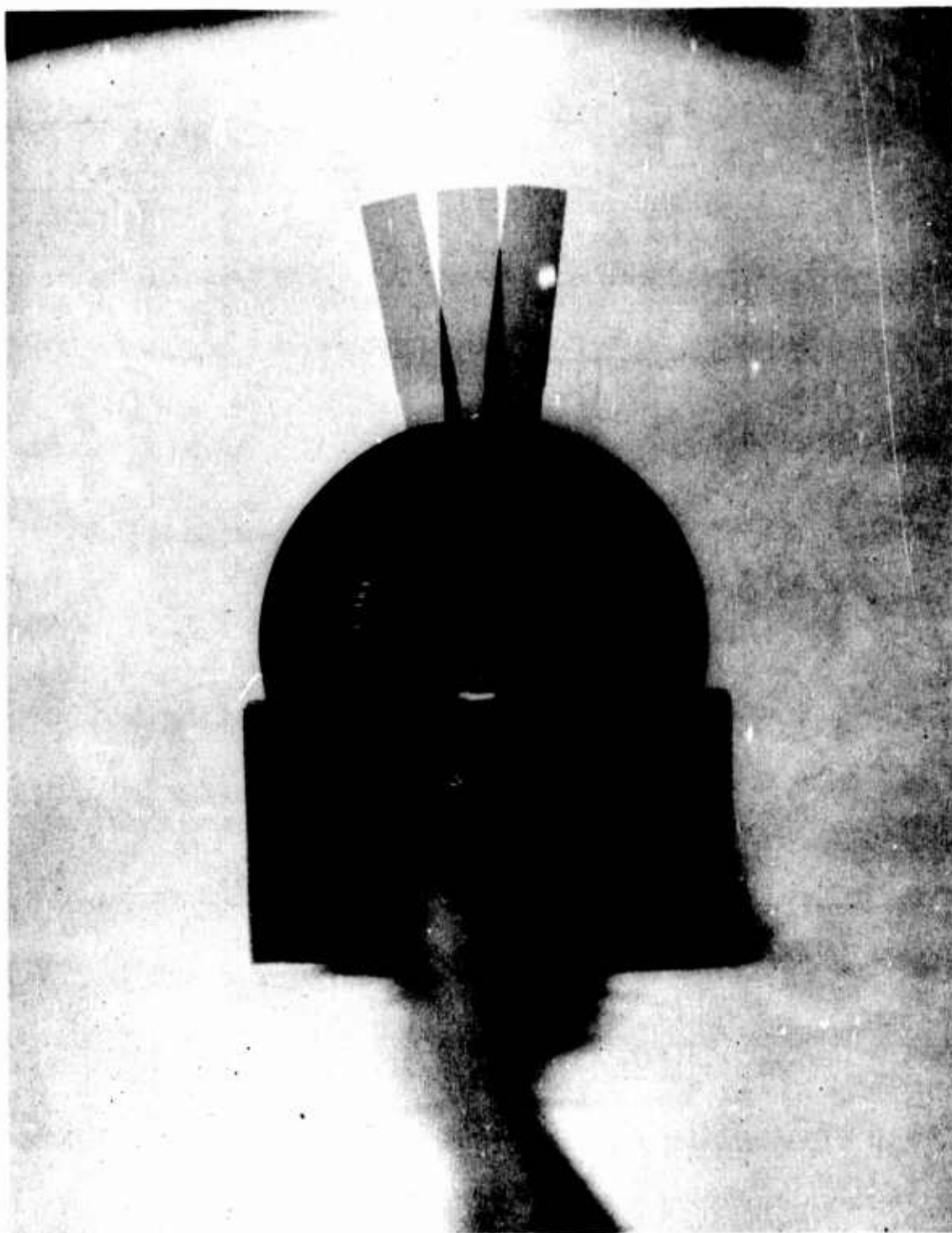
Figure 34. Rotation of Camera Assembly Within its Housing Provides Roll Simulation.
