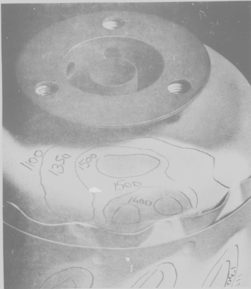
SHELLDYNE-H MODIFIED COMBUSTOR ISOTHERMS
