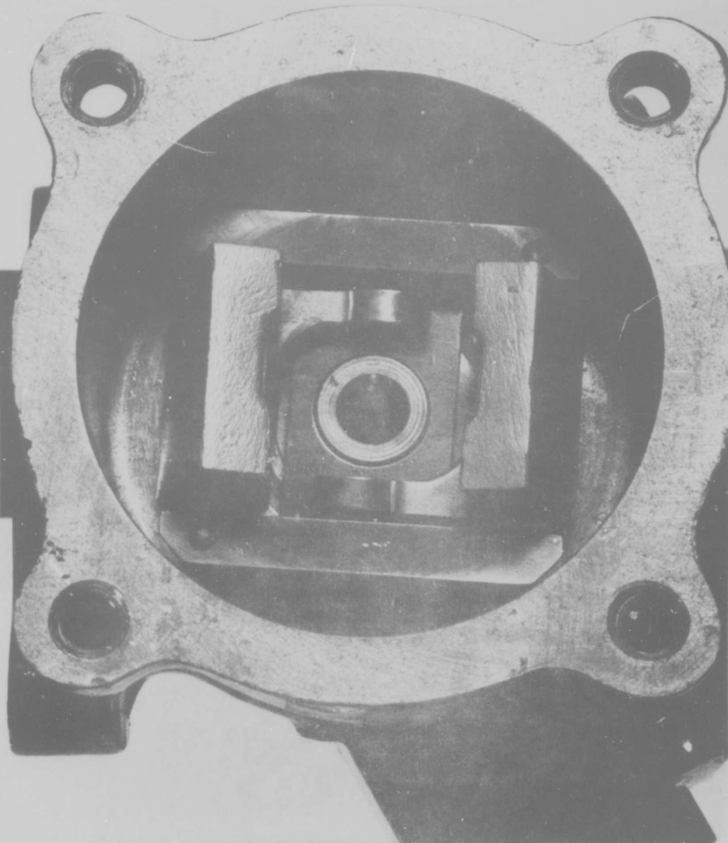
GOVERNOR FLYWEIGHT ASSEMBLY WITH SPOOL VALVE REMOVED
