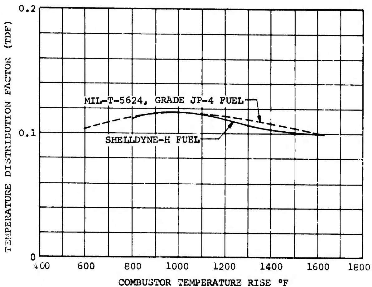
TEMPERATURE DISTRIBUTION FACTOR COMPARISON
