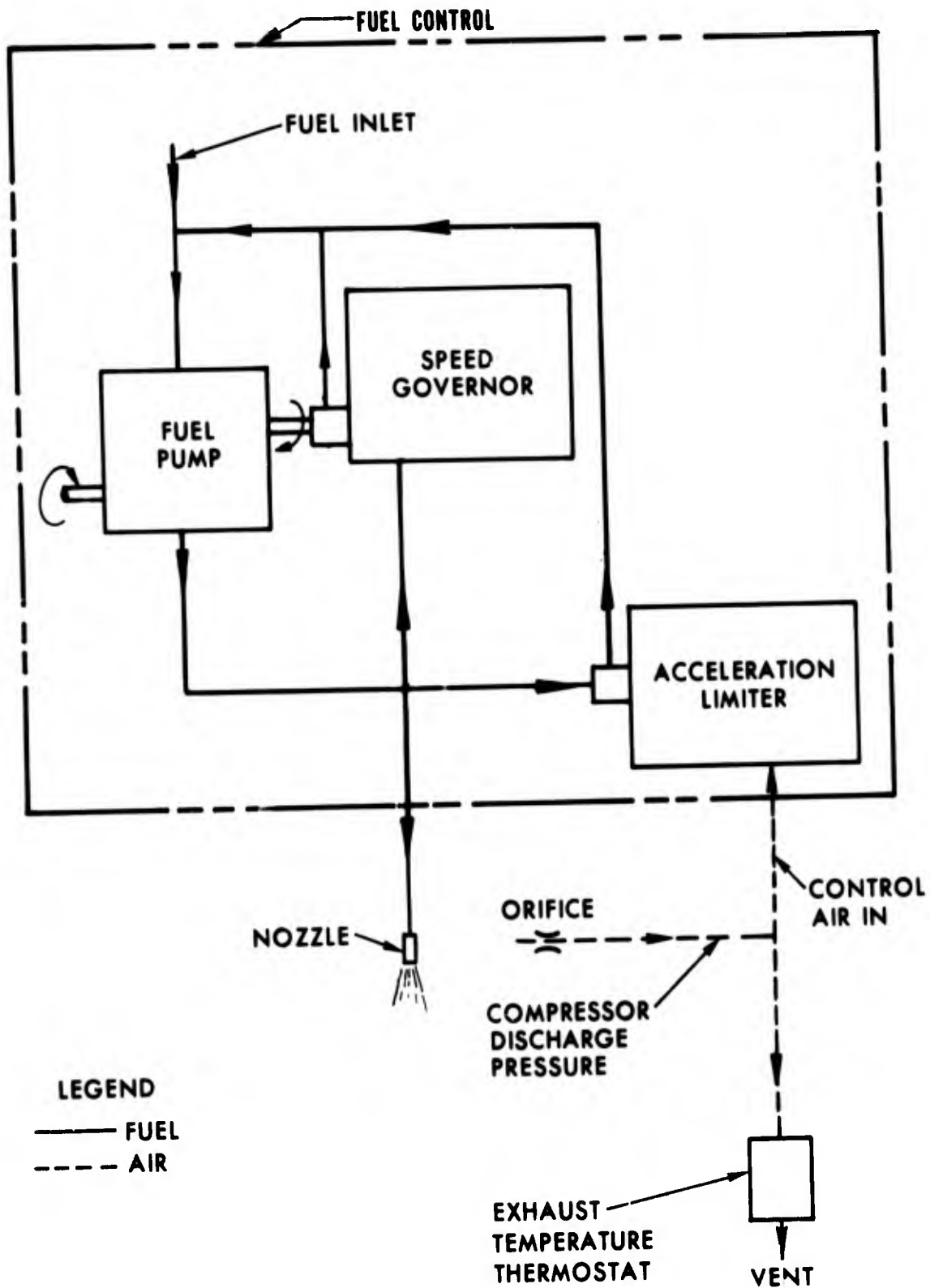
SCHEMATIC OF ACCELERATION LIMITER RELATIONSHIP FIGURE 6
