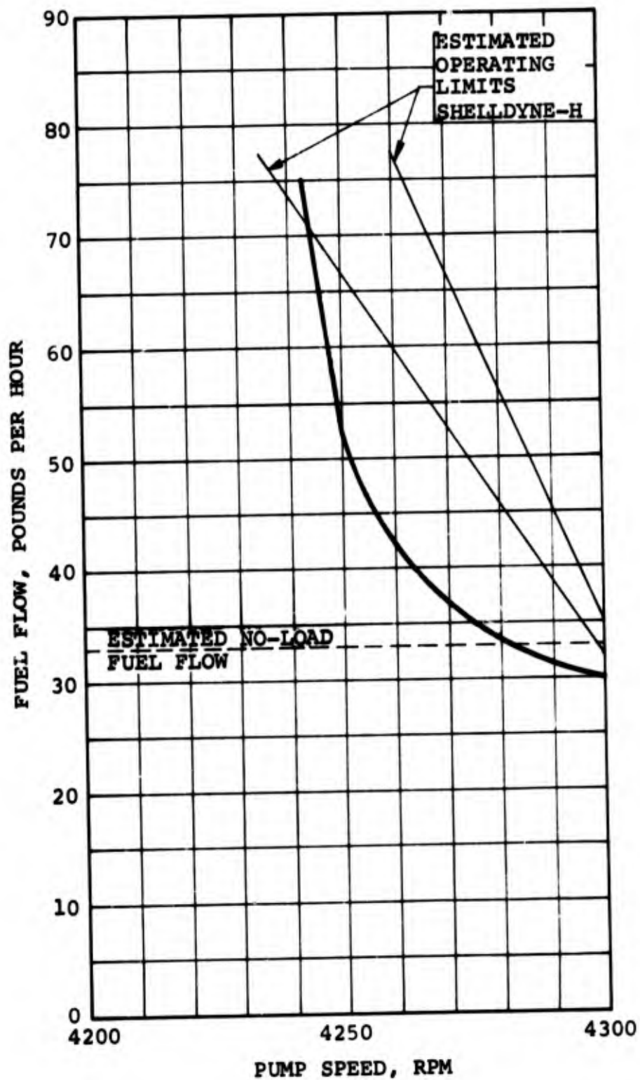
FUEL CONTROL UNIT GOVERNOR GAIN WITH SHELLDYNE-H FUEL AT 90°F AND 30-POUND-PER-INCH GOVERNOR SPRING
