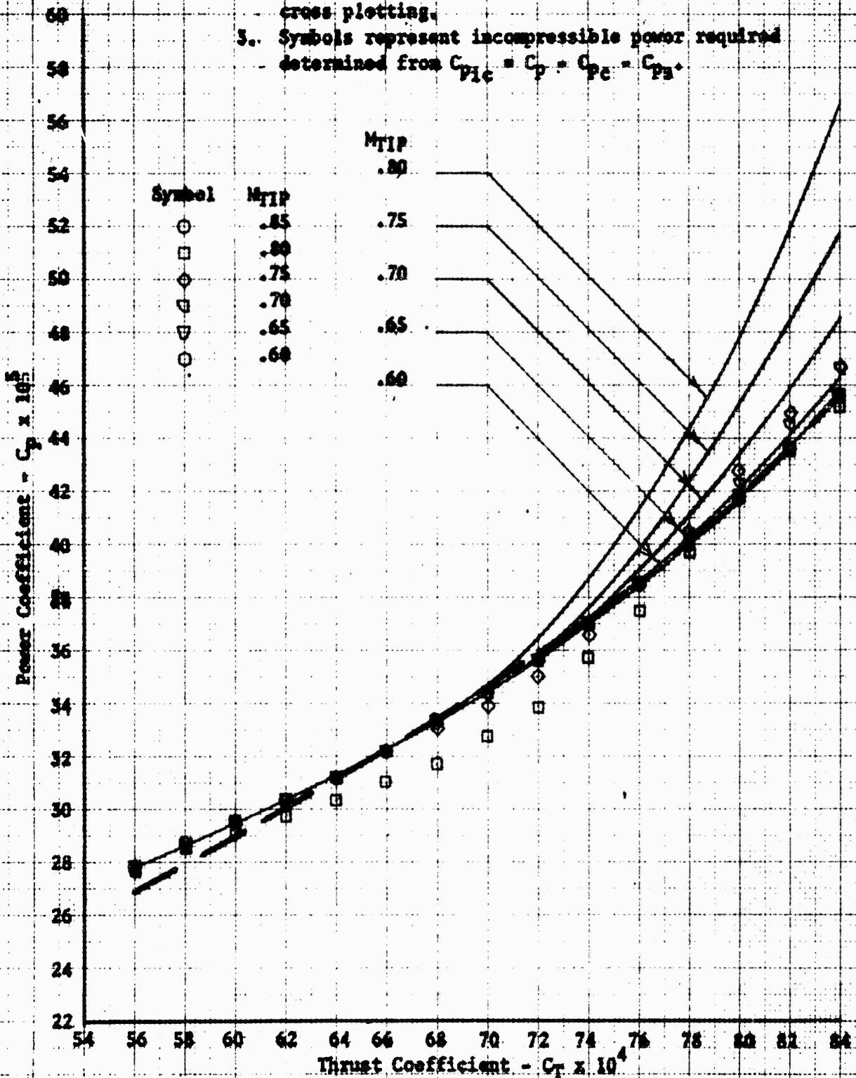
Figure 3. Nondimensional Level Flight Performance.
