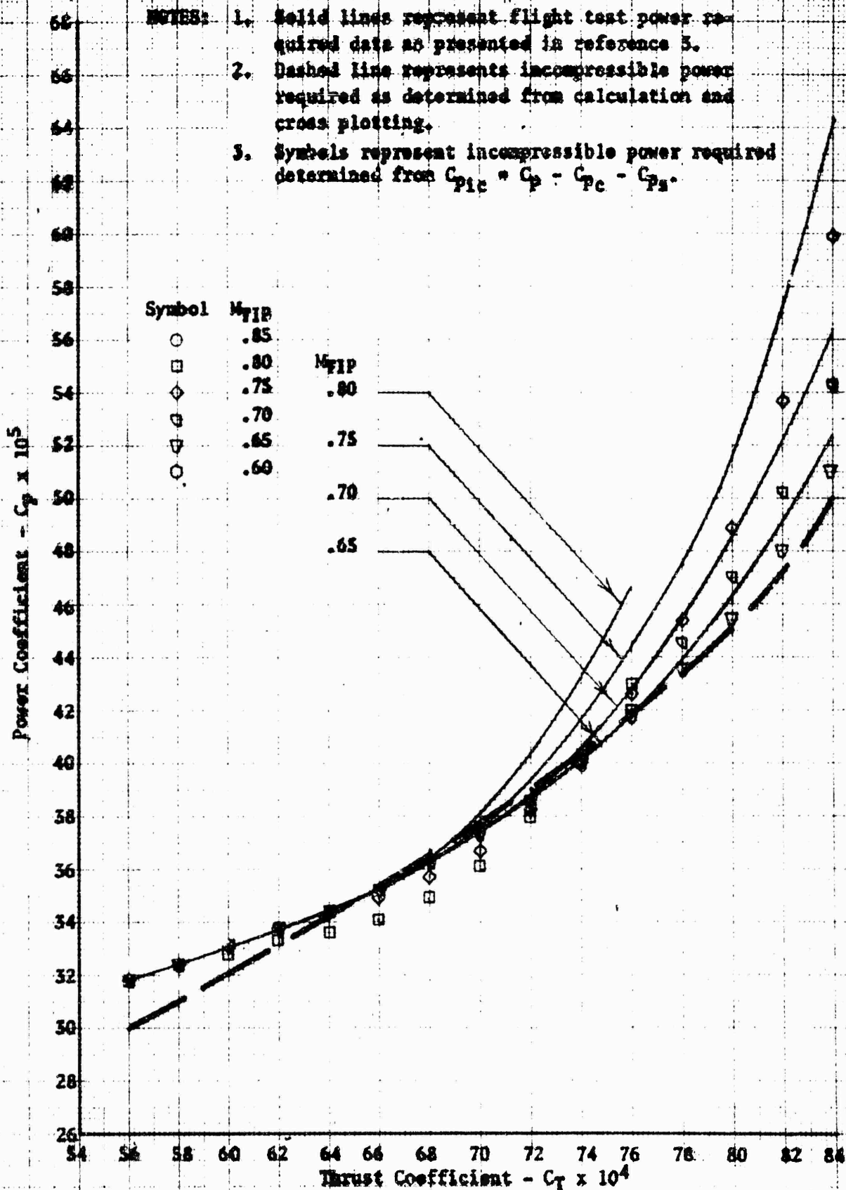
Figure 9. Nondimensional Level Flight Performance
