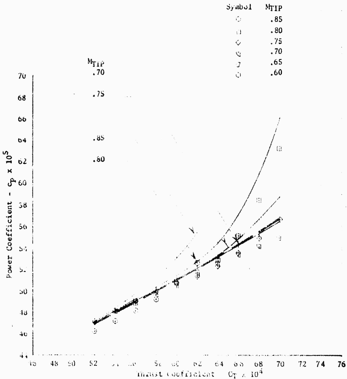
Figure 11. Semirandom level flight performance
