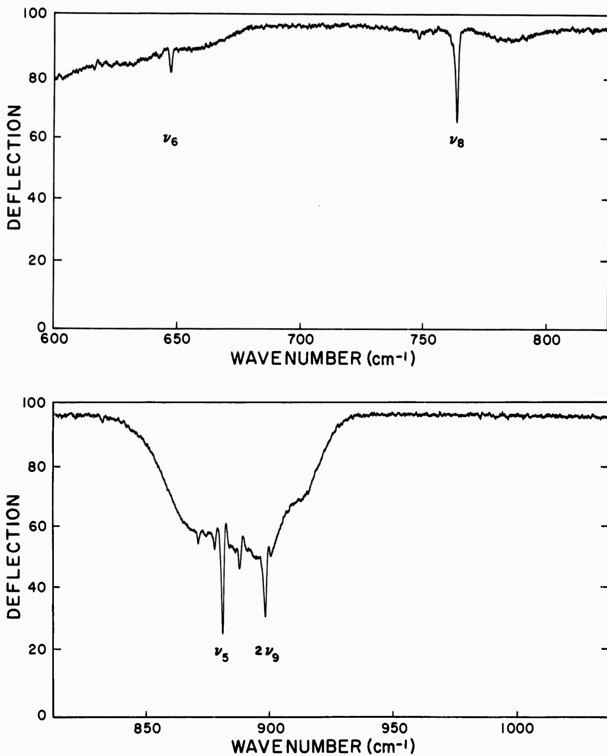
Fig. 4. Spectrum of \text{HNO}_3 vapor in the region 600\text{--}4000\text{ cm}^{-1} at \sim 0.5\text{ cm}^{-1} resolution, 4.6 mmHg pressure, at 40^\circ\text{C} in the 9.94 cm glass absorption cell.
