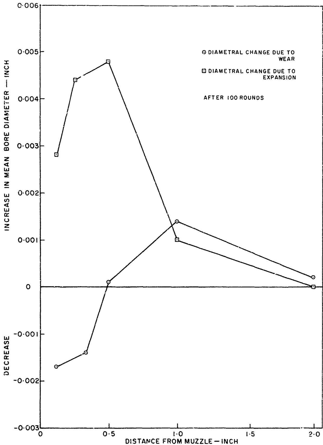
FIG.14: CHANGES IN BORE DIAMETER OWING TO WEAR AND EXPANSION, CARBONYL NICKEL SHOT
