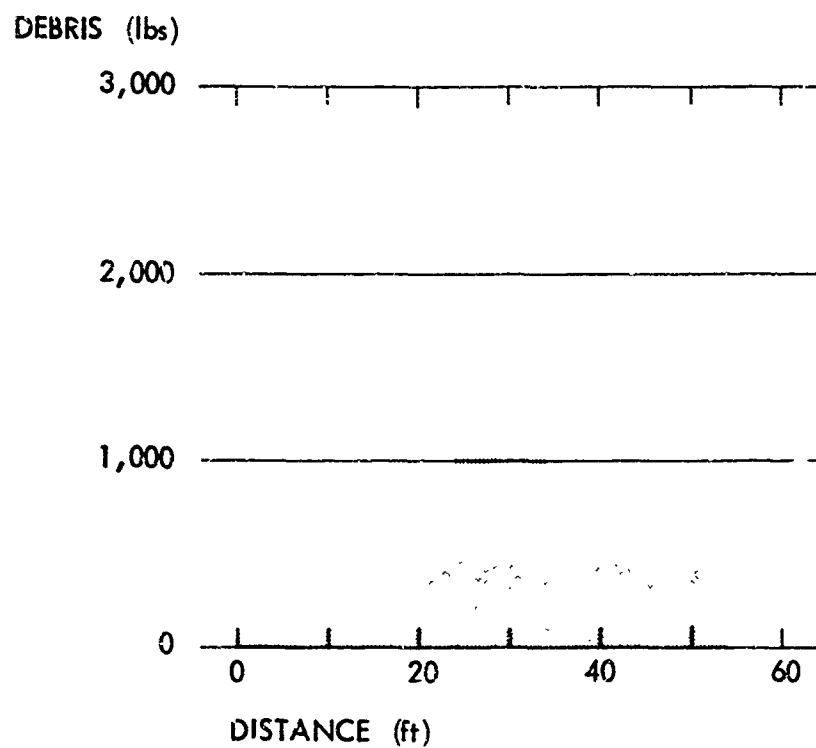
Debris Distribution, Wall Number 6
