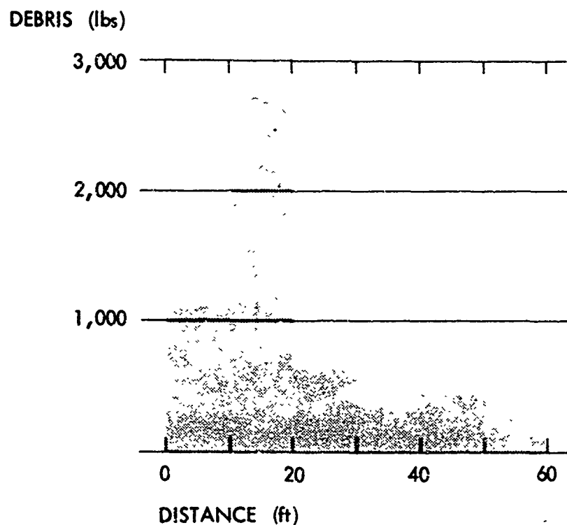
Debris Distribution, Wall Number 23
