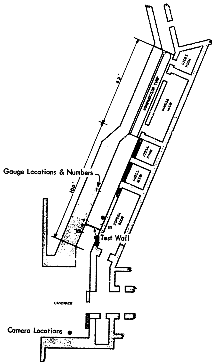
Fig. 5. Plan View of Shock Tunnel Facility
