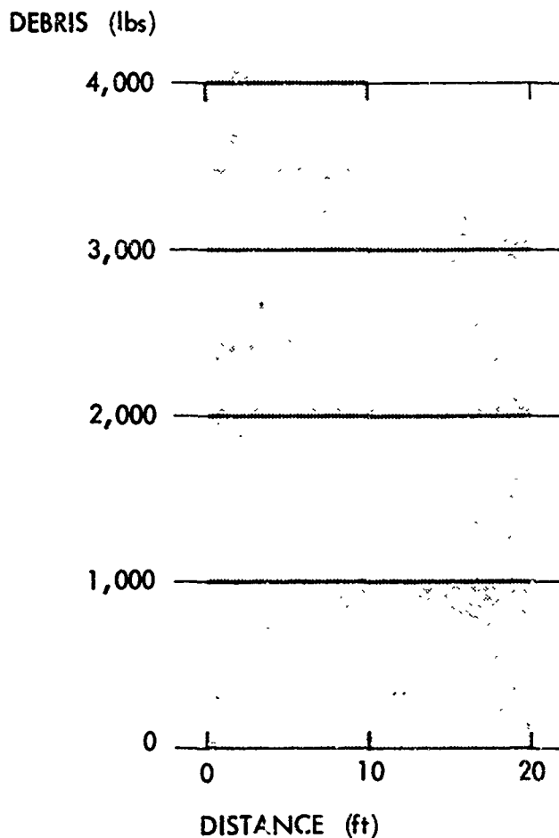
Debris Distribution, Wall Number 7
