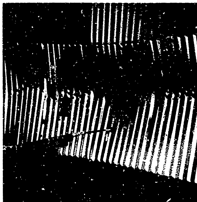
Fig. 7. Post-test View of Non-failing Wall
