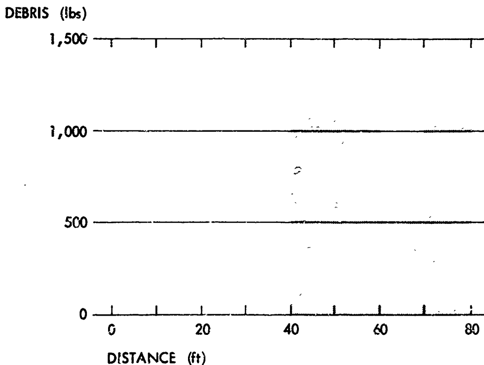
Debris Distribution, Wall Number 30
