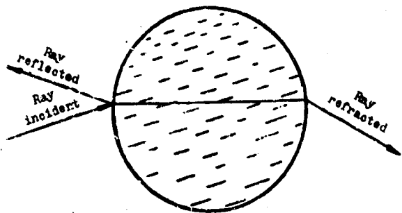
Fig. 1. Diagram of refraction and reflection of light by a droplet of fog.
