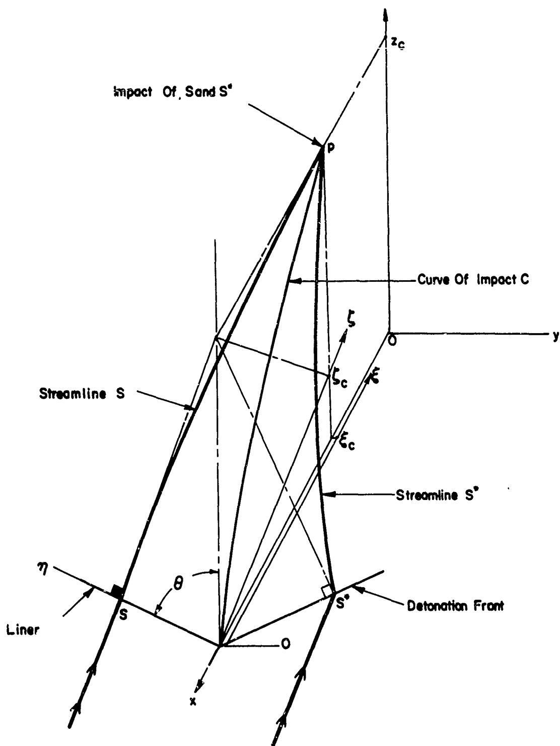
FIGURE 6. LINER FLOW AND STREAMLINE COORDINATES.
