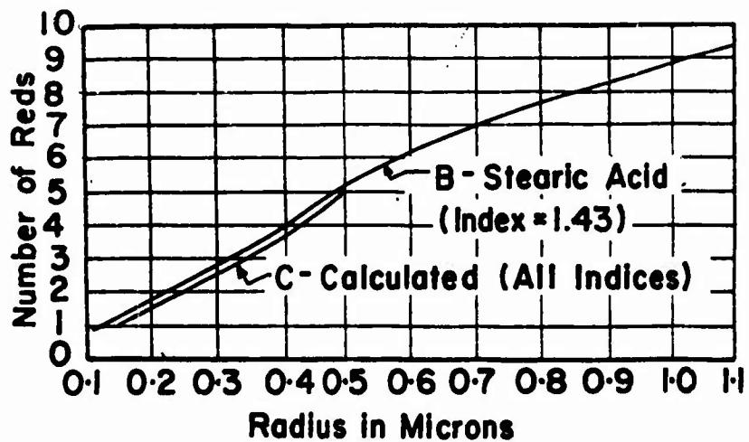
Figure 15. OBSERVED AND THEORETICAL NUMBERS OF REDS PLOTTED AGAINST PARTICLE RADIUS ( Sinclair 1950 )
